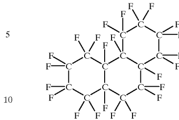
Chemical Formula 8
