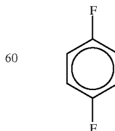
Chemical Formula 13
