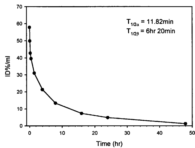
Plasma Clearance of 125 I-HSA-DX890
