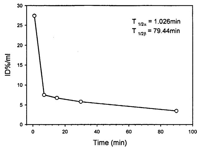
Plasma Clearance of 125 I - DX890
