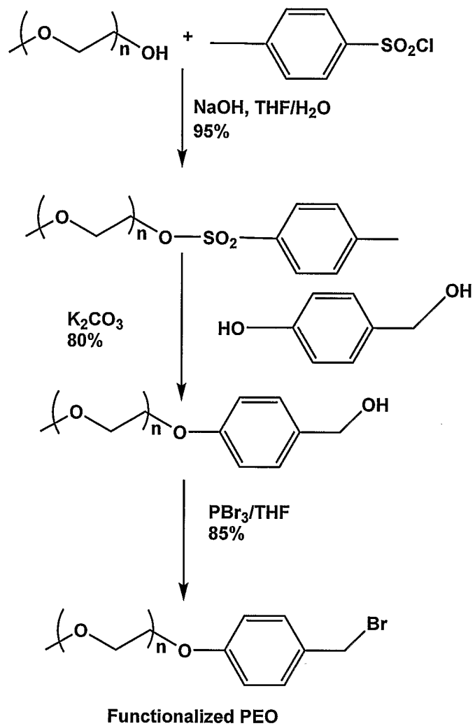
Scheme 1-Functionalizing Poly(ethylene oxide) Monomethyl Ethers
