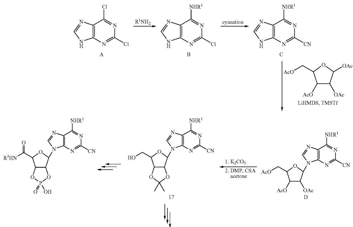
Scheme 10
