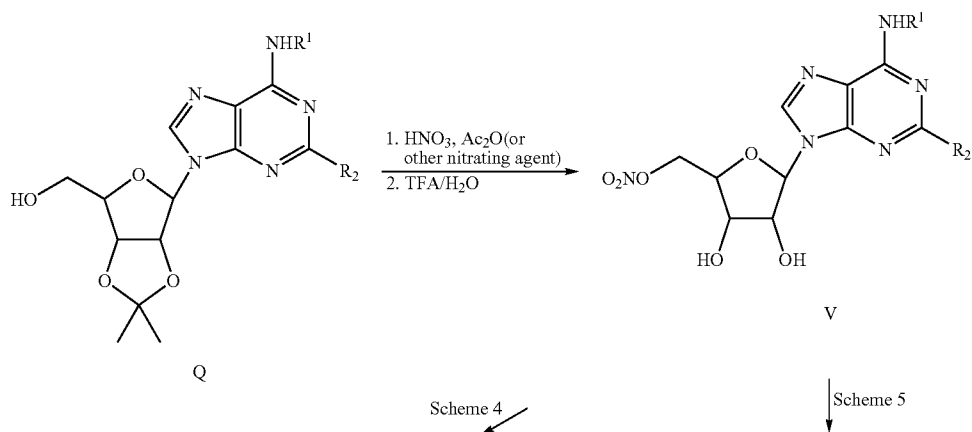
Scheme 33
