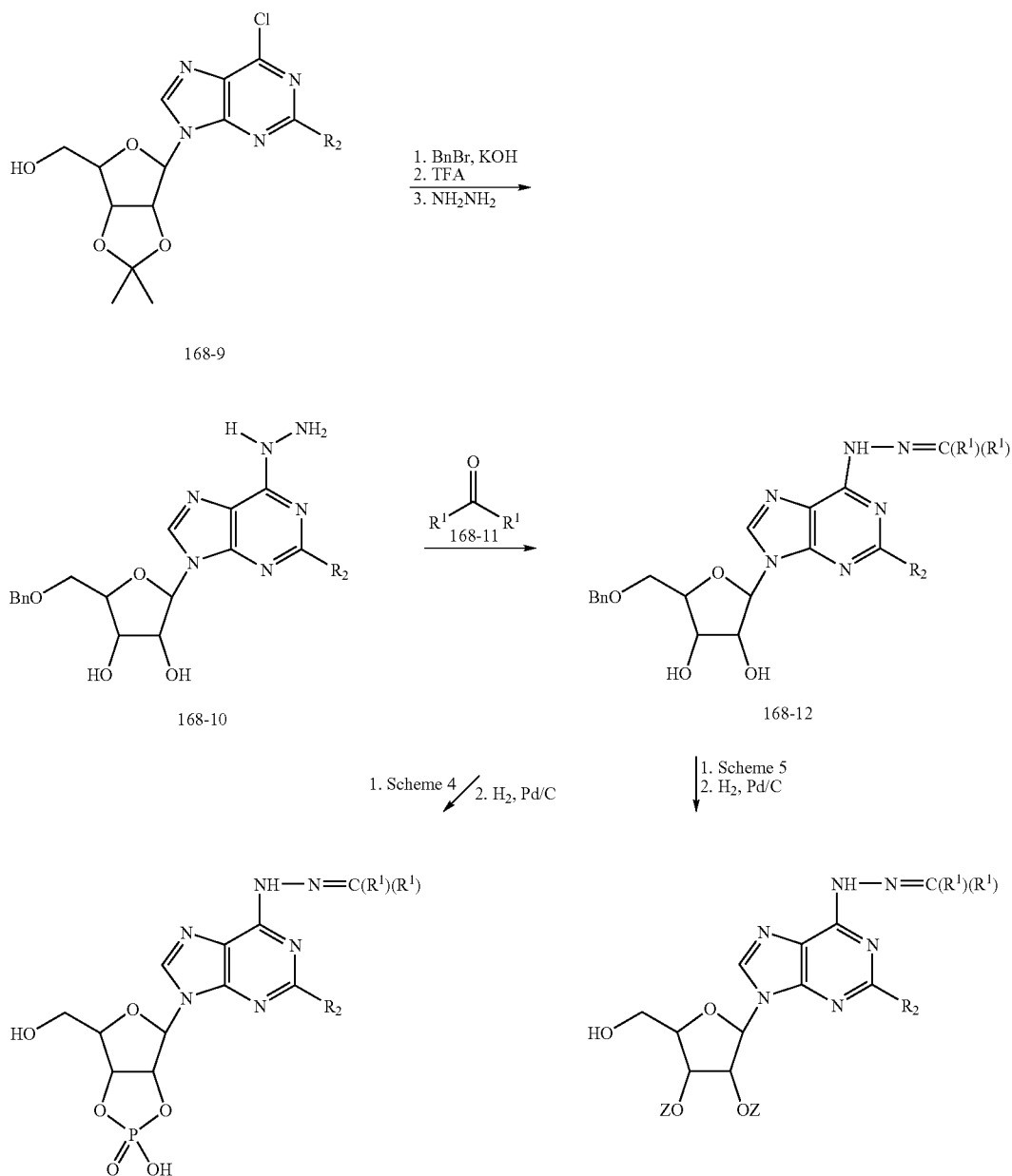
Scheme 18
