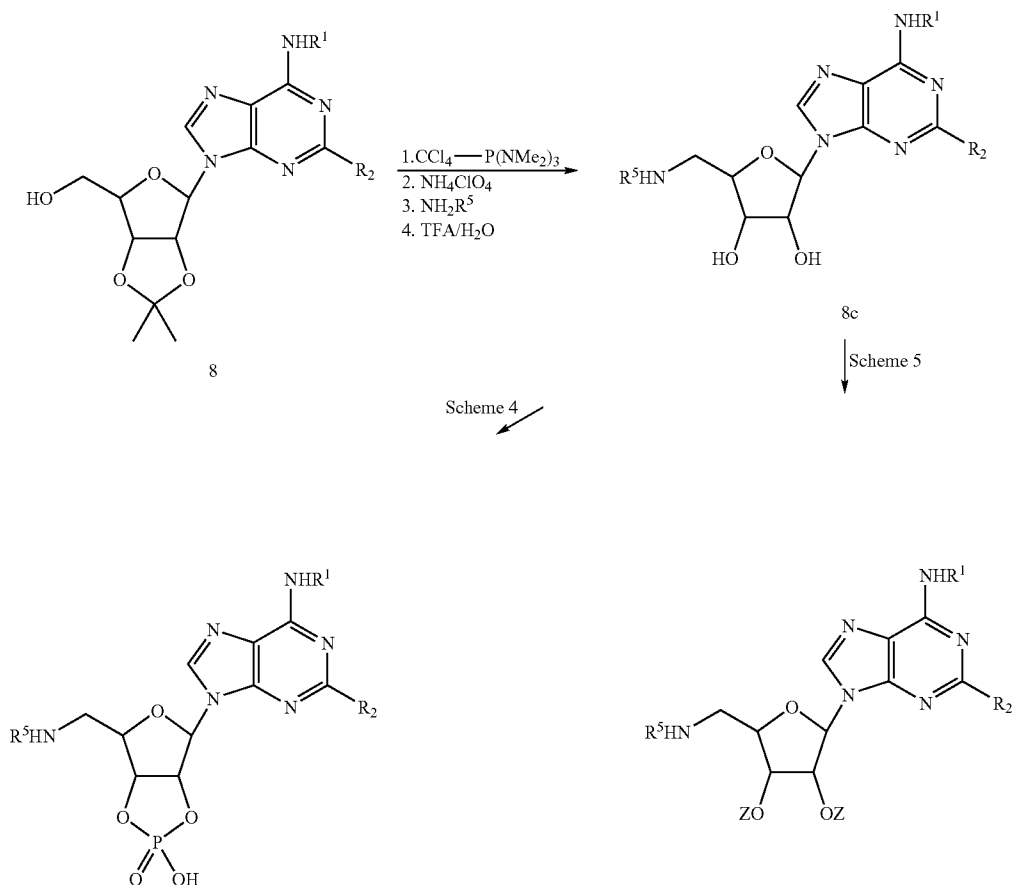
Scheme 14
