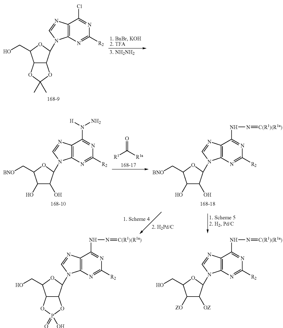
Scheme 21
