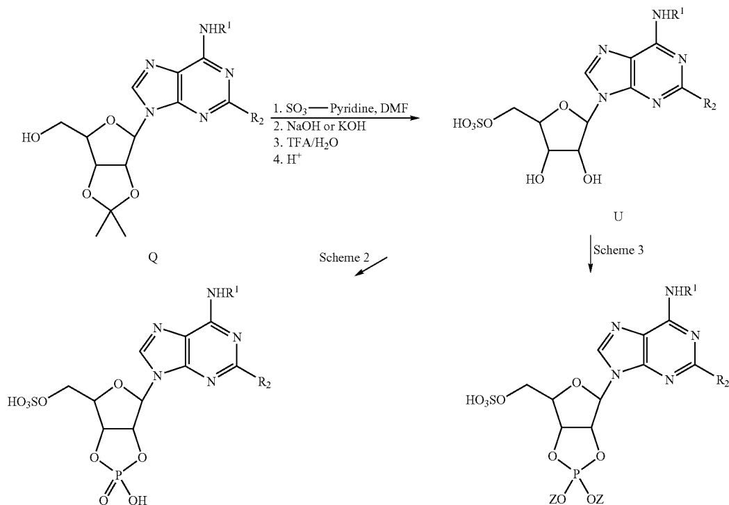
Scheme 32
