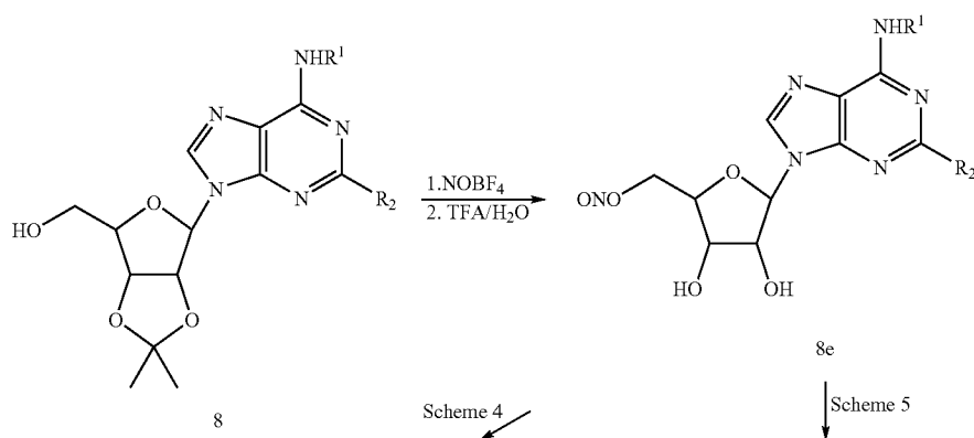
Scheme 16
