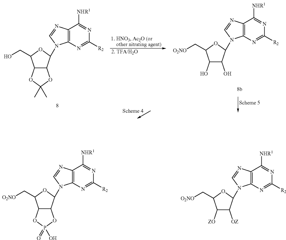
Scheme 13
