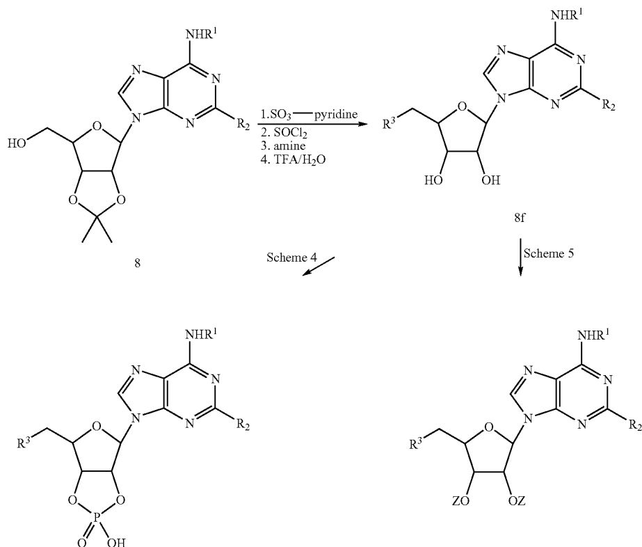
Scheme 17
