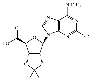
2',3'-Isopropylidene-2-cyano-N 6 -methyladenosine-5'-carboxylic acid
