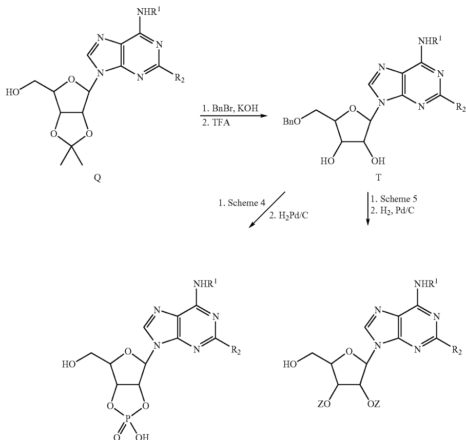
Scheme 31
