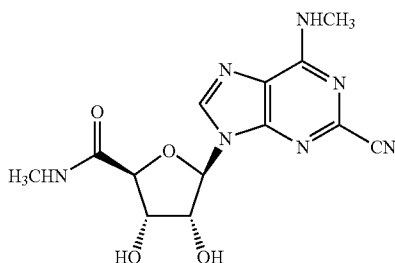
Synthesis of Compound 64a
