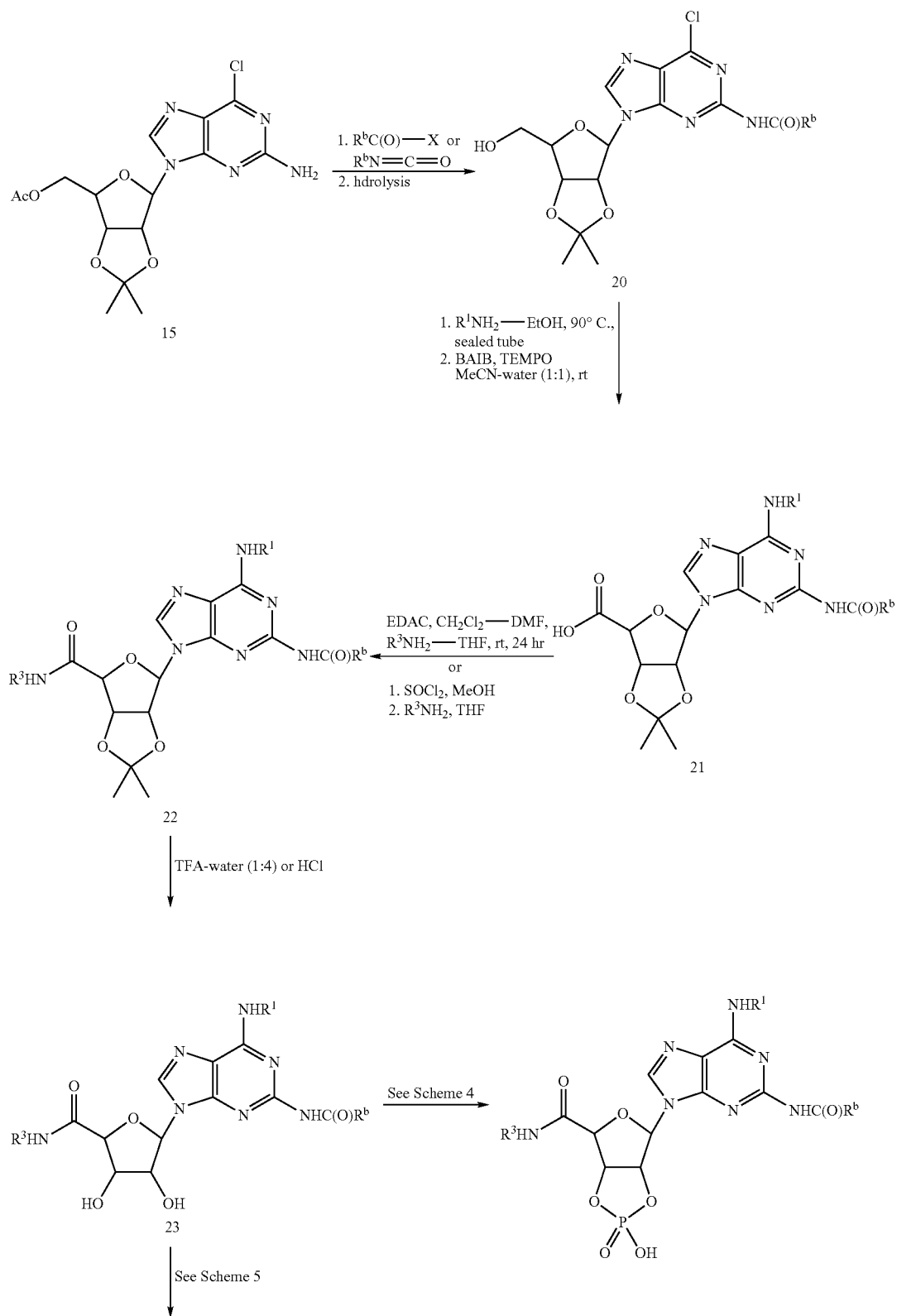
Scheme 9
