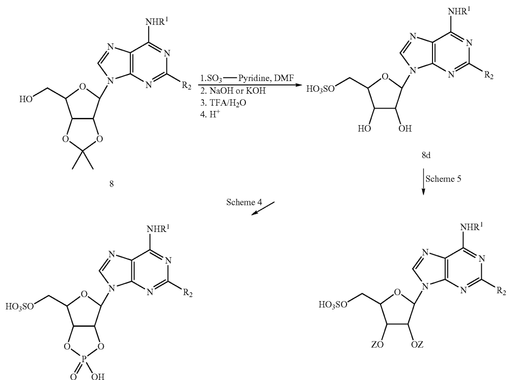
Scheme 15
