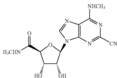
N-methyl-2-cyano-N 6 -methyladenosine-5'-N-carboxamide
