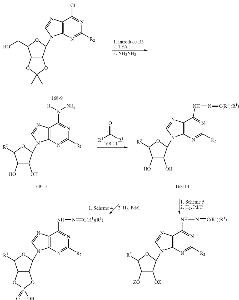
Scheme 19
