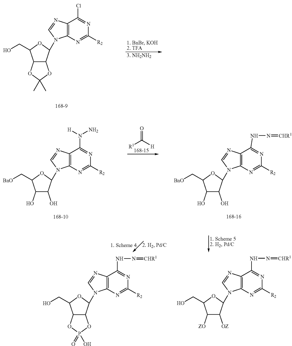
Scheme 20
