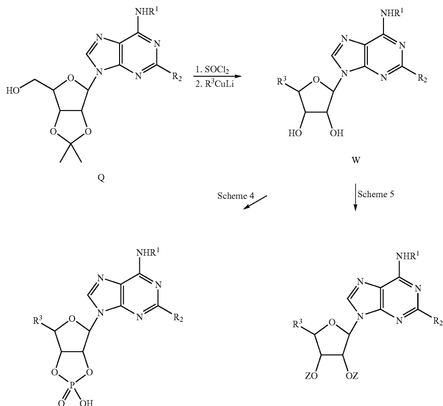
Scheme 34
