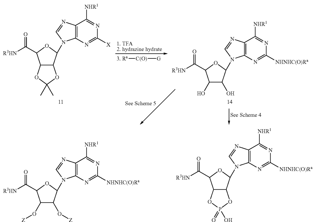
Scheme 7
