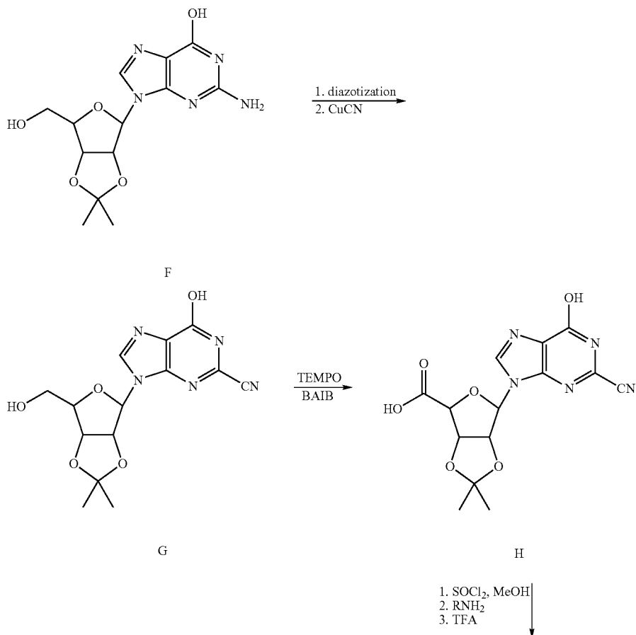
Scheme 11
