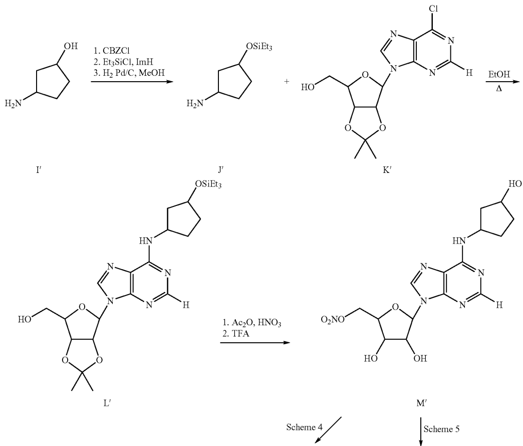
Scheme 23
