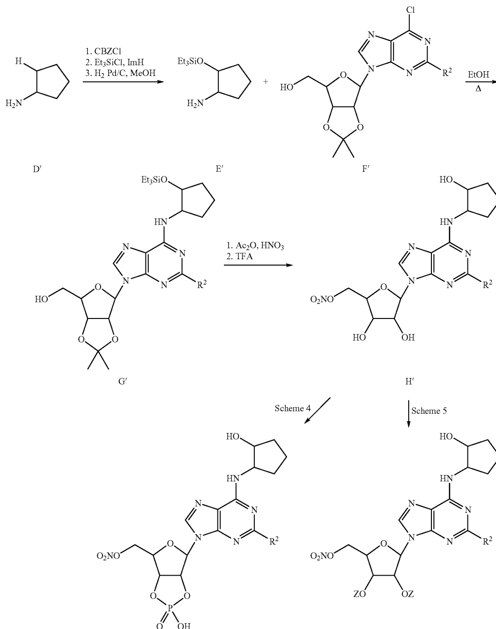
Scheme 22
