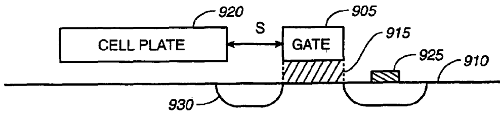
FIG. 9 (PRIOR ART)
