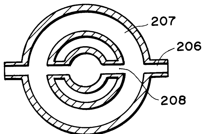
D-D' SECTION
