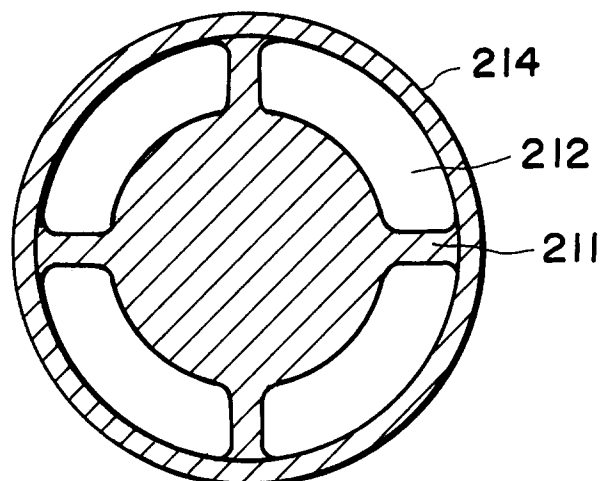
C-C' SECTION
