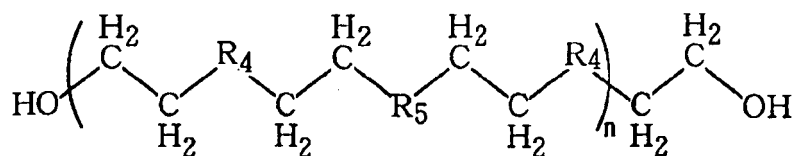
General formula (10)
