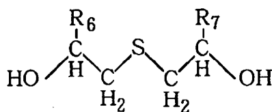
General formula (11)
