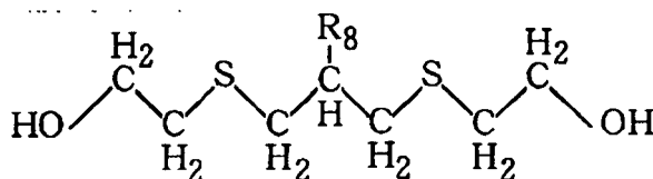
General formula (12)
