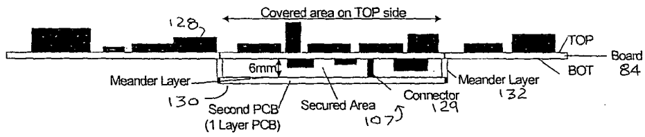
Close Up of Secure Area on Board
