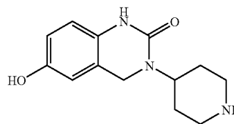
6-Hydroxy-3-piperidin-4-yl-3,4-dihydro-1H-quinazolin-2-one
