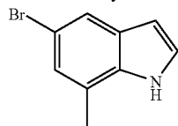
5-Bromo-7-methyl-1H-indole
