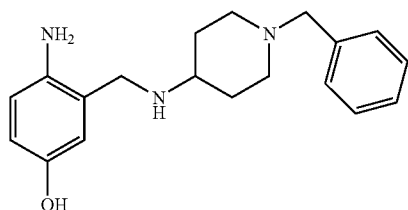
4-Amino-3-[(1-benzyl-piperidin-4-yl-amino)-methyl]-phenol
