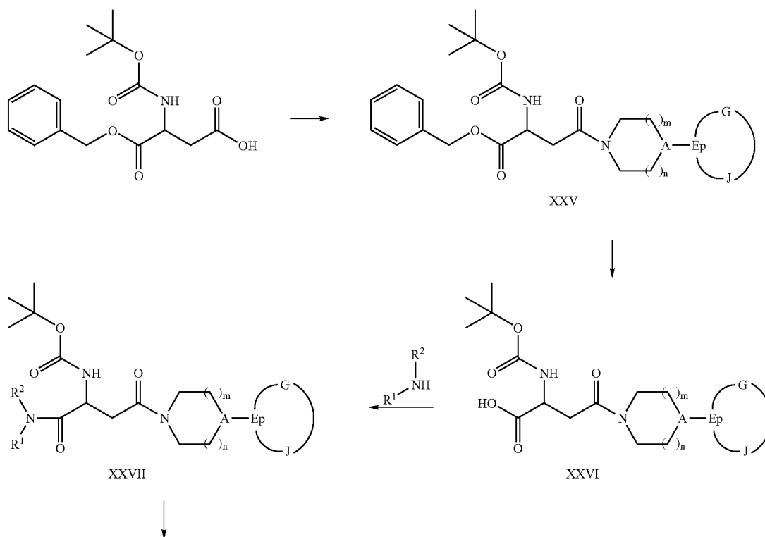
Scheme 8. Synthesis of Formula I Compounds
