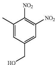
(3-Methyl-4,5-dinitrophenyl)methanol
