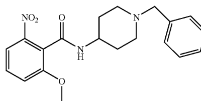
N-(1-Benzyl-piperidin-4-yl)-2-methoxy-6-nitro-benzamide
