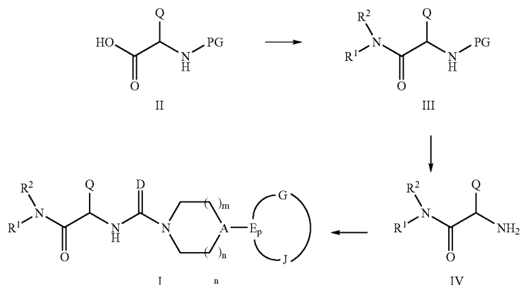
Scheme 1. Synthesis of Formula I Compounds
