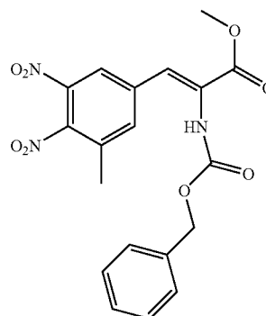
Benzyl (Z)-1-(methoxycarbonyl)-2-(3-methyl-4,5-dinitrophenyl)vinylcarbamate
