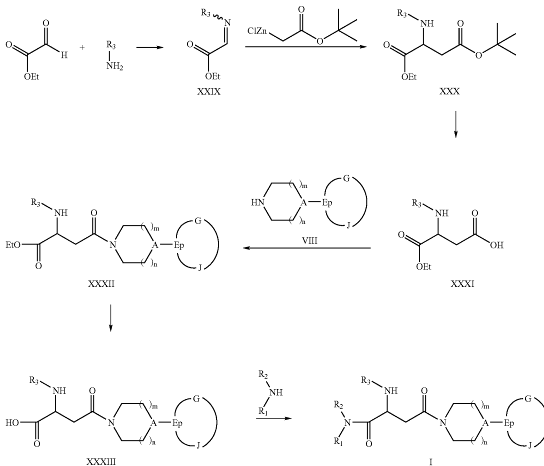
Scheme 9. Synthesis of Formula I Compounds
