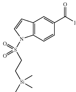
1-(2-Trimethylsilylanyl-ethanesulfonyl)-1H-indole-5-carbaldehyde
