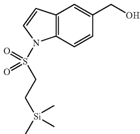
[1-(2-Trimethylsilylanyl-ethanesulfonyl)-1H-indol-5-yl]-methanol
