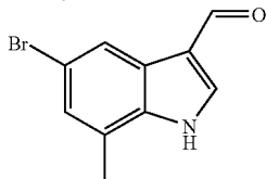
5-Bromo-7-methyl-1H-indole-3-carboxaldehyde
