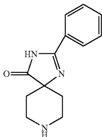
2-Phenyl-1,3,8-triaza-spiro[4.5]dec-1-en-4-one, hydrochloride
