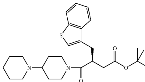
3 (S)-Benzo[b]thiophen-3-ylmethyl-4-[1,4']bipiperidiny-1'-yl-4-oxo-butyl ester
