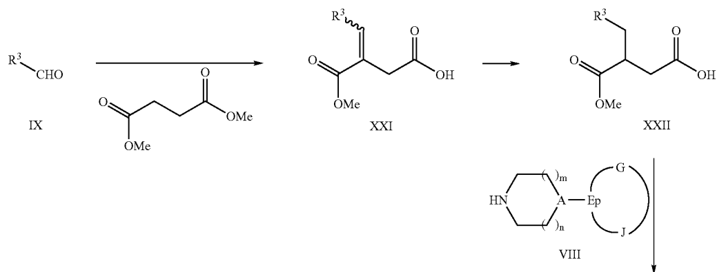
Scheme 7. Synthesis of Formula I Compounds
