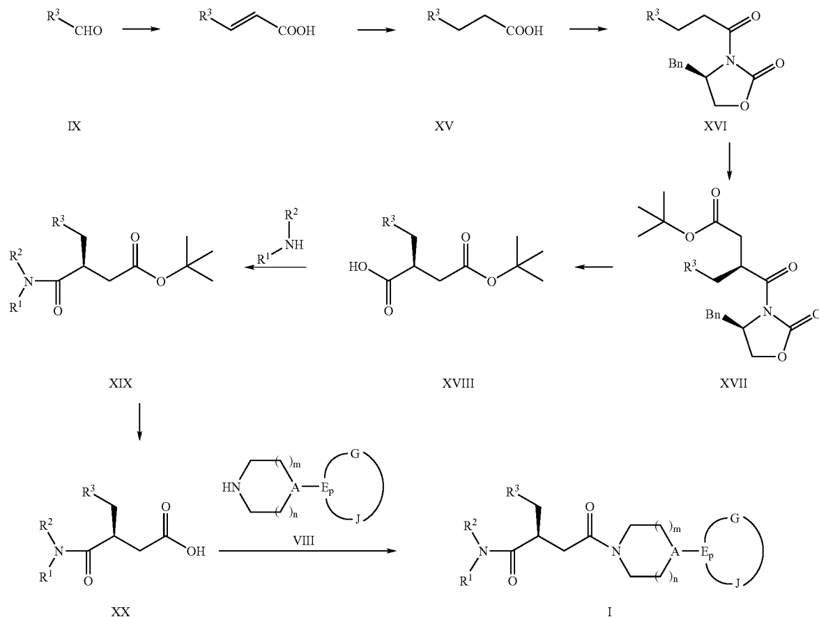
Scheme 5. Synthesis of Formula I Compounds
