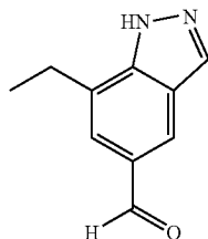
7-Ethyl-1H-indazole-5-carbaldehyde
