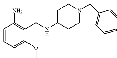
(2-Amino-6-methoxy-benzyl)-(1-benzyl-piperidin-4-yl)-amine
