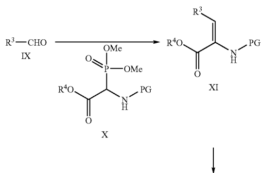
Scheme 4. Synthesis of Formula II and Formula V Compounds
