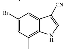
5-Bromo-7-methyl-1H-indole-3-carbonitrile
