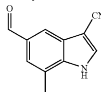
5-Formyl-7-methyl-1H-indole-3-carbonitrile
