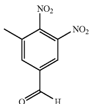
3-Methyl-4,5-dinitrobenzaldehyde
