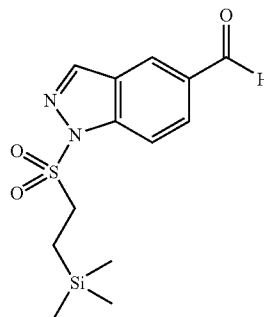
1-(2-Trimethylsilylanyl-ethanesulfonyl)-1H-indazole-5-carbaldehyde
