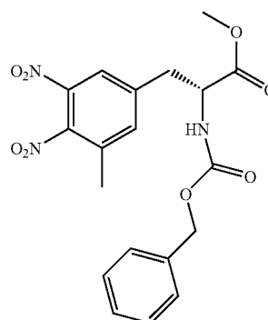
Benzyl (R)-1-(methoxycarbonyl)-2-(3-methyl-4,5-dinitrophenyl)ethylcarbamate
