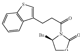
3-(3-Benzo[b]thiophen-3-yl-propionyl)-4(R)-benzyl-oxazolidin-2-one
