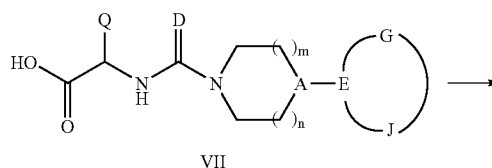
Scheme 3. Synthesis of Formula I Compounds
