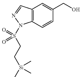
[1-(2-Trimethylsilylanyl-ethanesulfonyl)-1H-indazol-5-yl]-methanol
