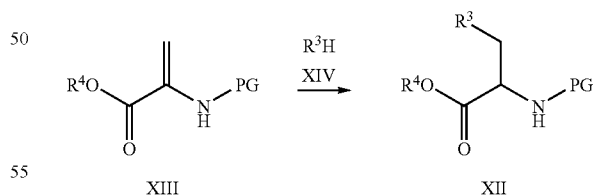
Scheme 5. Synthesis of Formula XII
