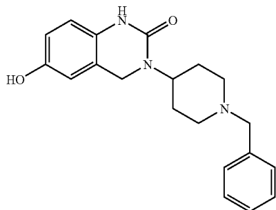
3-(1-Benzyl-piperidin-4-yl)-6-hydroxy-3,4-dihydro-1H-quinazolin-2-one
