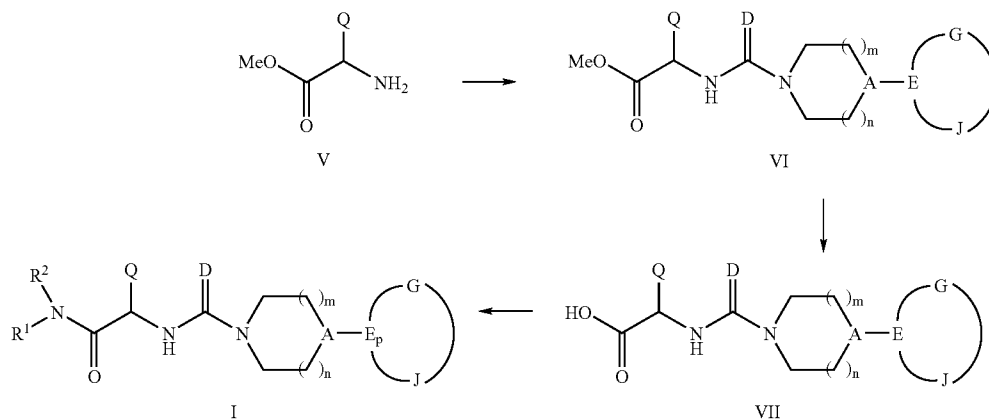
Scheme 2. Synthesis of Formula I Compounds
