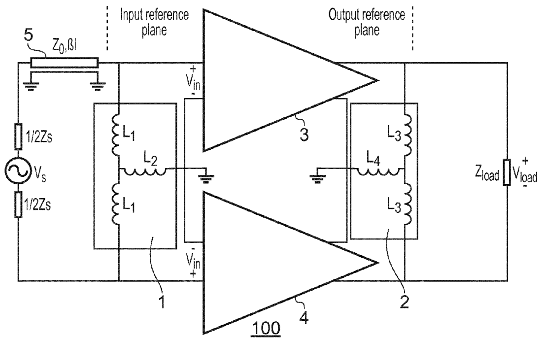
FIG. 2 A more detailed view of an RF front-end used in a transmitter
