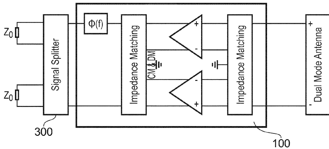
FIG. 9 A Radar and a wireless receiver
