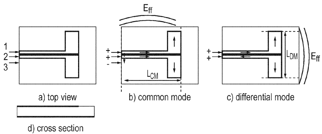
FIG. 10 A dual mode multiband antenna
