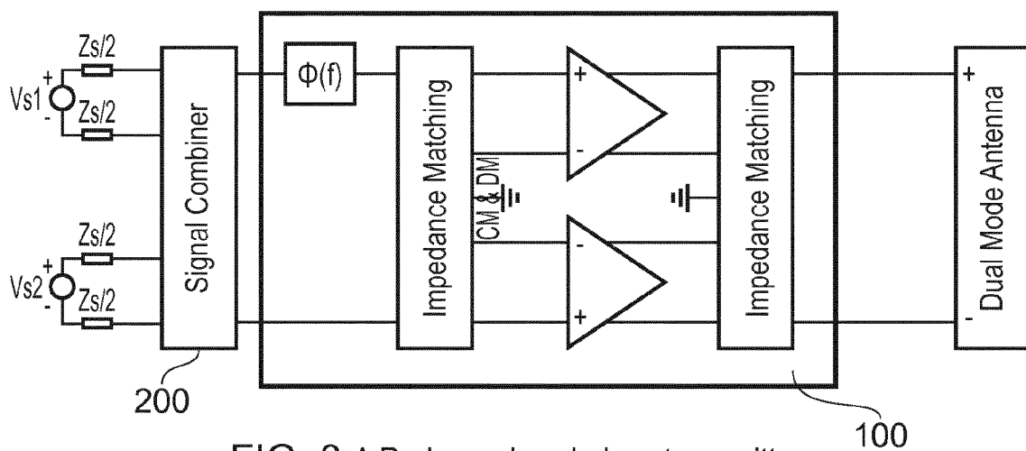
FIG. 8 A Radar and a wireless transmitter
