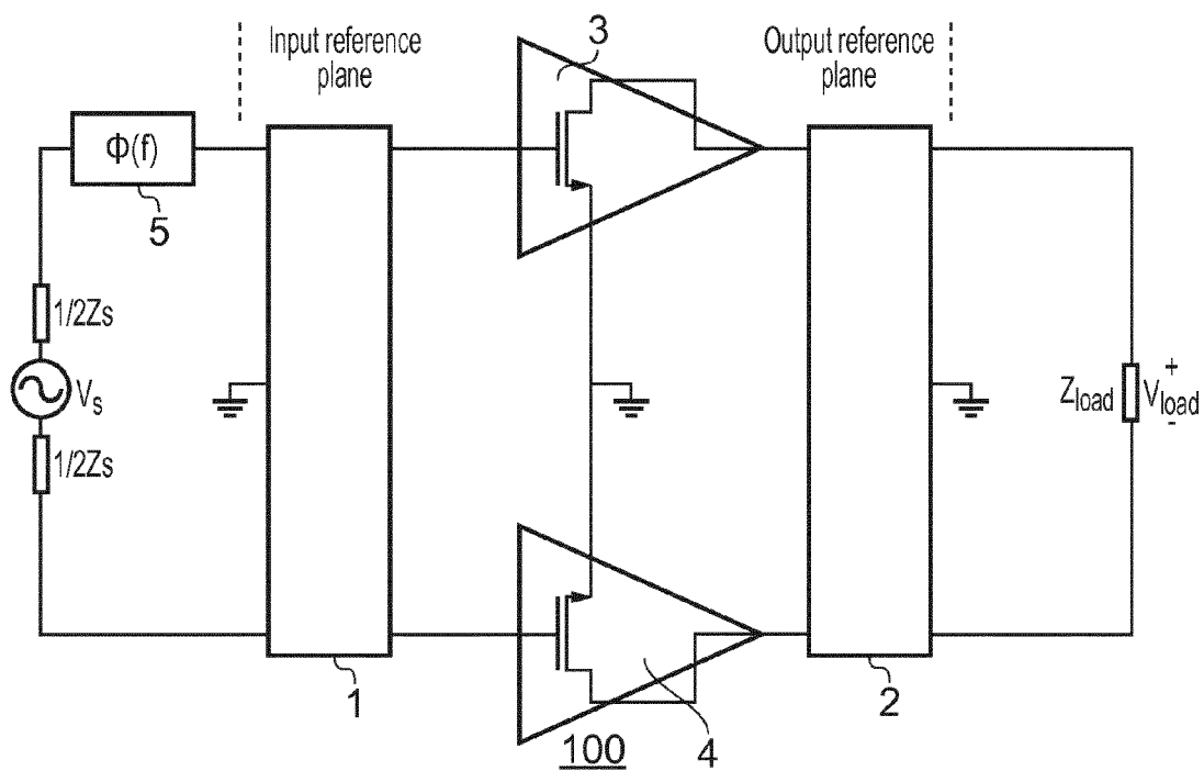
FIG. 4 Another embodiment of an RF front-end used in a transmitter
