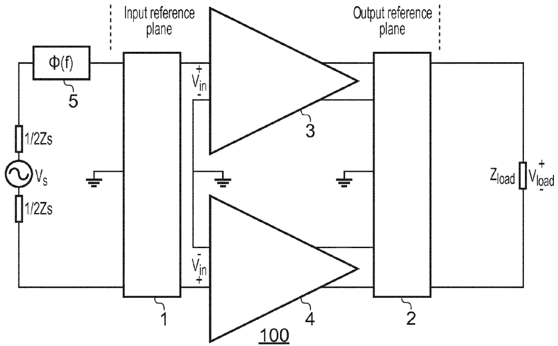
FIG. 1 An RF front-end used in a transmitter
