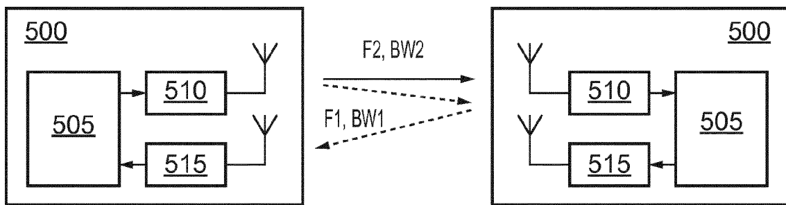
FIG. 6 A radar system with dual mode multiband antenna
