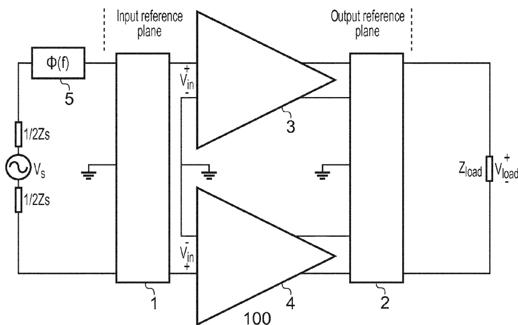
FIG. 1 An RF front-end used in a transmitter
