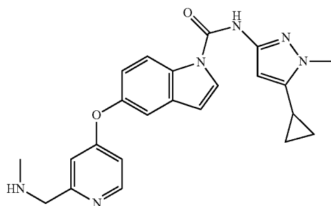
149-D. N-(5-cyclopropyl-1-methyl-1H-pyrazol-3-yl)-5-(2-((methylamino)methyl)pyridin-4-yloxy)-1H-indole-1-carboxamide
