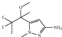
130-C. 1-Methyl-5-(2,2,2-trifluoro-1-methoxy-1-methyl-ethyl)-1H-pyrazol-3-ylamine
