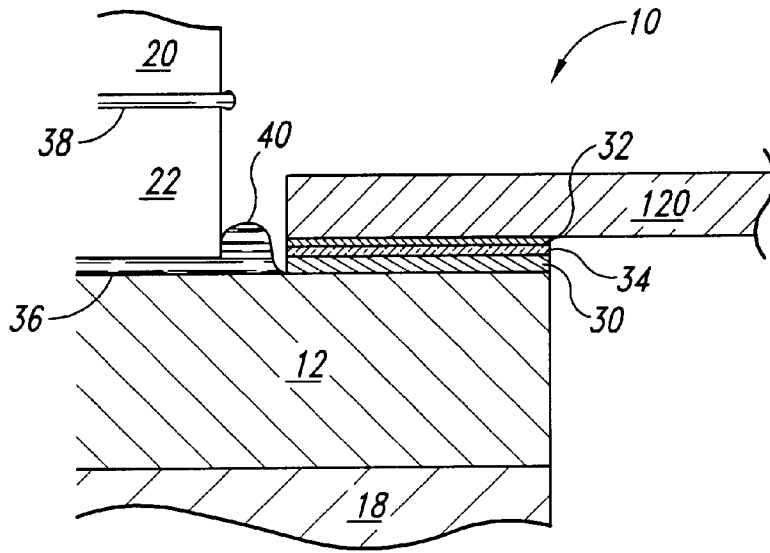
Fig. 1C (Prior Art)
