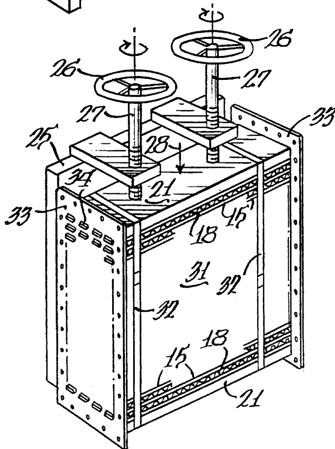
FIG. 3. CORE AND HEADER ASSEMBLY
