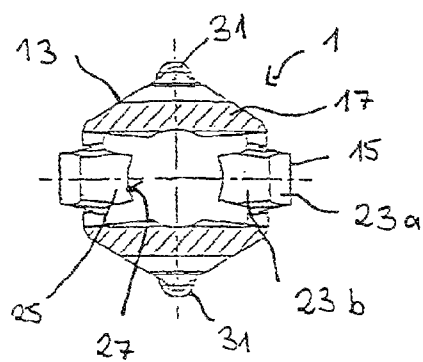
Fig. 3 (SECTION VIEW E-E)
