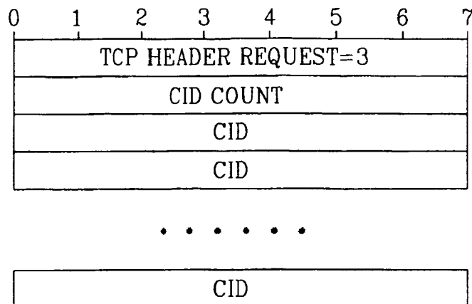
2/13 FIG. 3 RELATED ART
