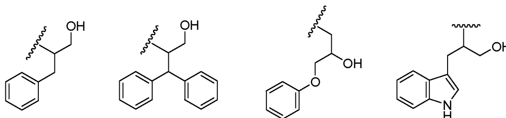
[Chemical formula 37]
