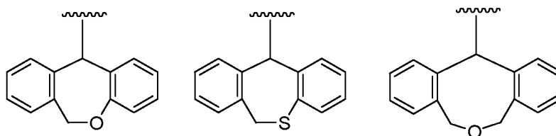
[Chemical formula 36]
