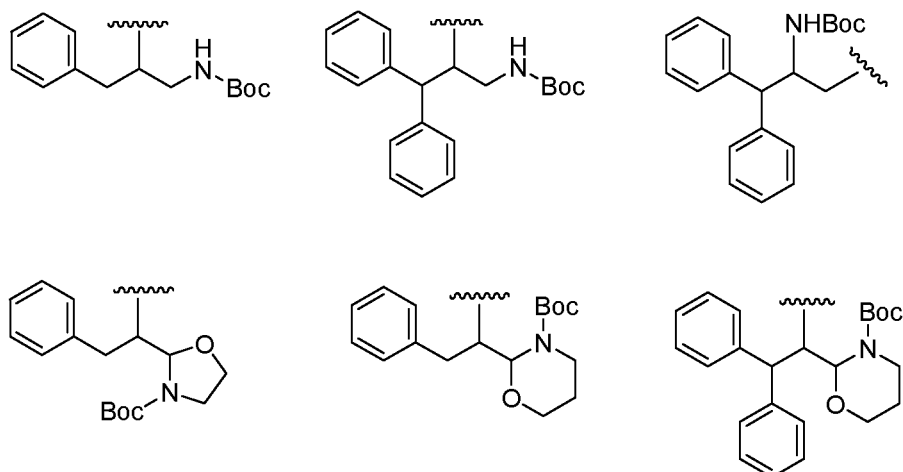
[Chemical formula 47]
