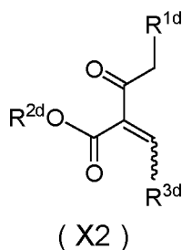
[Chemical formula 1]
