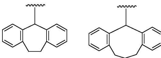
[Chemical formula 35]
