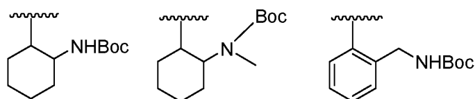
[Chemical formula 48]
