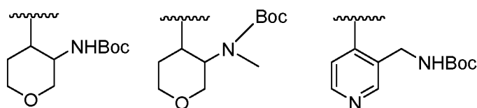
[Chemical formula 49]
