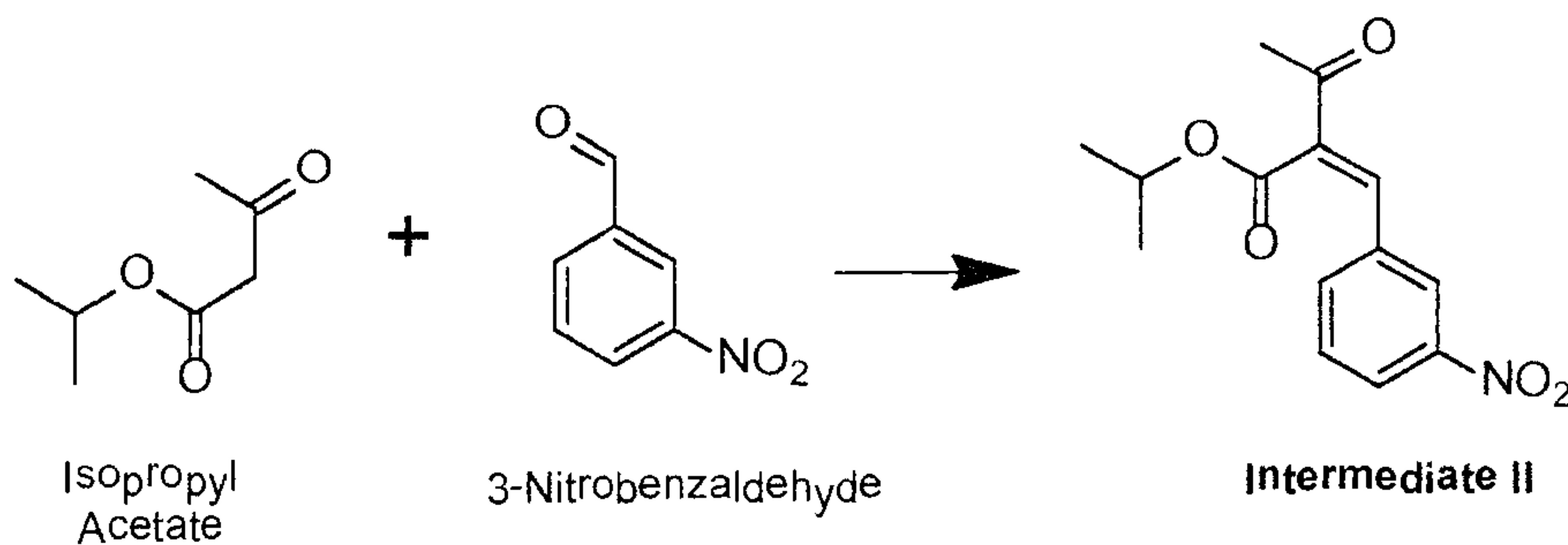
Scheme 2
