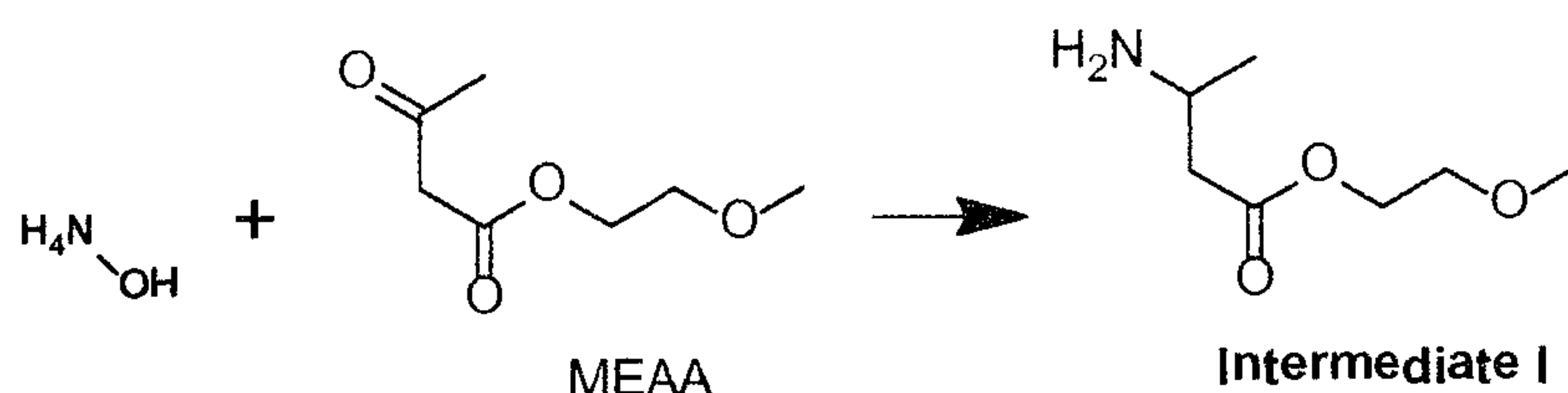
Scheme 1
