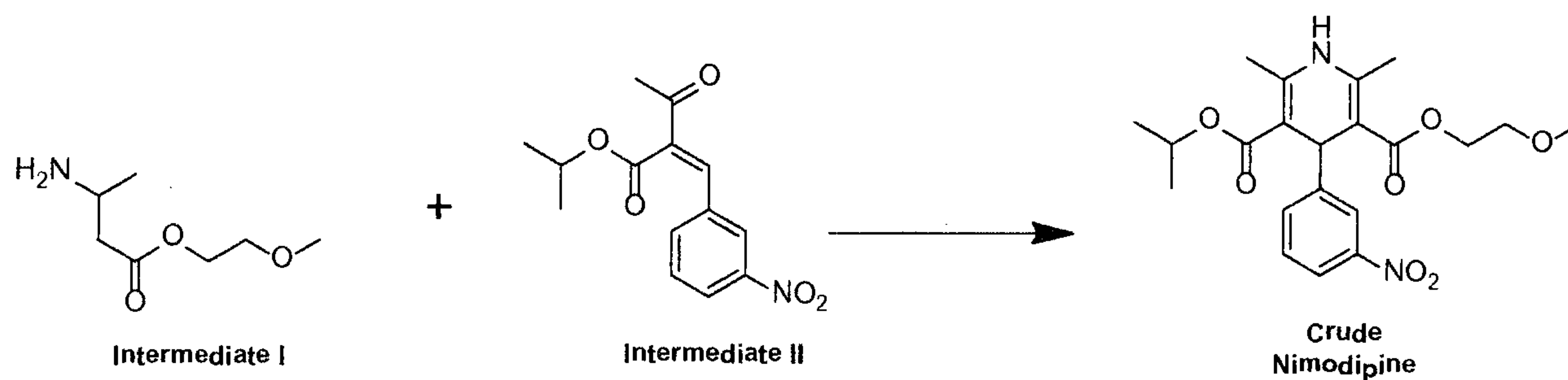
Scheme 3
