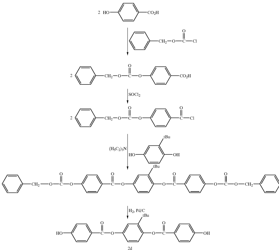
Reaction scheme 3
