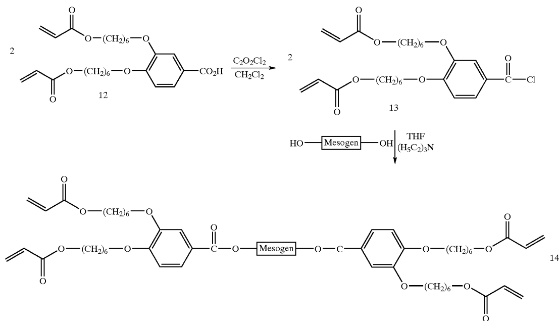
Reaction scheme 5
