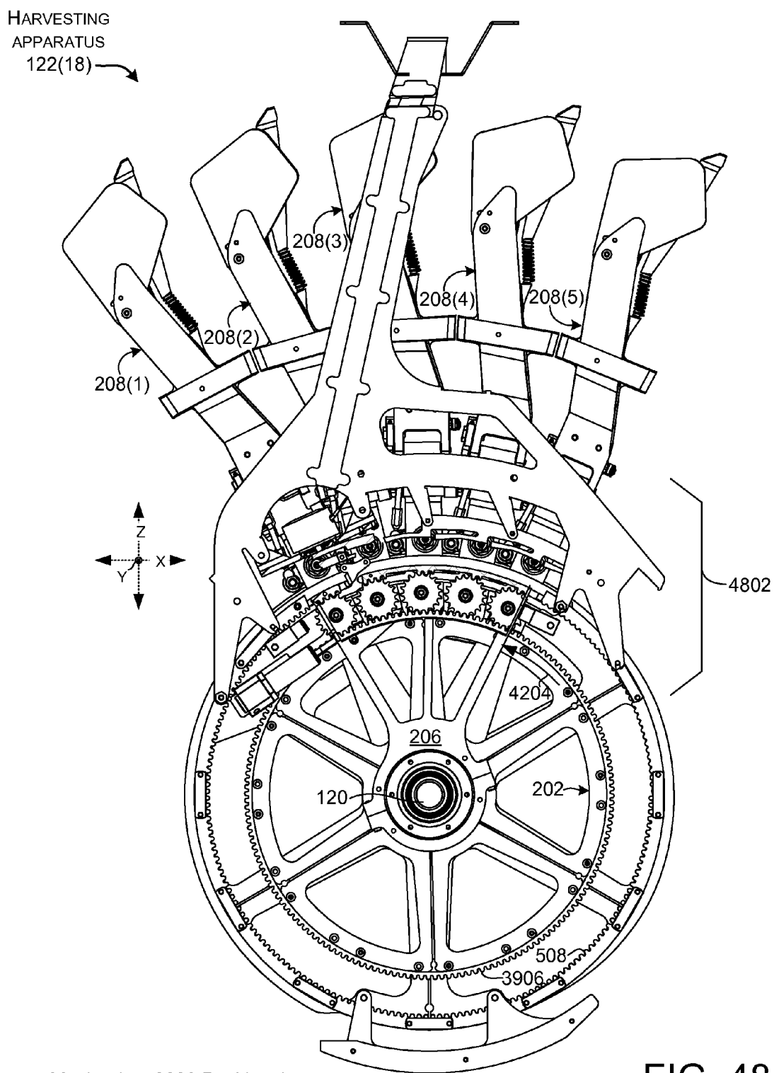
Mechanism 2009 Position 4
