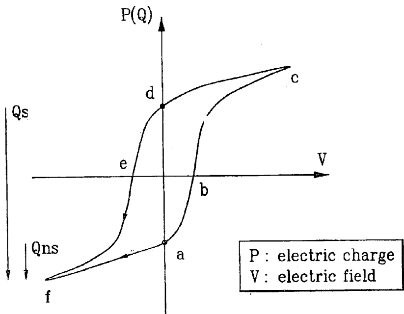
FIG. 1 Related Art
