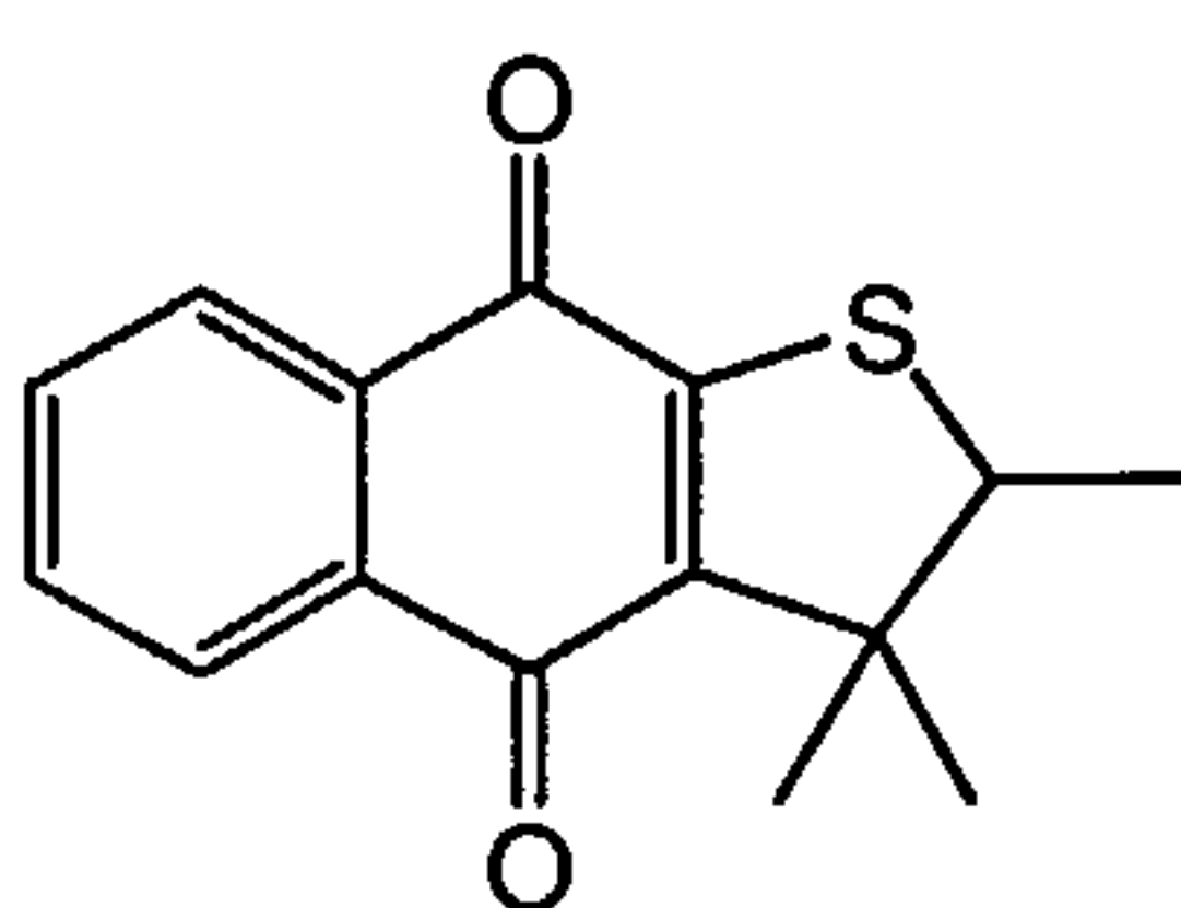
Compound 4
