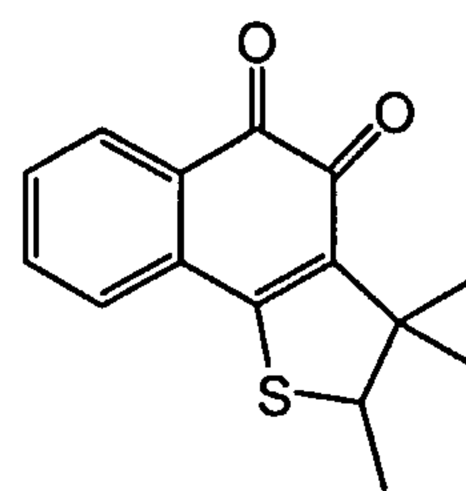
Compound 3
