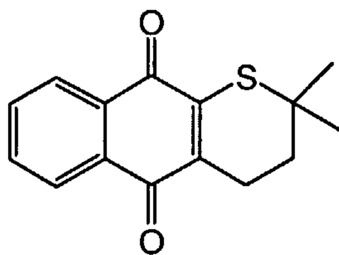
Compound 2
