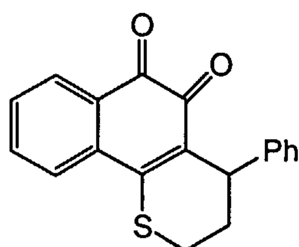
Compound 7
