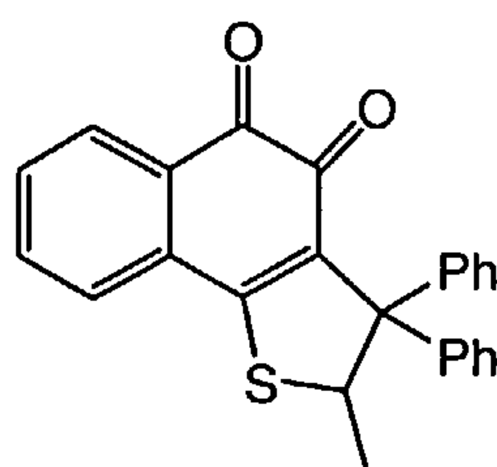
Compound 5
