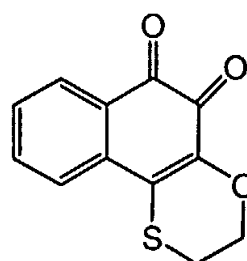
Compound 8
