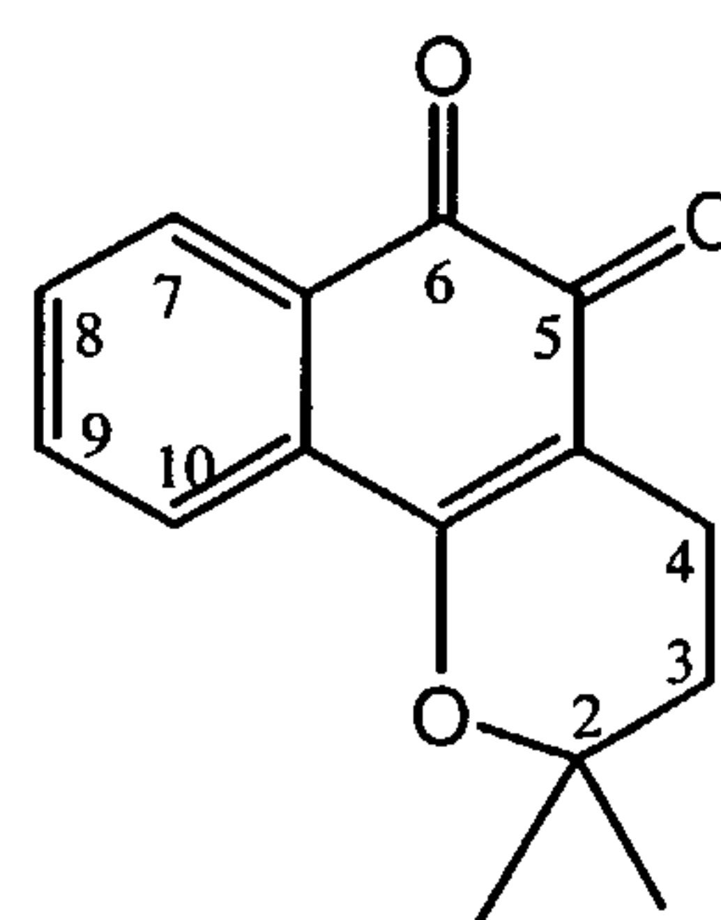
Beta-Lapachone
