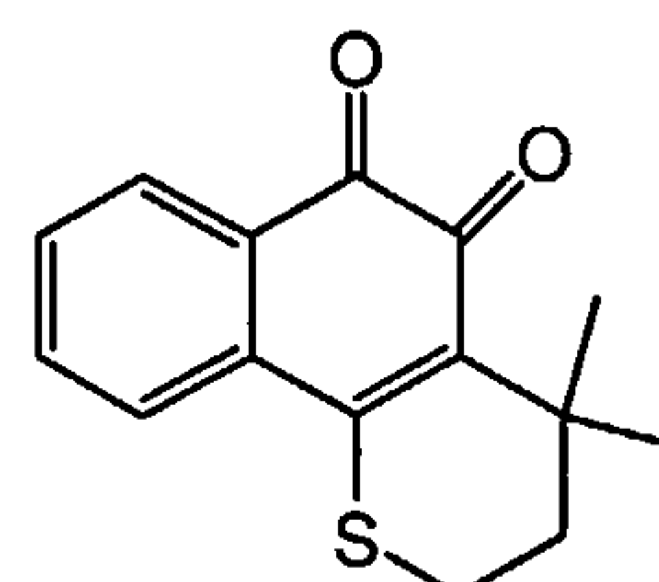
Compound 6
