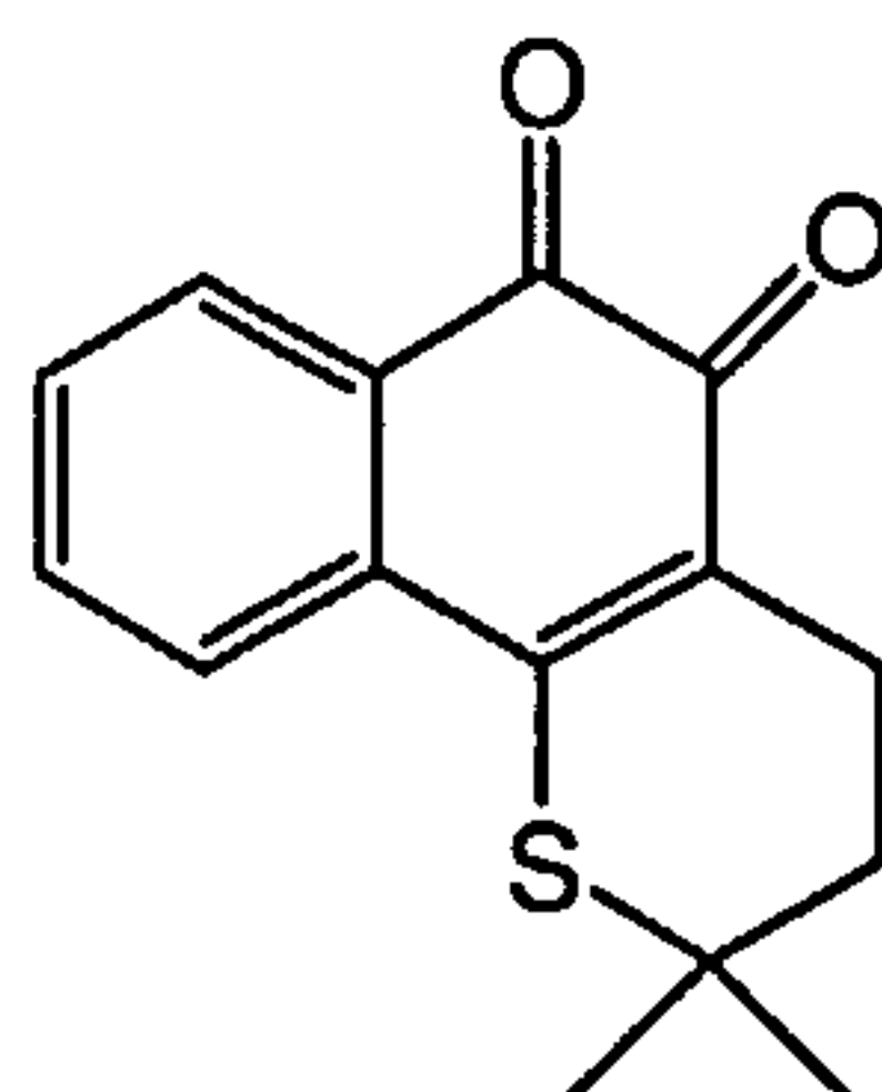
Compound 1
