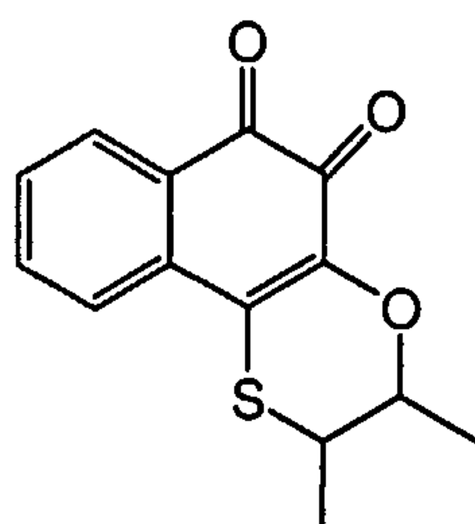
Compound 10
