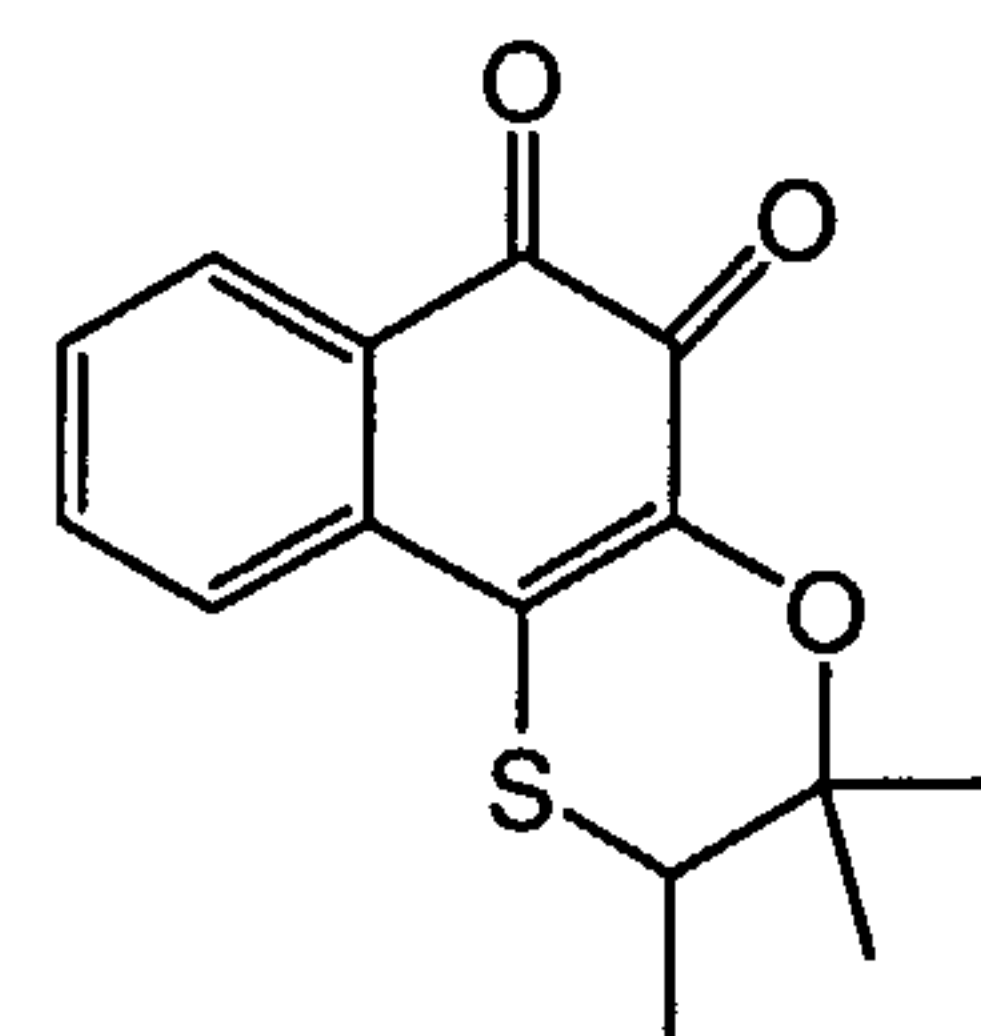
Compound 12
