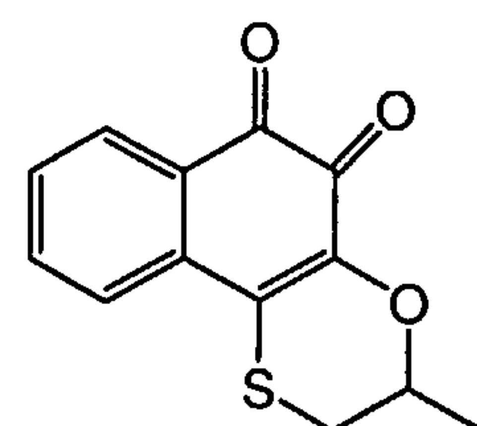
Compound 9
