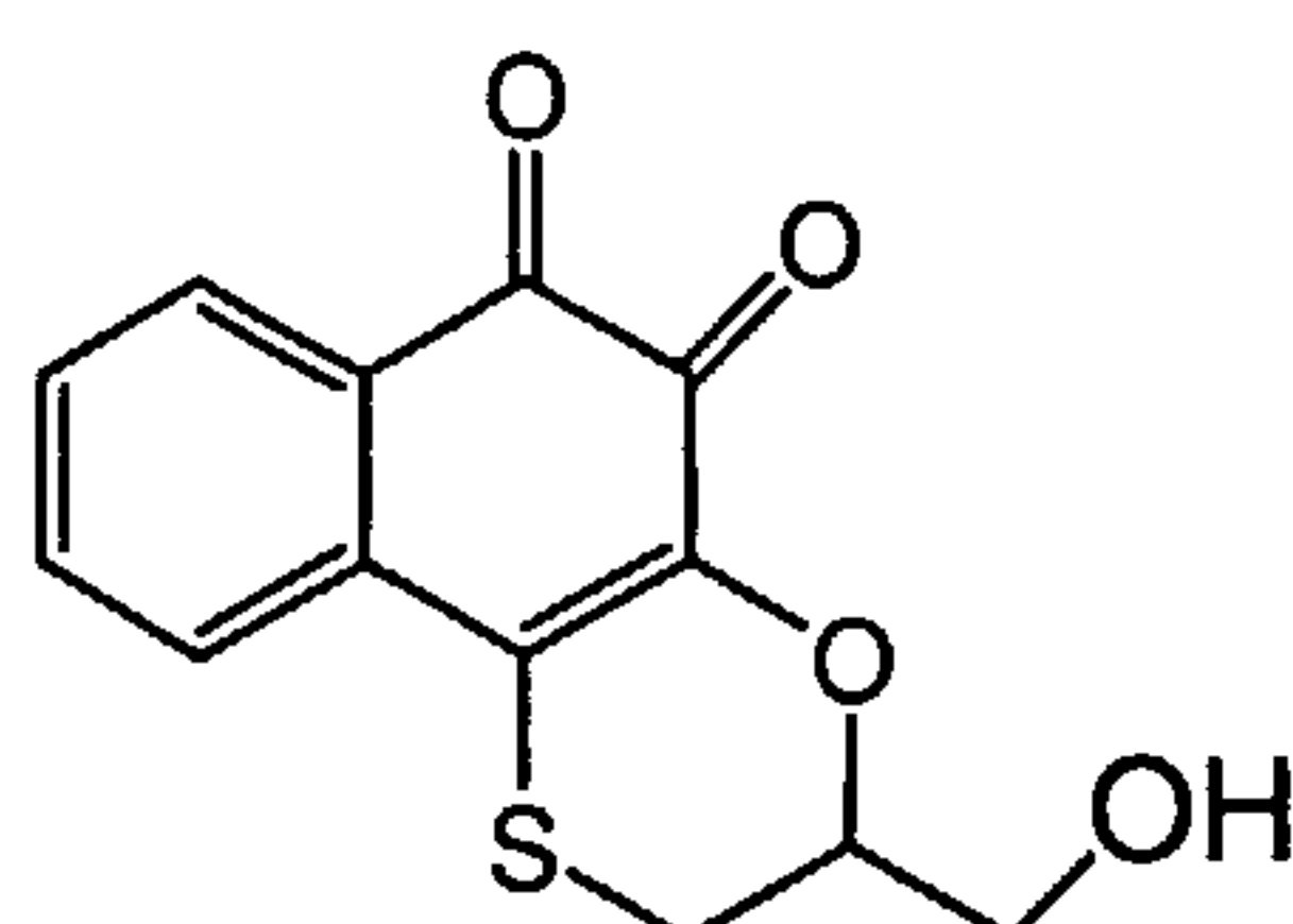
Compound 11
