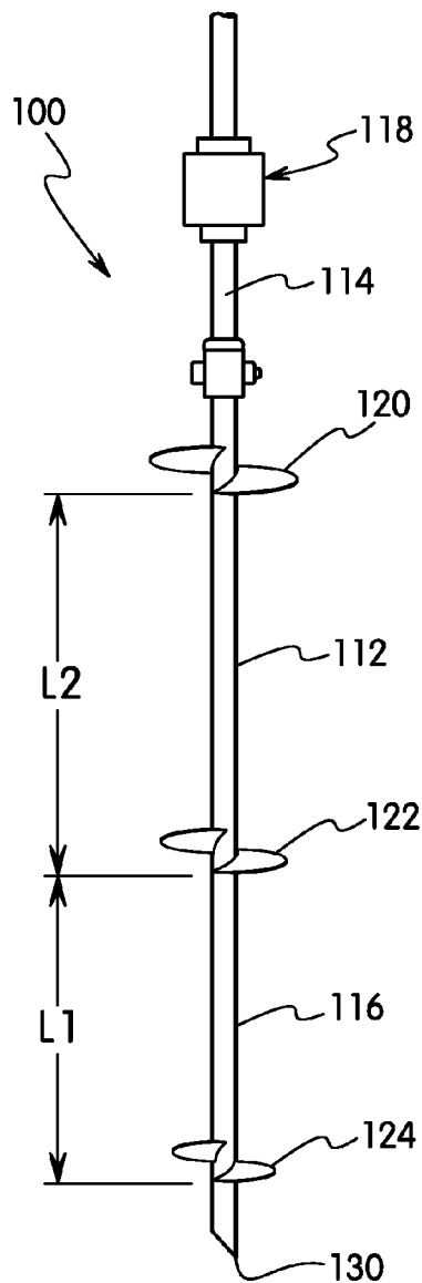
FIG. 1 (PRIOR ART)
