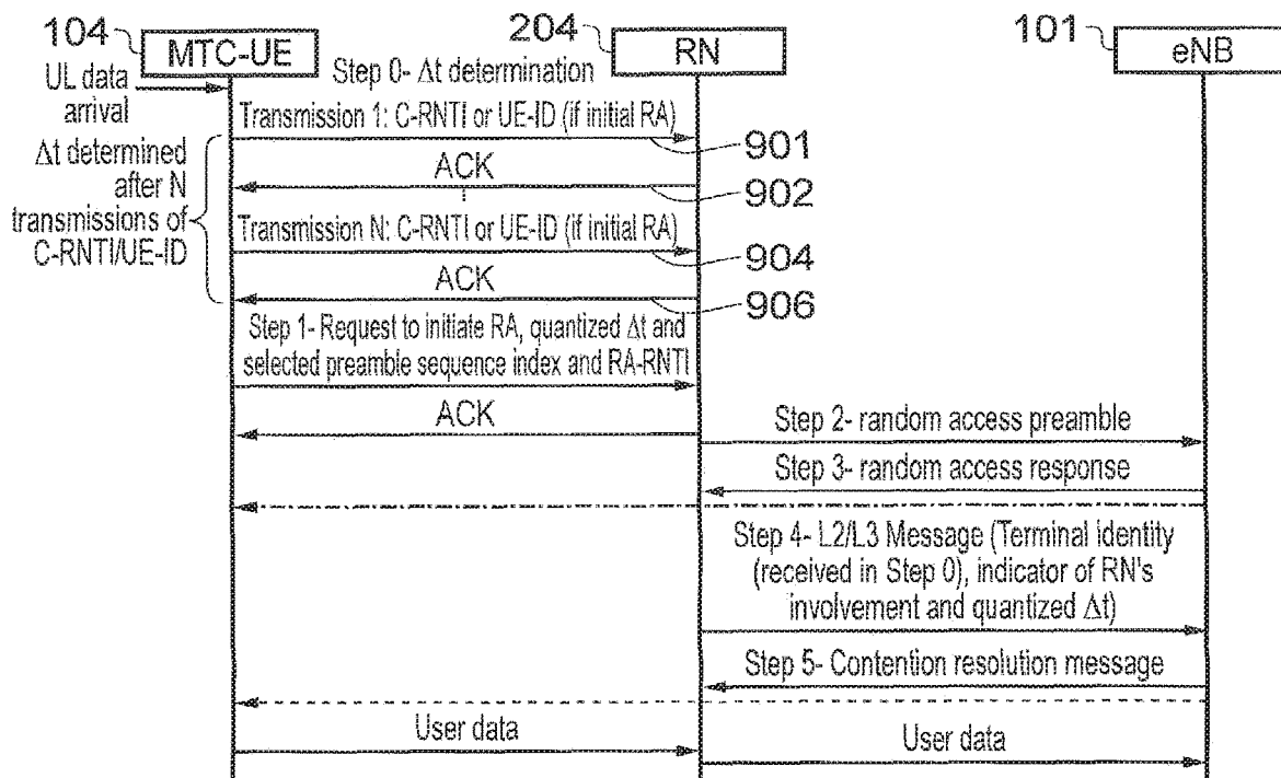
FIG. 9 Random Access procedure through RN (Solution 1)
