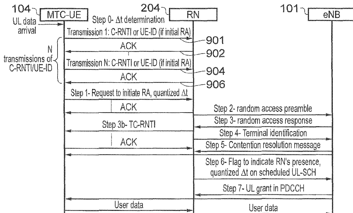
FIG. 12 Random Access procedure through RN (Solution 4)
