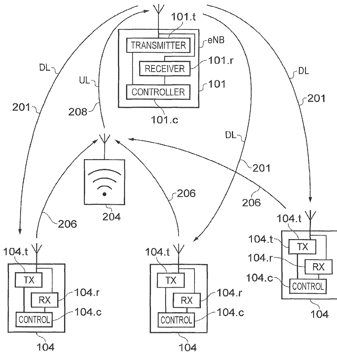
Example deployment of UEs and operation of an ad hoc relay node
