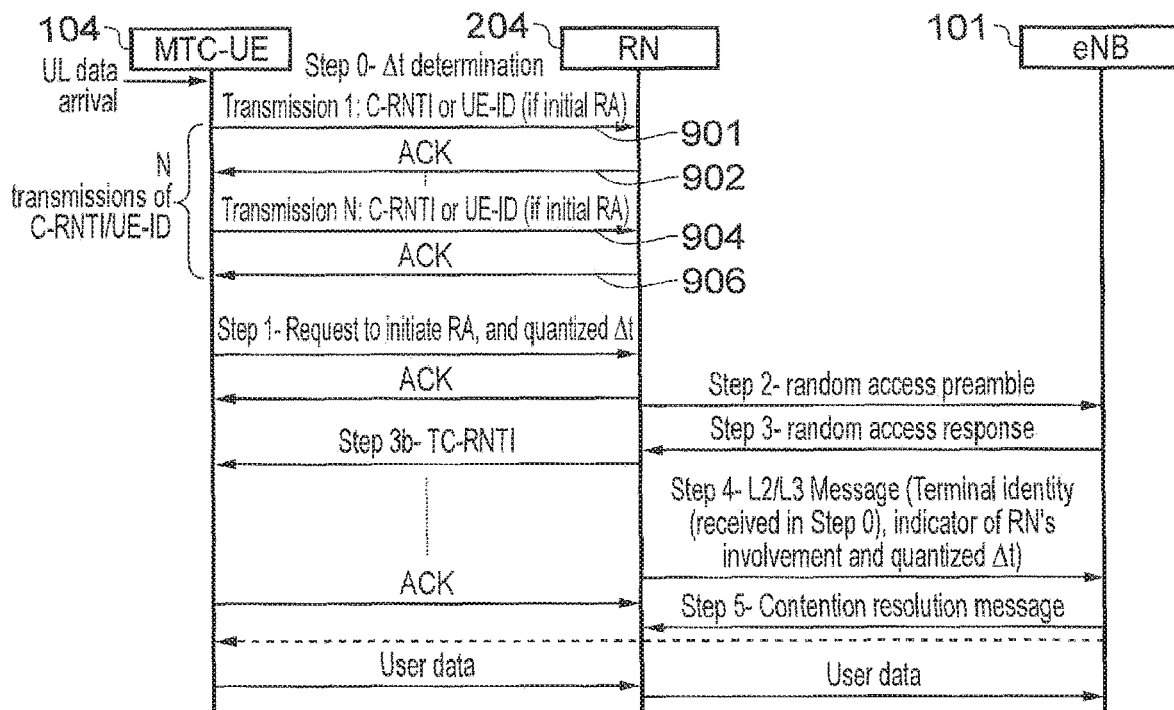
FIG. 10 Random Access procedure through RN (Solution 2)
