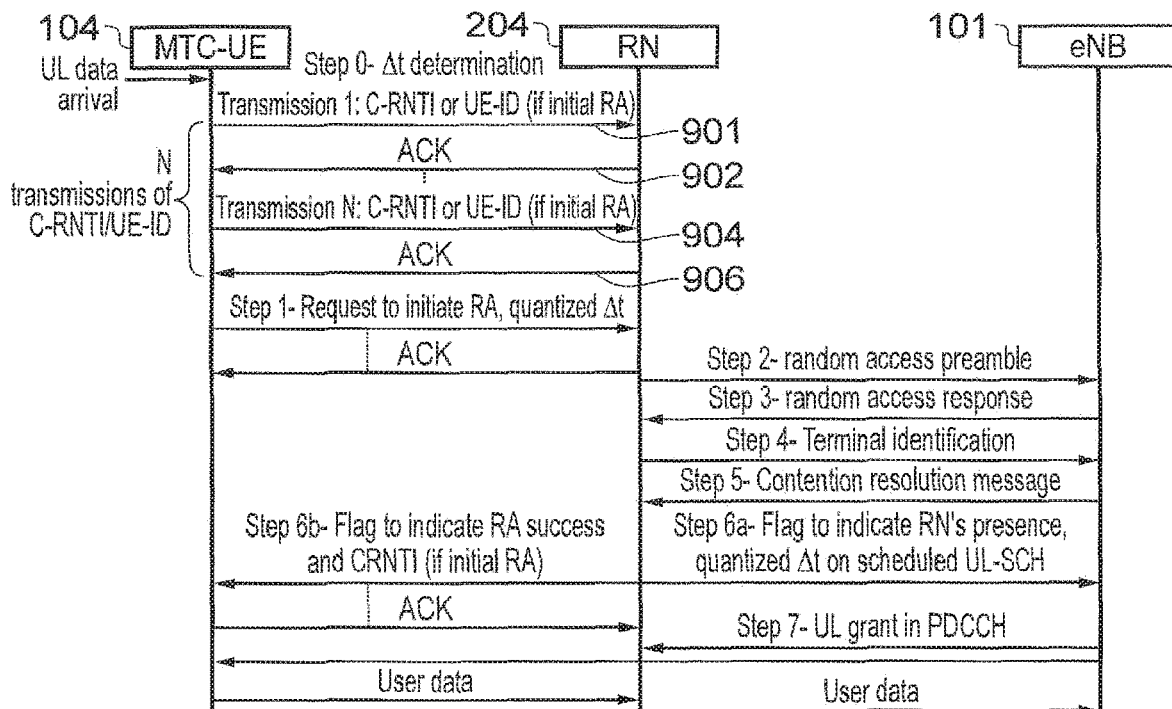
FIG. 11 Random Access procedure through RN (Solution 3)
