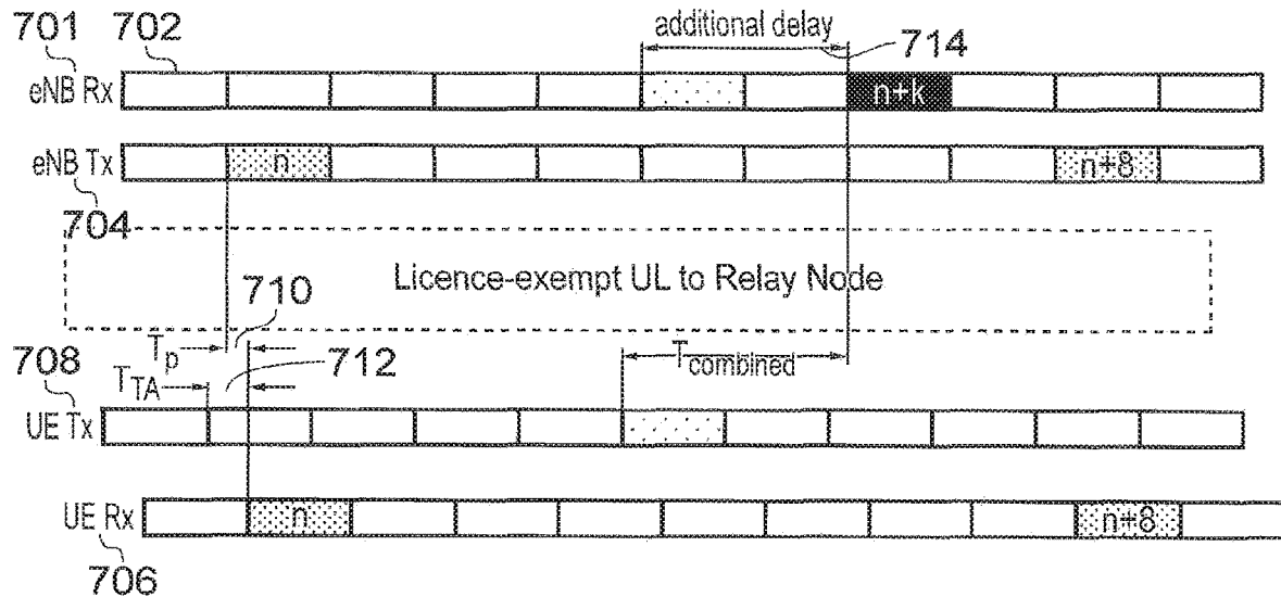
Timing diagram for determining UL delay from relaying
