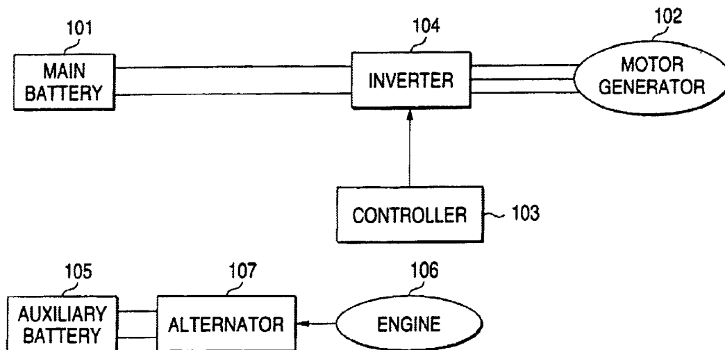
FIG. 13 PRIOR ART
