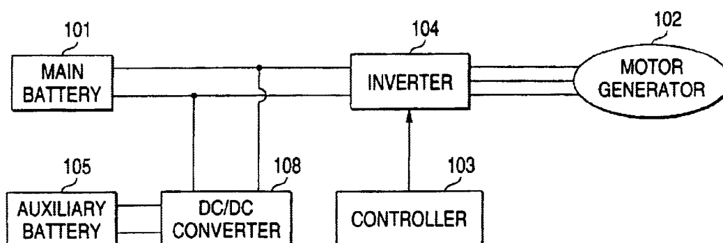
FIG. 14 PRIOR ART
