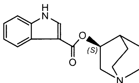
XXII (Compound 2)
