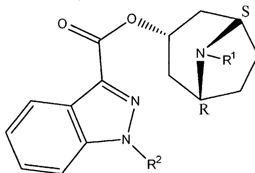
XIII
