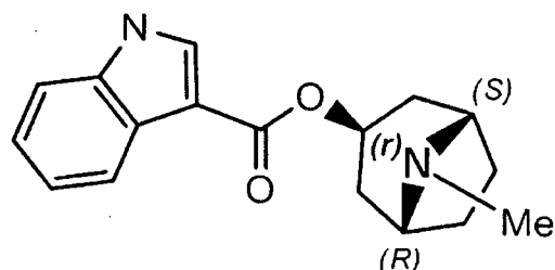
XXI (Compound 4)
