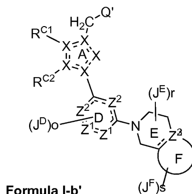
Formula I-b'
