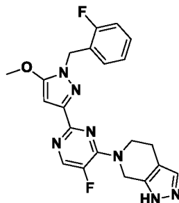
Compound I-6
