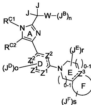
Formula IIE
