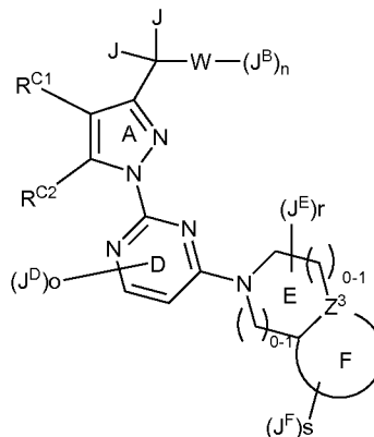
Formula IIIB.
