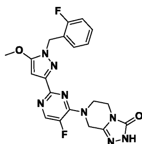
Compound I-2
