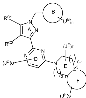
Formula IIIA'
