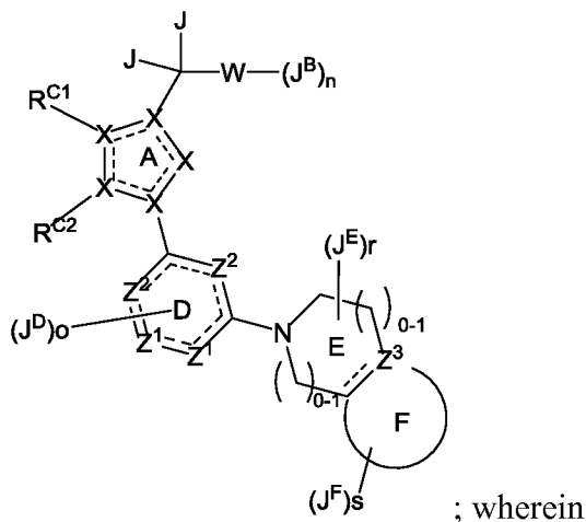
Formula I
