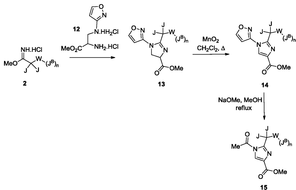
Scheme 7
