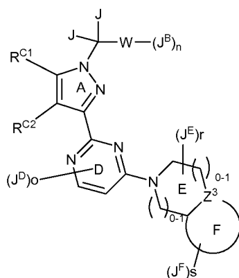
Formula IIIA
