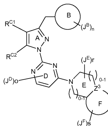
Formula IIIB';
