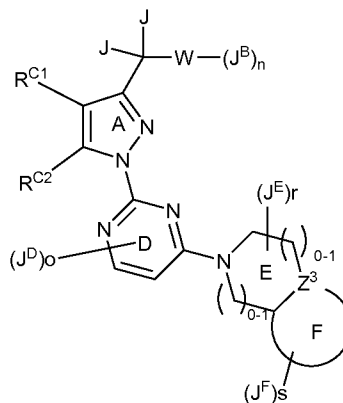
Formula IIIB.
