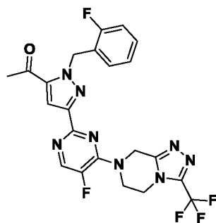
Compound I-13
