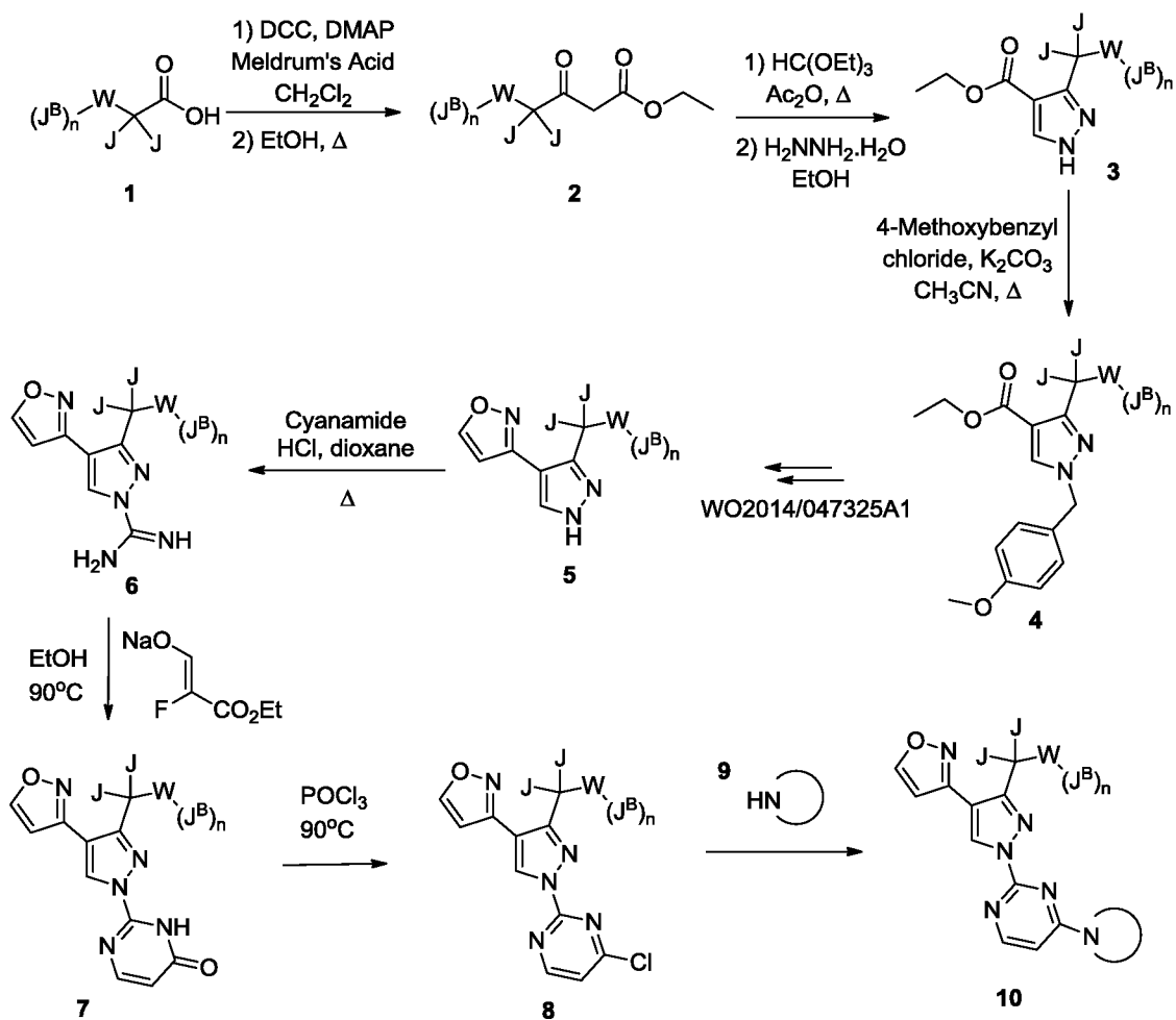
Scheme 1
