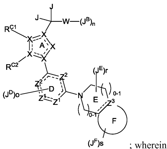
Formula I
