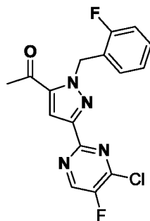
Intermediate-1C
