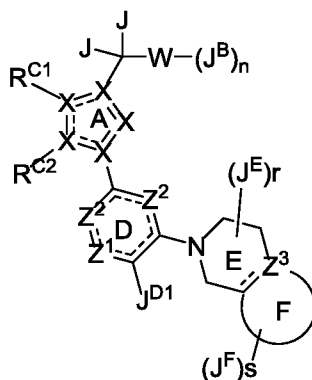
Formula I'B;
