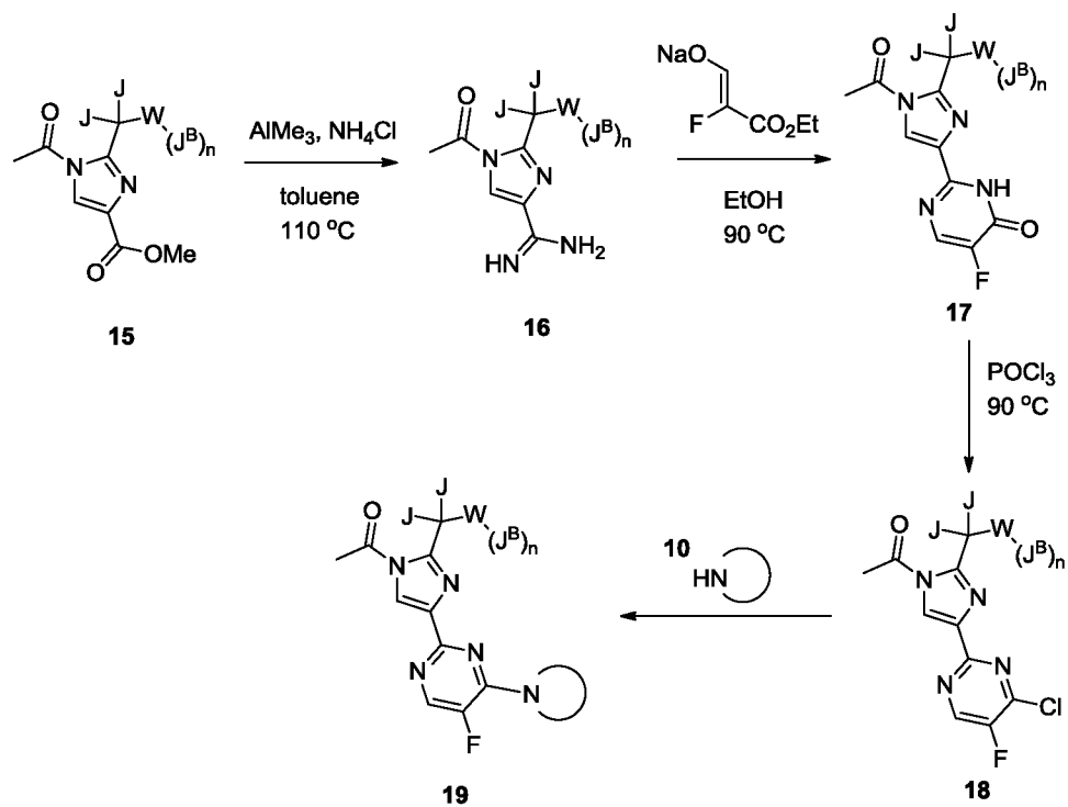
Scheme 11
