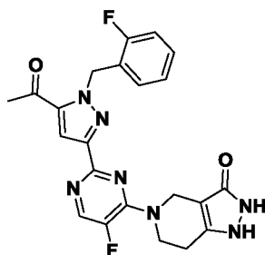
Compound I-16
