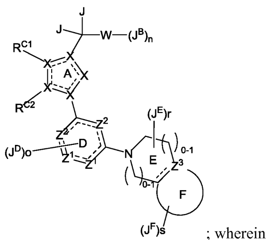
Formula I
