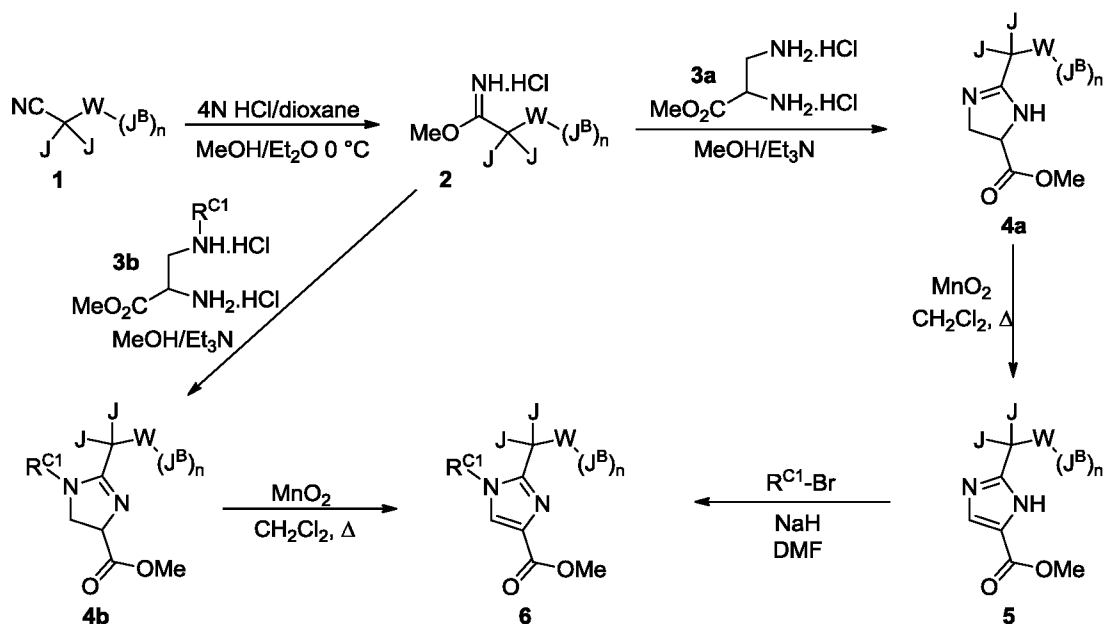
Scheme 8
