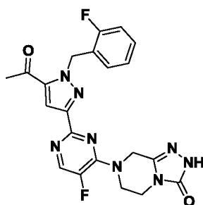
Compound I-14
