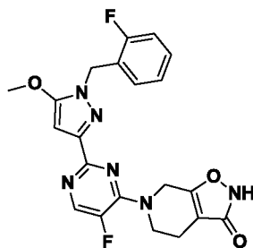
Compound I-5
