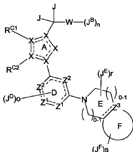
Formula I'
