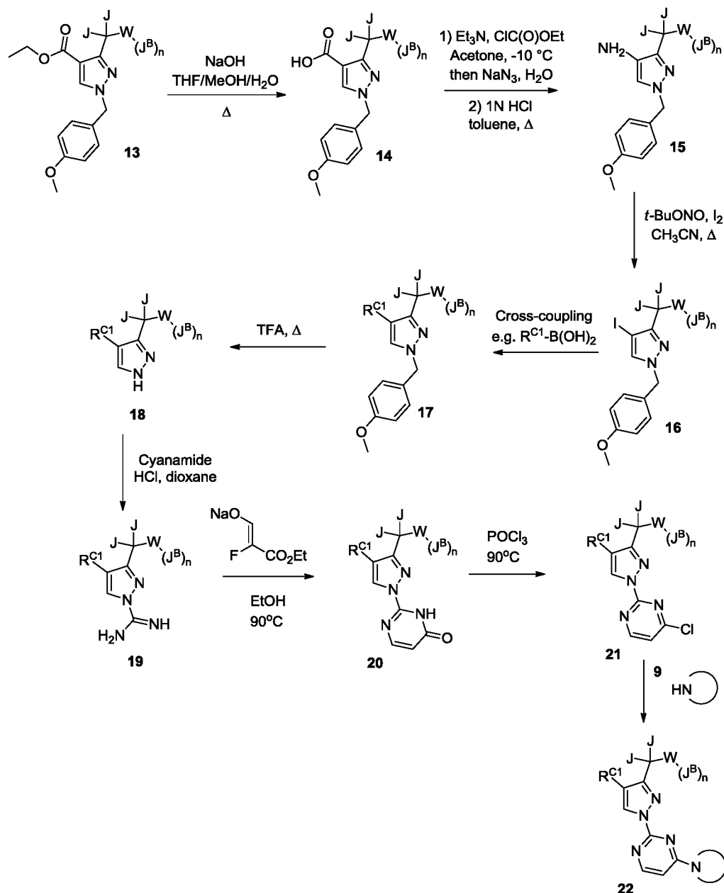
Scheme 3
