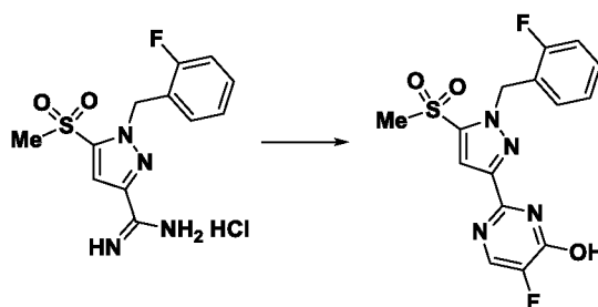
Intermediate 20
