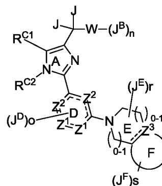
Formula IIF
