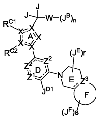
Formula I'B;
