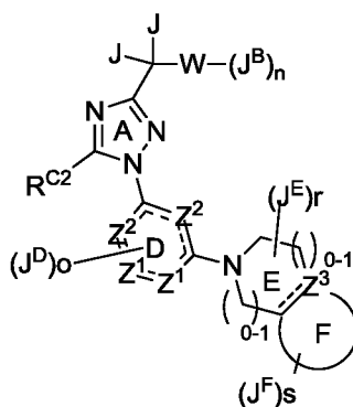
Formula IID
