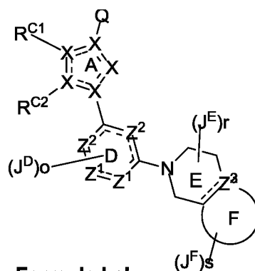
Formula I-a'
