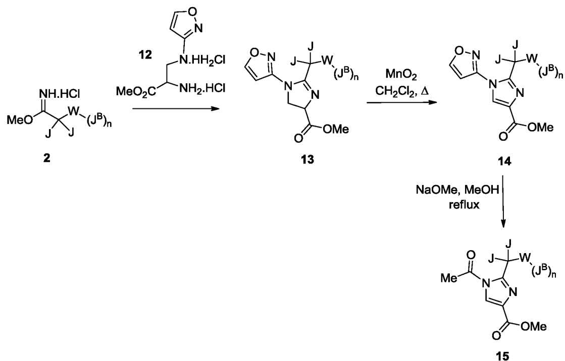
Scheme 11
