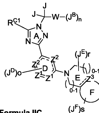
Formula IIC
