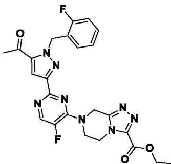
Compound I-18
