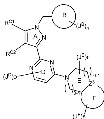
Formula IIIA'
