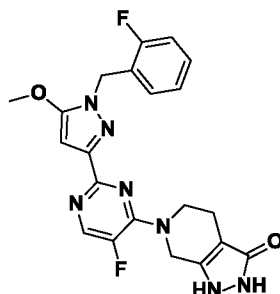
Compound I-7
