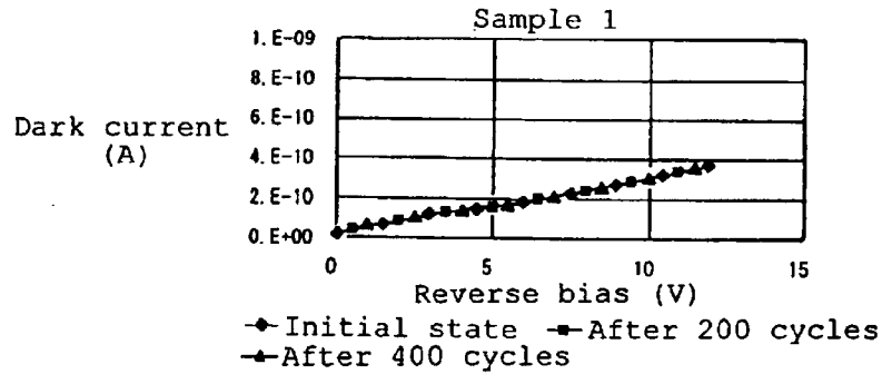
FIG. 2C-2 Temperature cycle test (-40 to 125 °C)
