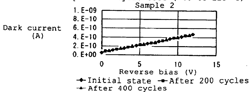
FIG. 2C-2 Temperature cycle test (-40 to 125 °C)
