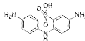
XC-ESI10 C_{12}H_{13}N_3O_3S Exact Mass: 279.0678 Mol. Wt.: 279.3149
