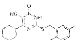
XC-ESI8 C_{20}H_{23}N_3OS Exact Mass: 353.1562 Mol. Wt.: 353.4611
