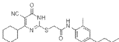
XC-ESI6 C_{24}H_{30}N_4O_3S Exact Mass: 438.2089 Mol. Wt.: 438.6856
