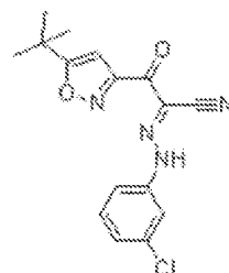
XC-ESI9 C_{16}H_{15}ClN_4O_2 Exact Mass: 330.0884 Mol. Wt.: 330.7689
