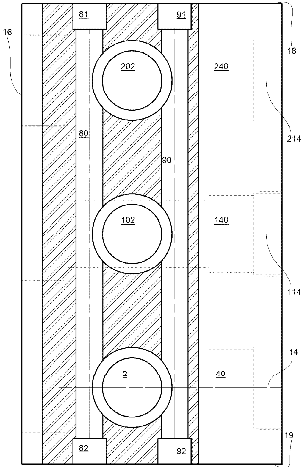
Section "C-C" of Figure 12A Figure 12C
