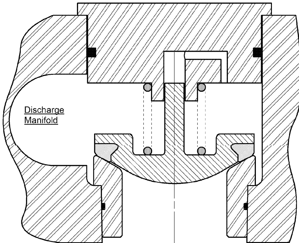
Detail "B-B" of Figure 6A
