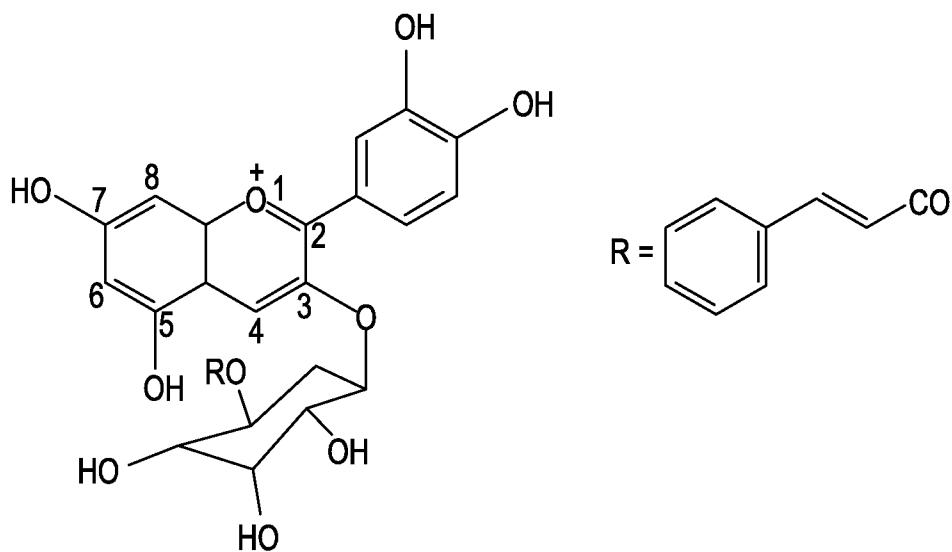
II: CYANIDIN -3- GLUCOSIDE-COUMARATE
