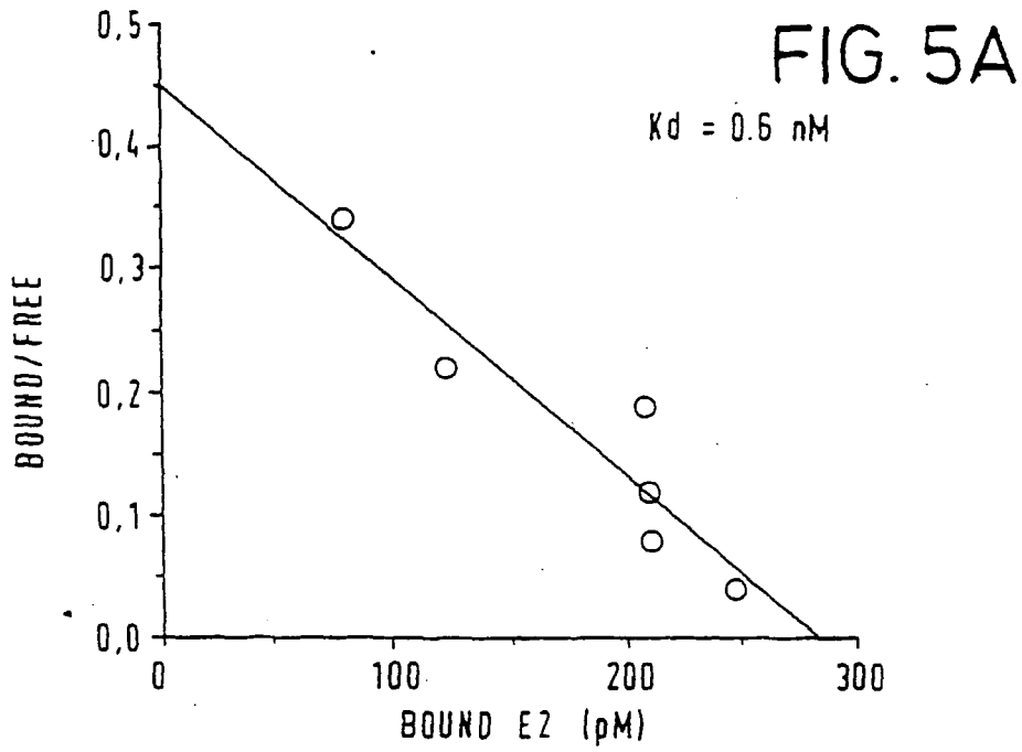
SCATCHARD PLOT OF ER-BETA
