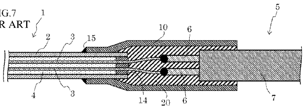
FIG. 8 PRIOR ART
