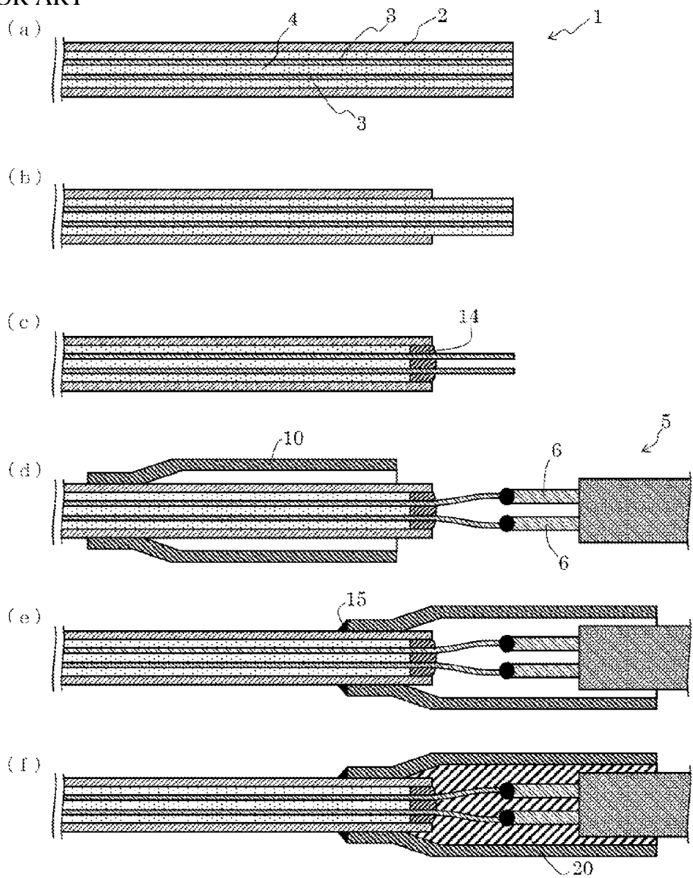
FIG. 9 PRIOR ART
