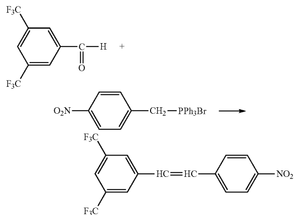
Reaction Formula (1)
