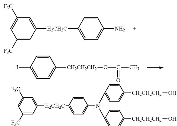
Reaction Formula (3)
