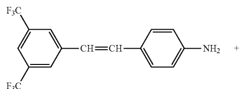
Reaction Formula (6)
