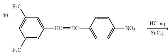
Reaction Formula (5)
