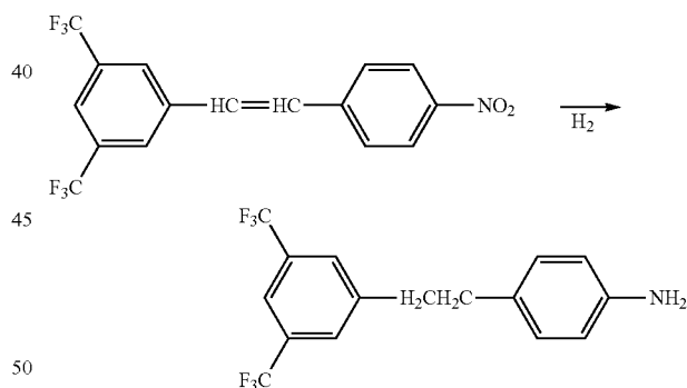
Reaction Formula (2)
