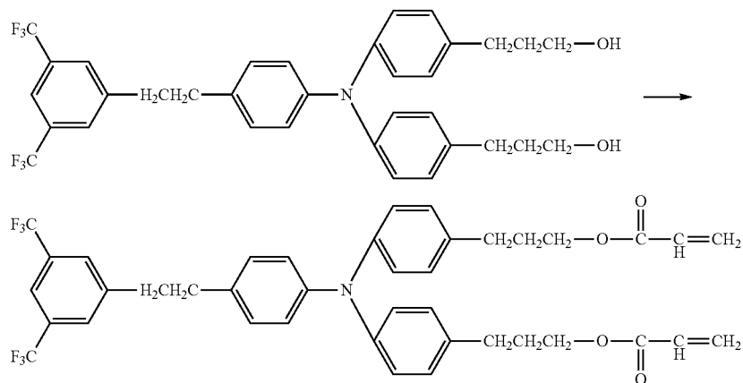
Reaction Formula (4)
