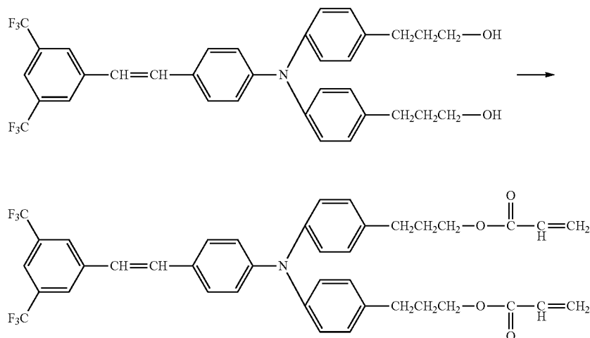
Reaction Formula (7)
