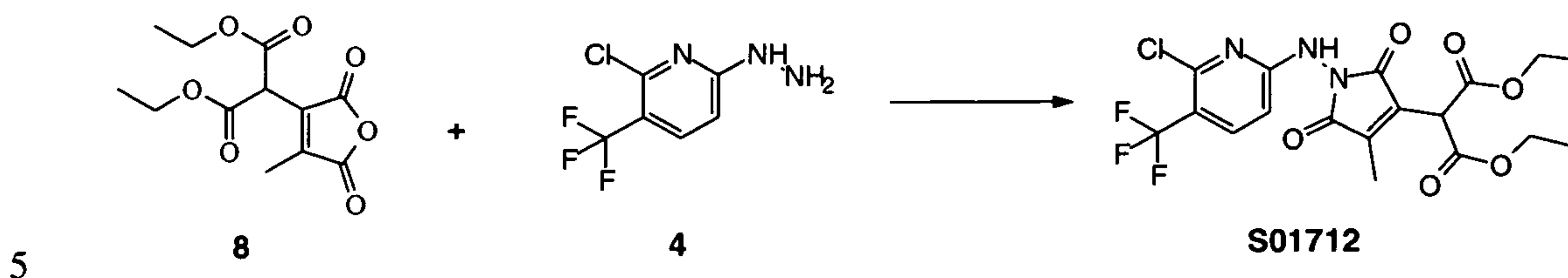
Scheme 13
