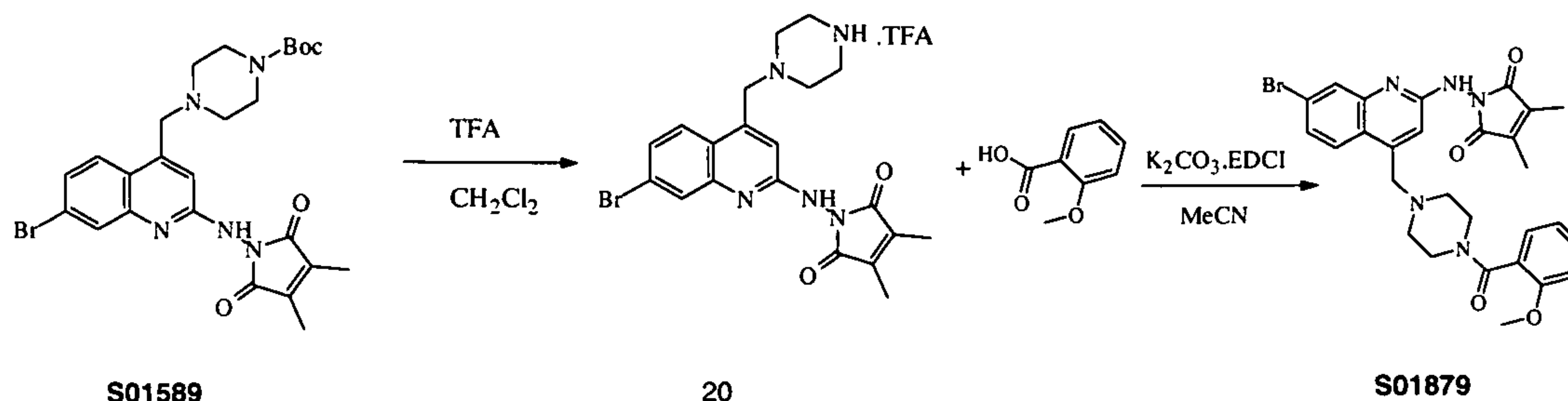
Scheme 8
