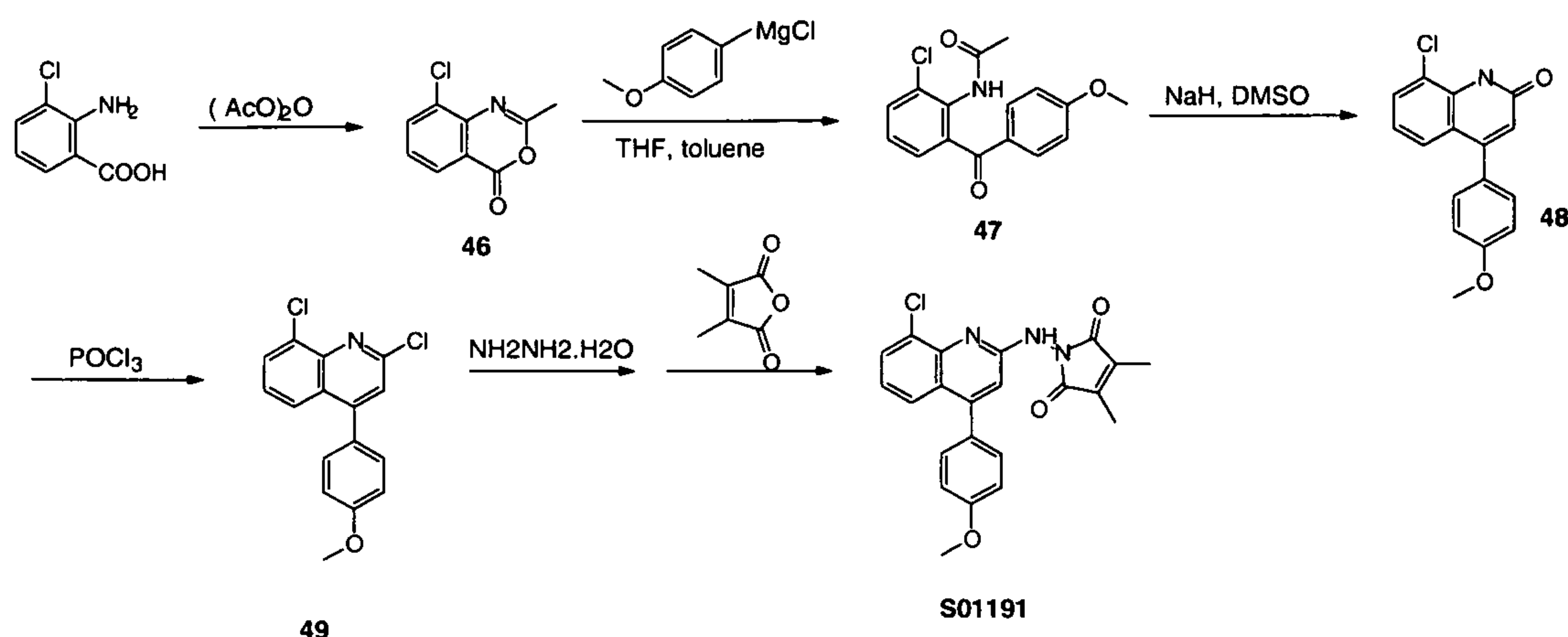
Scheme 24
