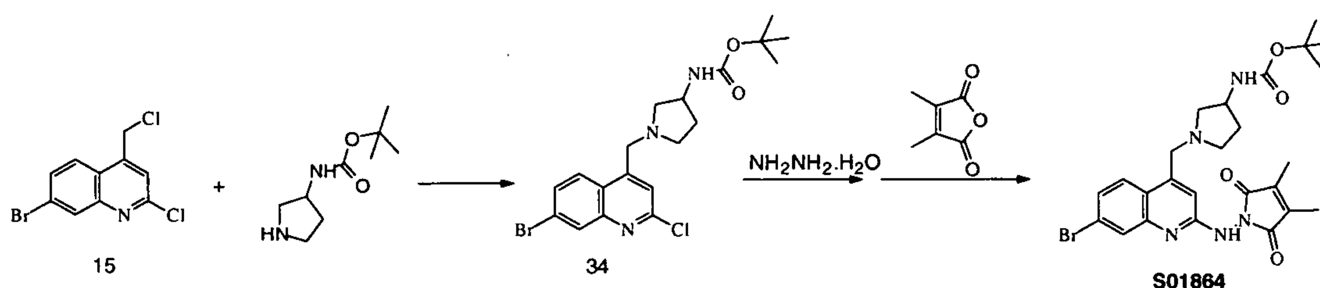
Scheme 18
