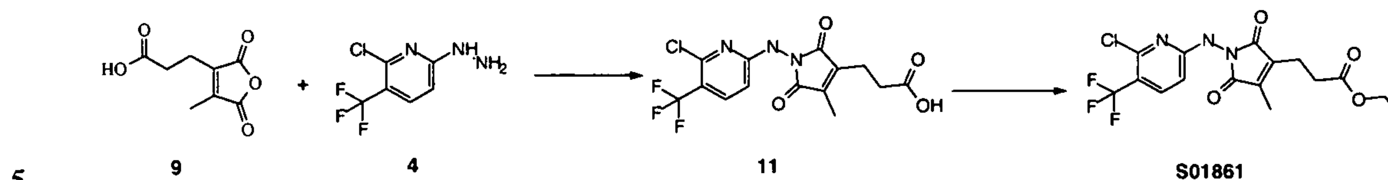
Scheme 5
