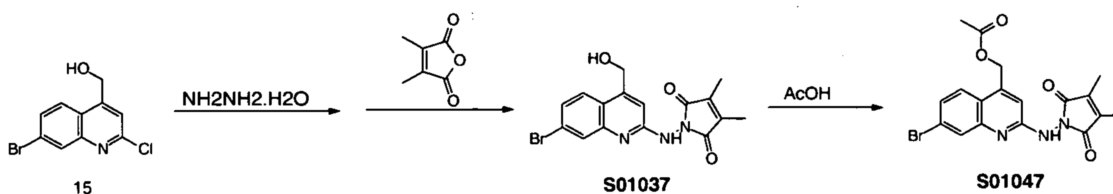
Scheme 7
