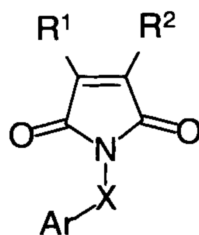
(I)
