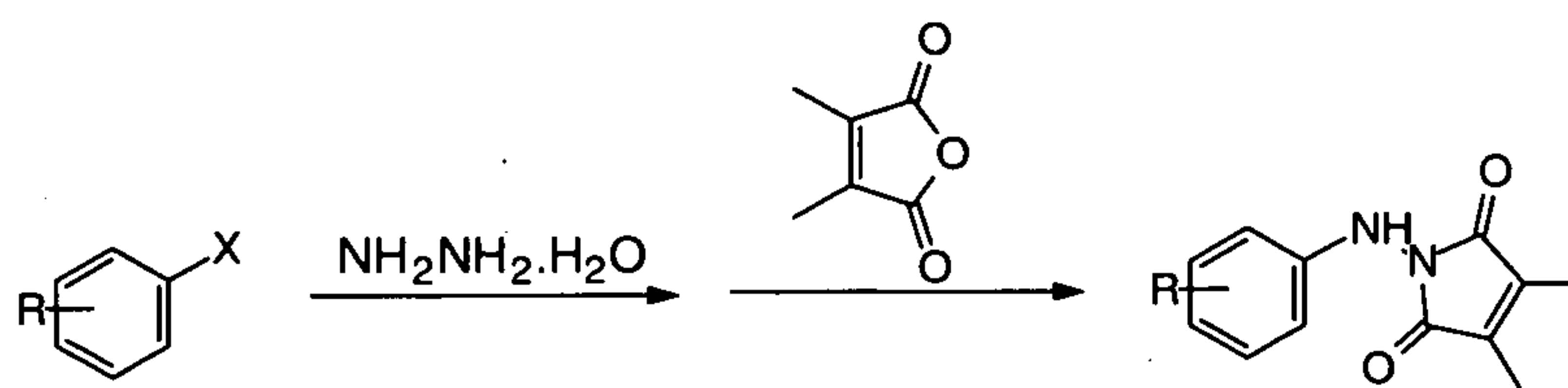
Scheme 1
