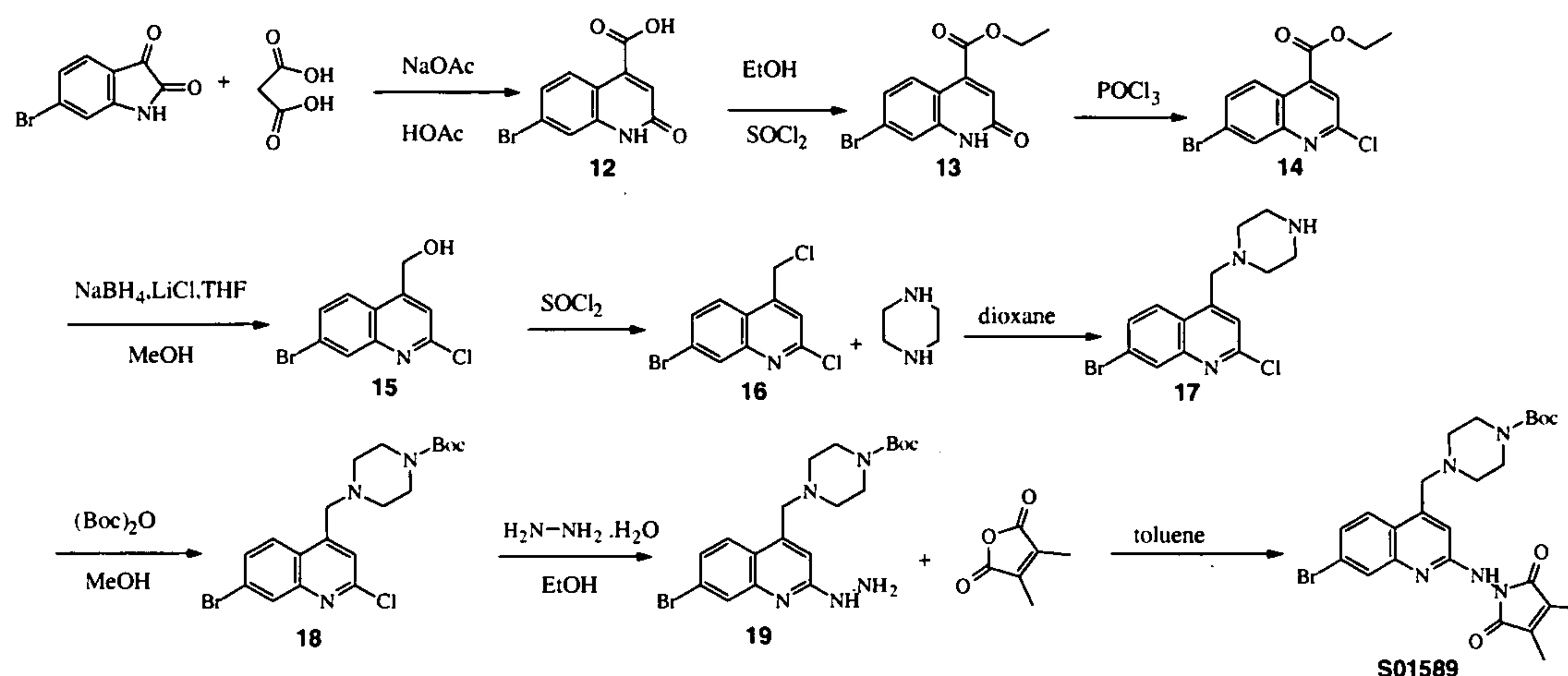
Scheme 6
