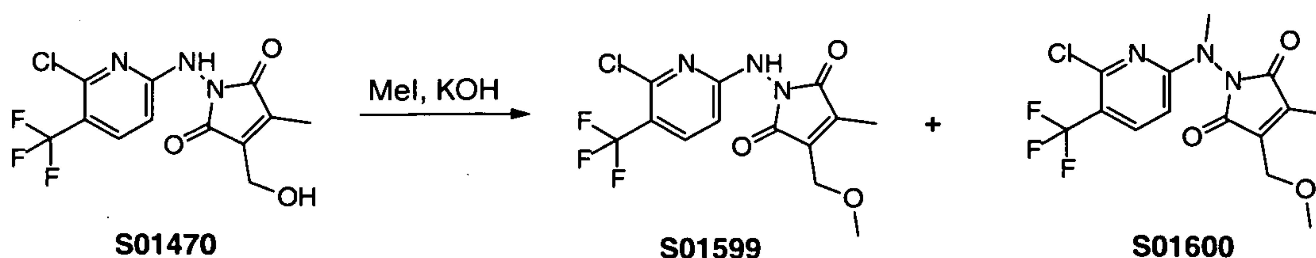
Scheme 12
