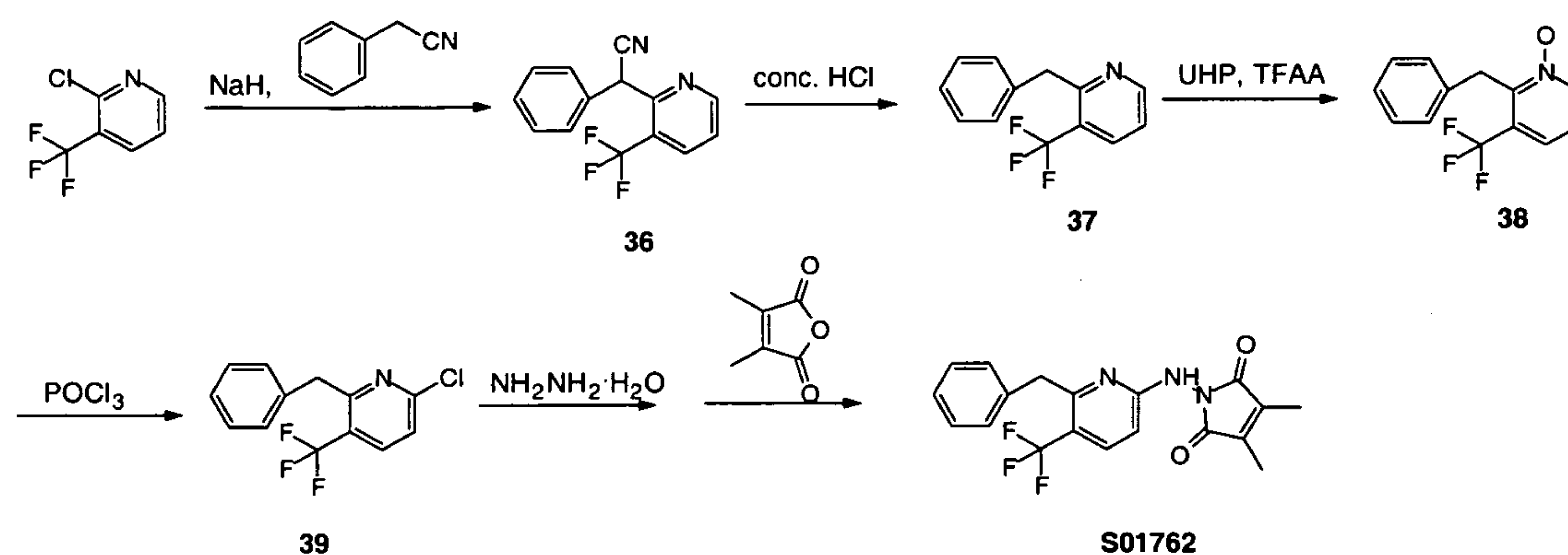
Scheme 20
