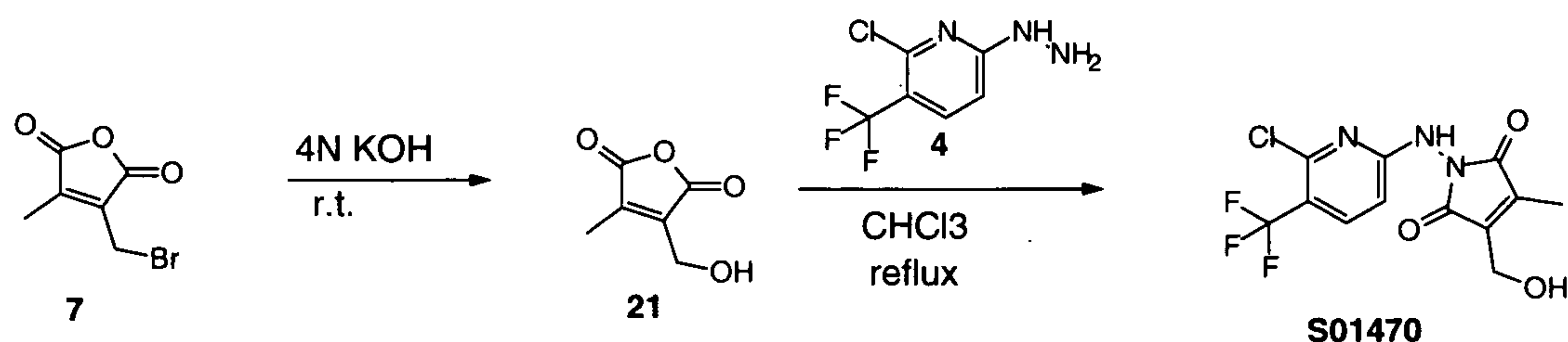
Scheme 11
