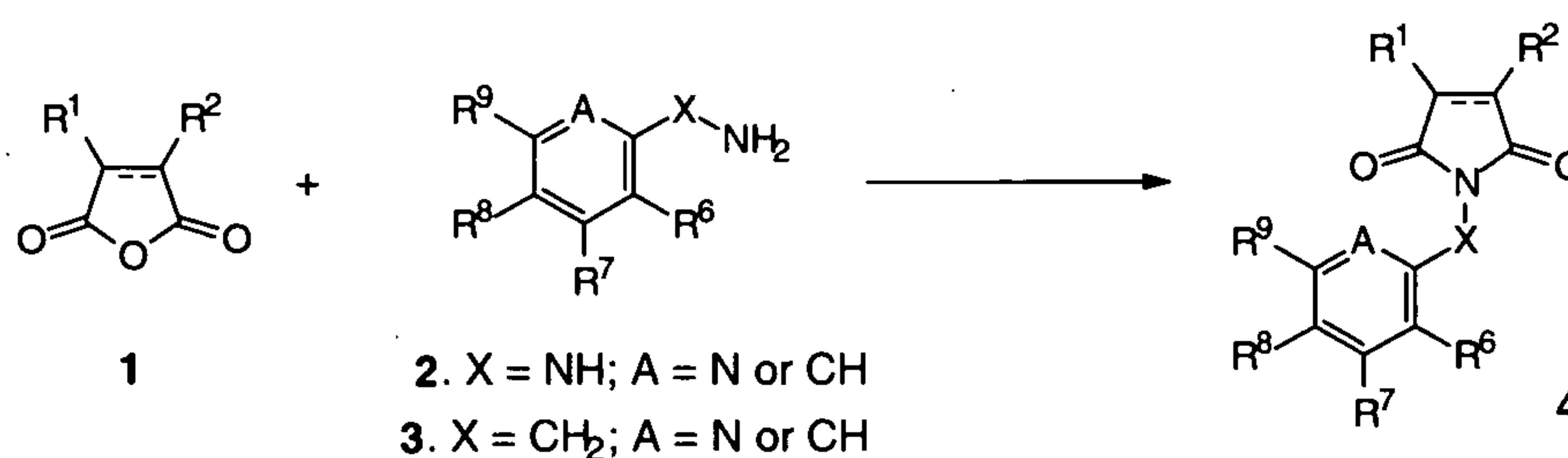
Scheme 1
