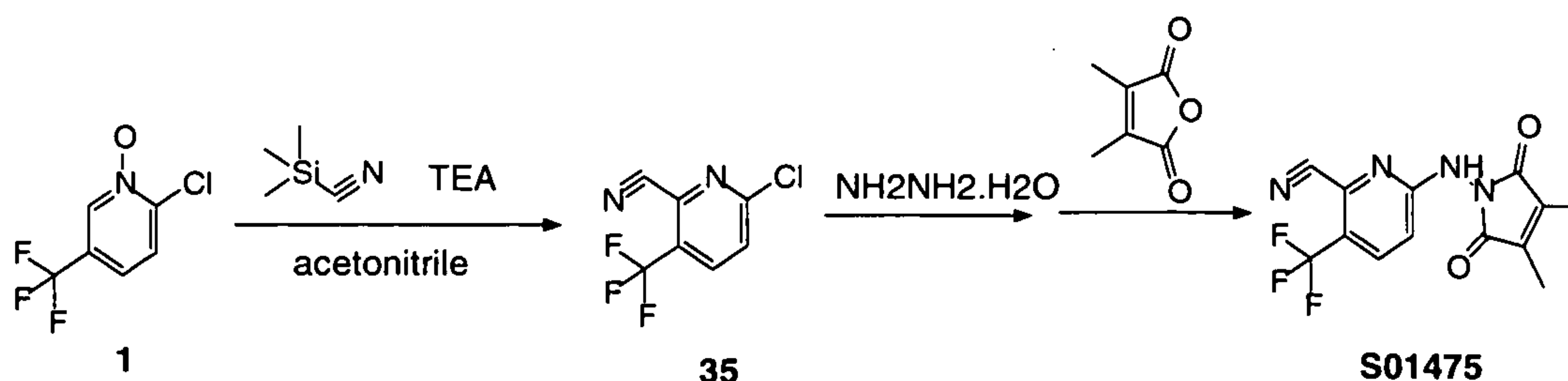
Scheme 19
