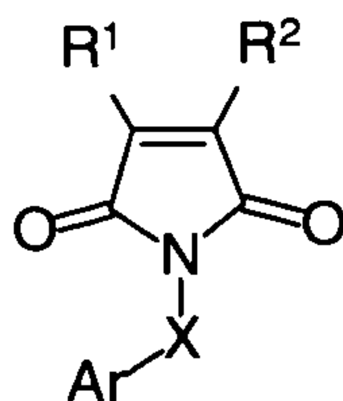
(I)
