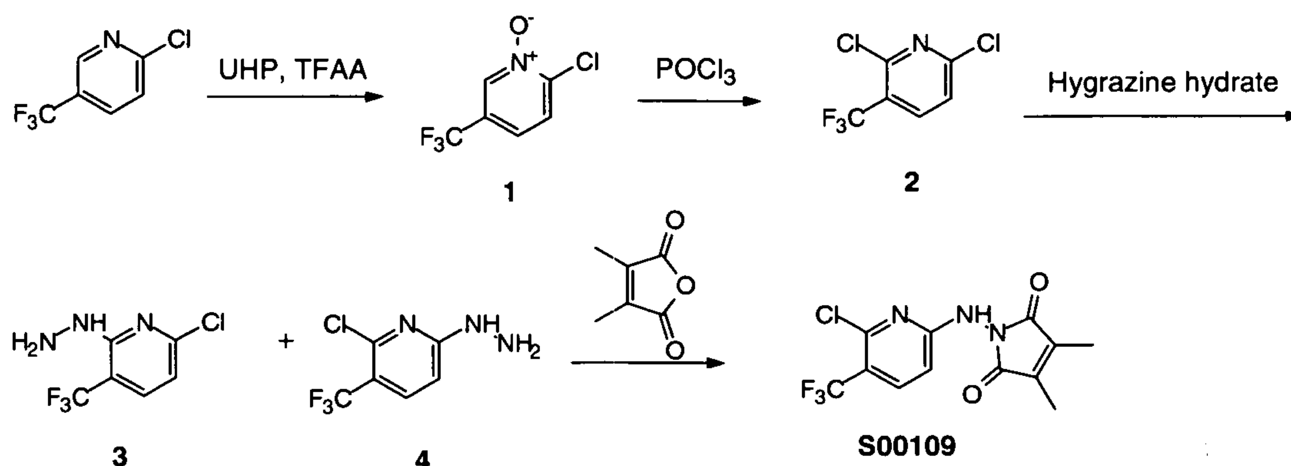
Scheme 2
