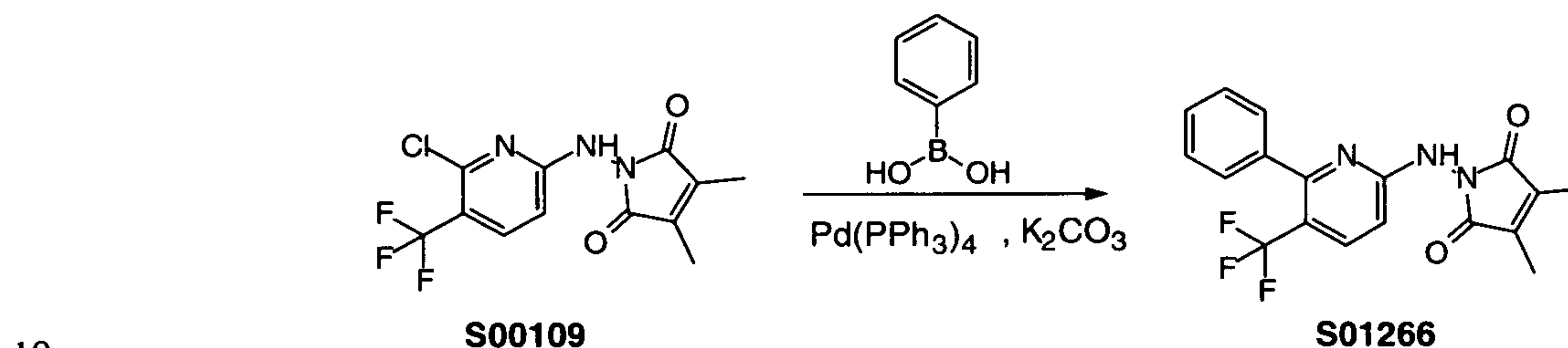
Scheme 14
