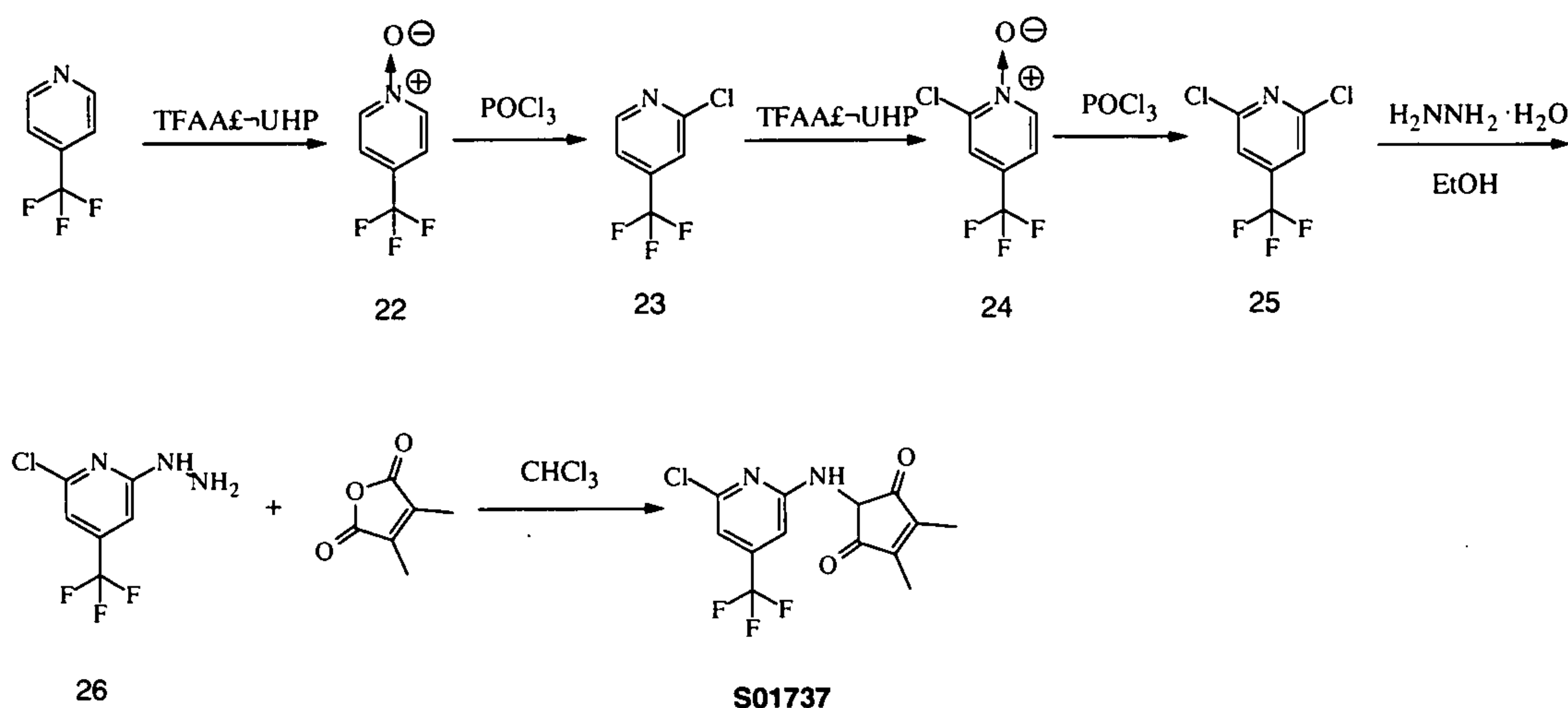
Scheme 15
