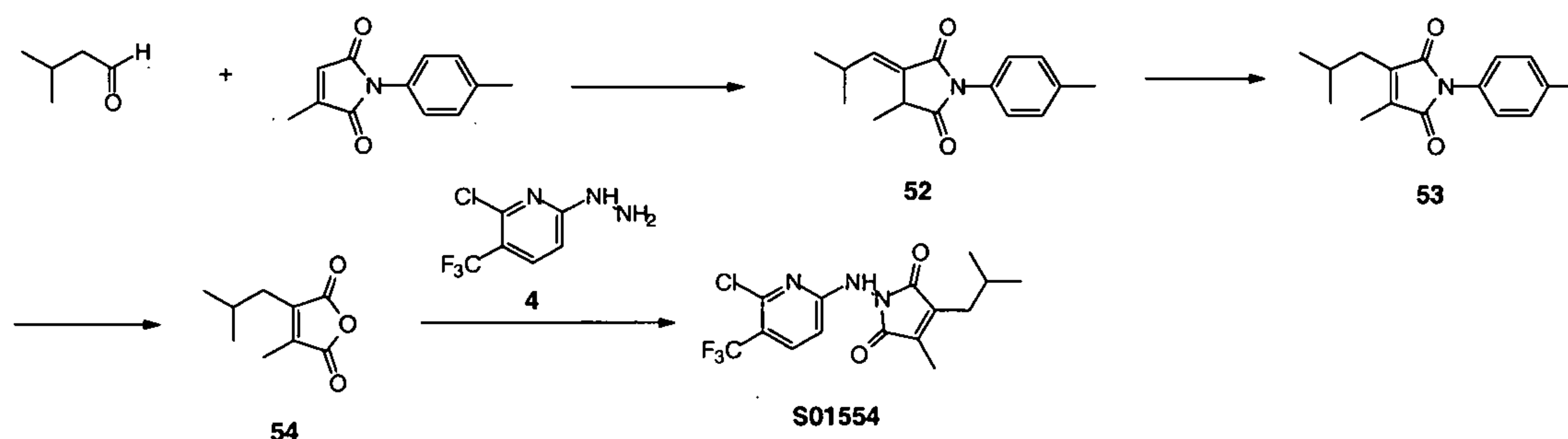
Scheme 26
