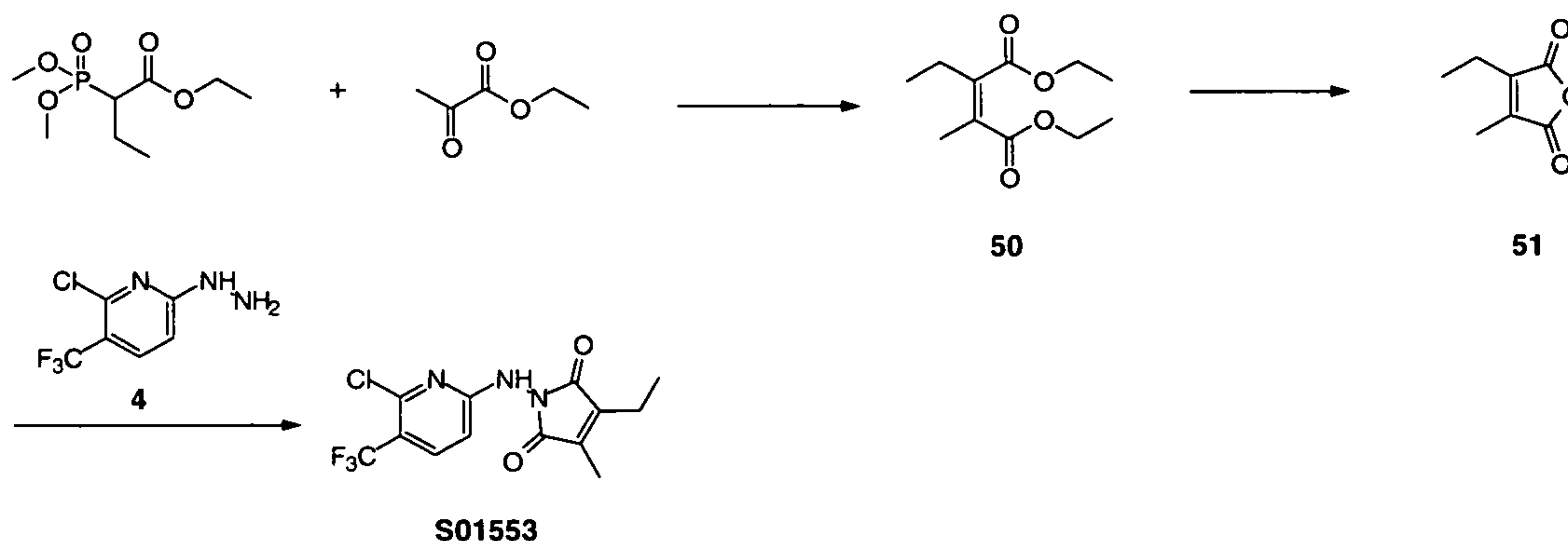
Scheme 25
