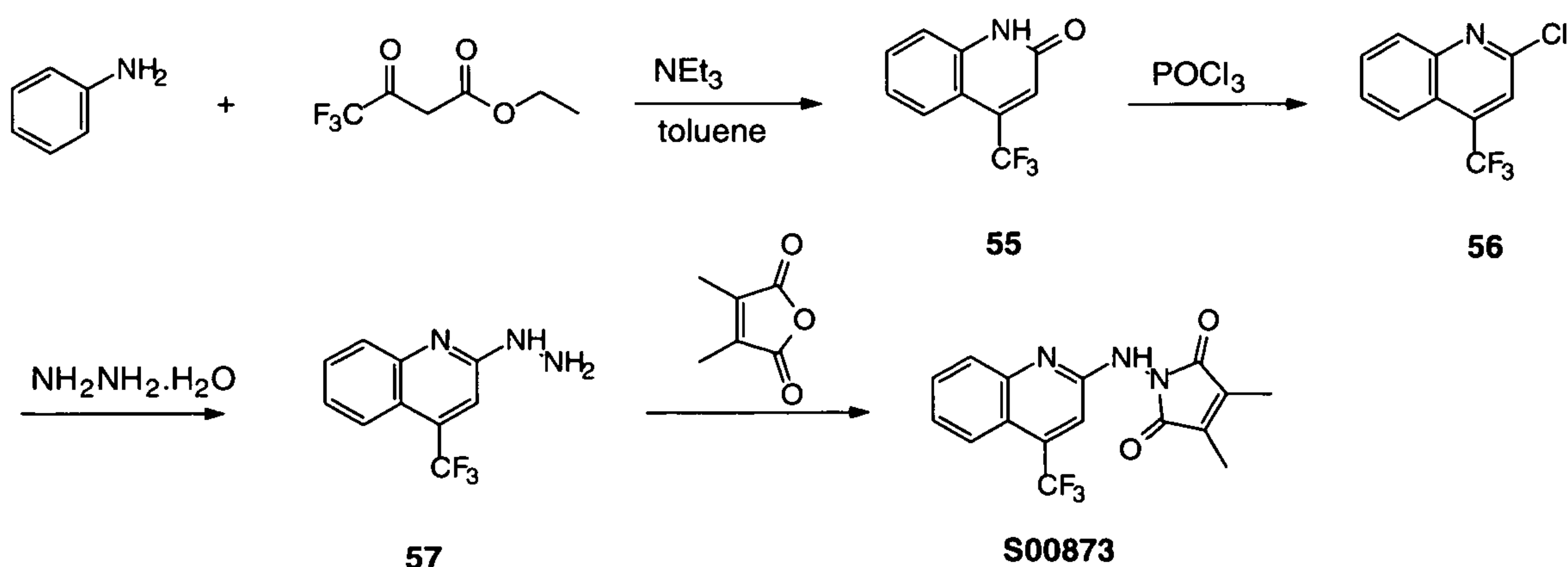
Scheme 27
