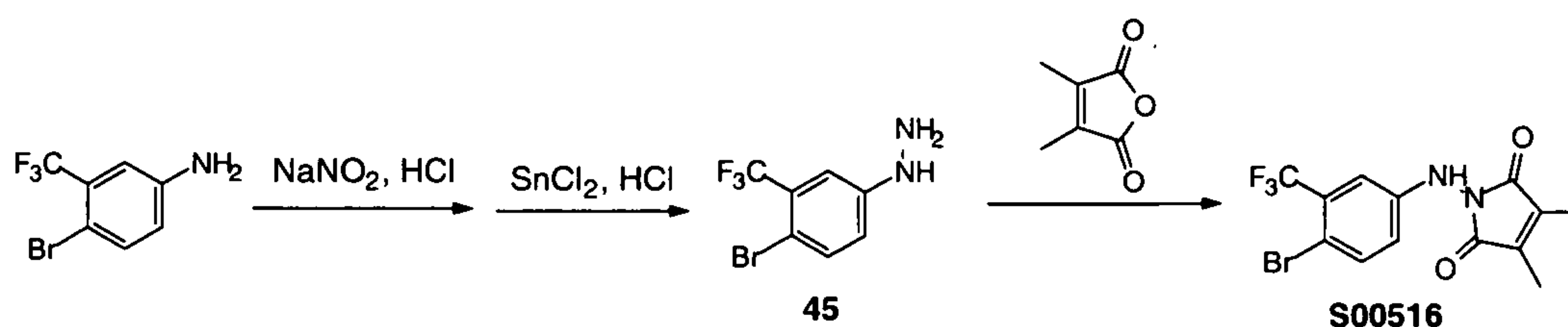
Scheme 23
