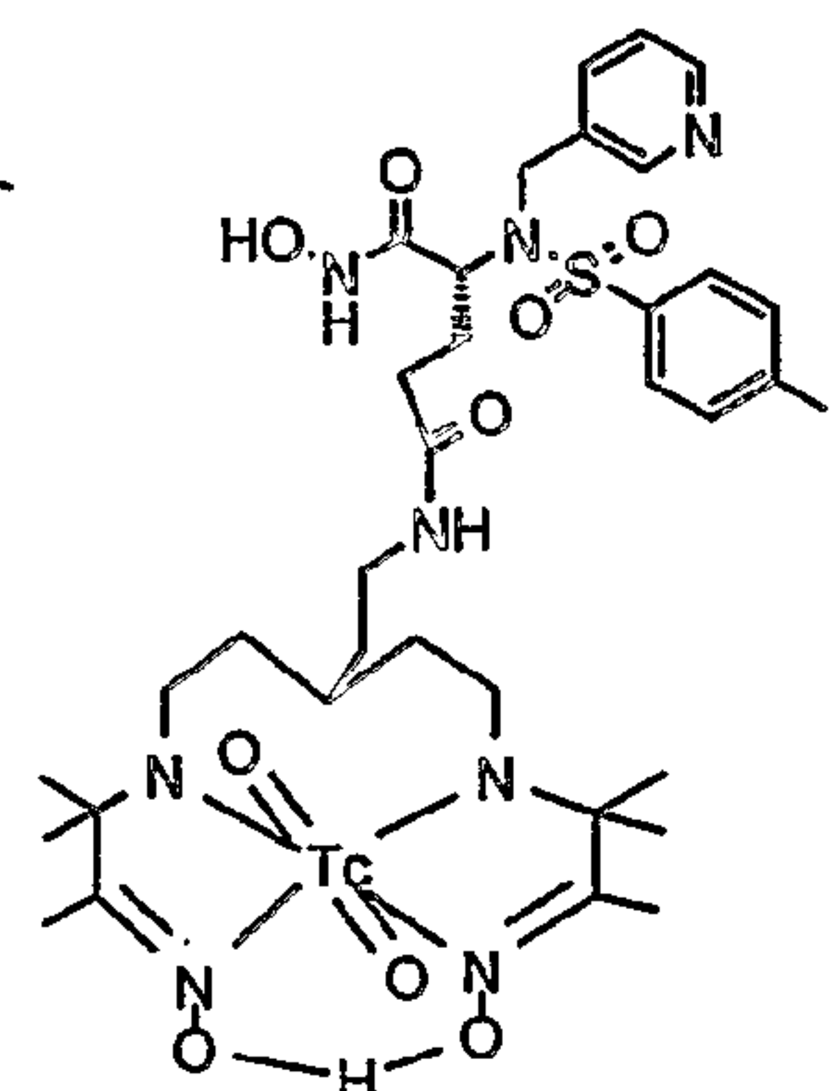
Compound 3
