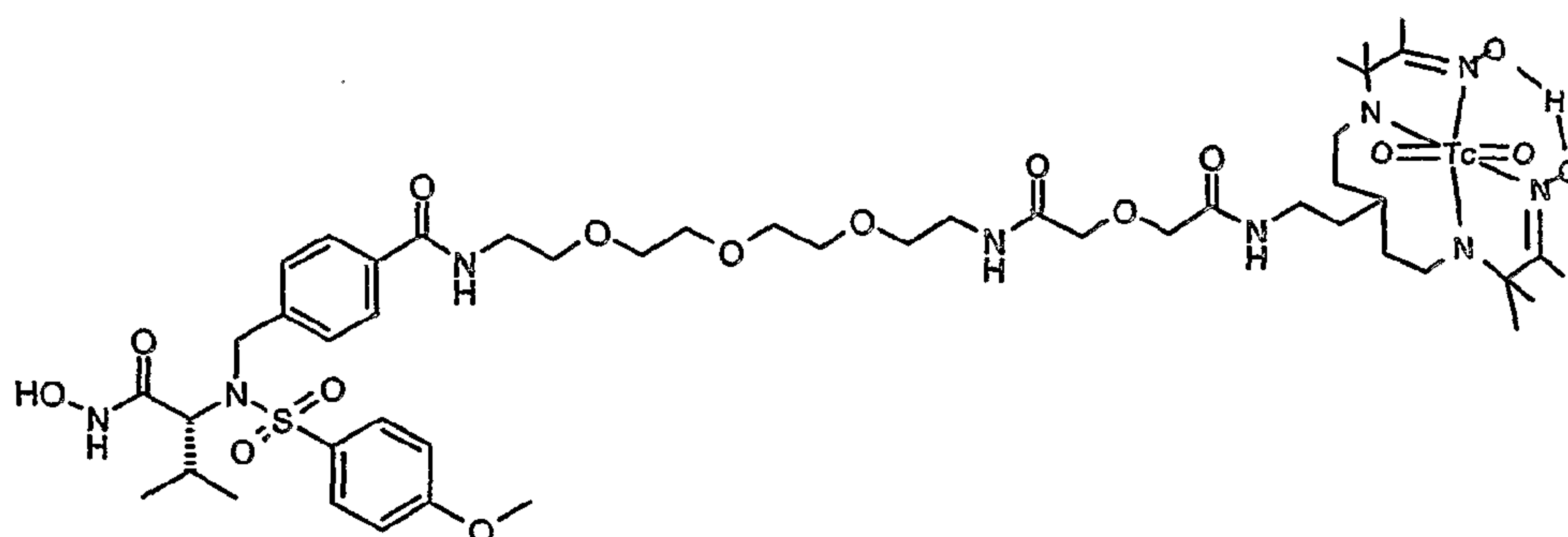
Compound 16
