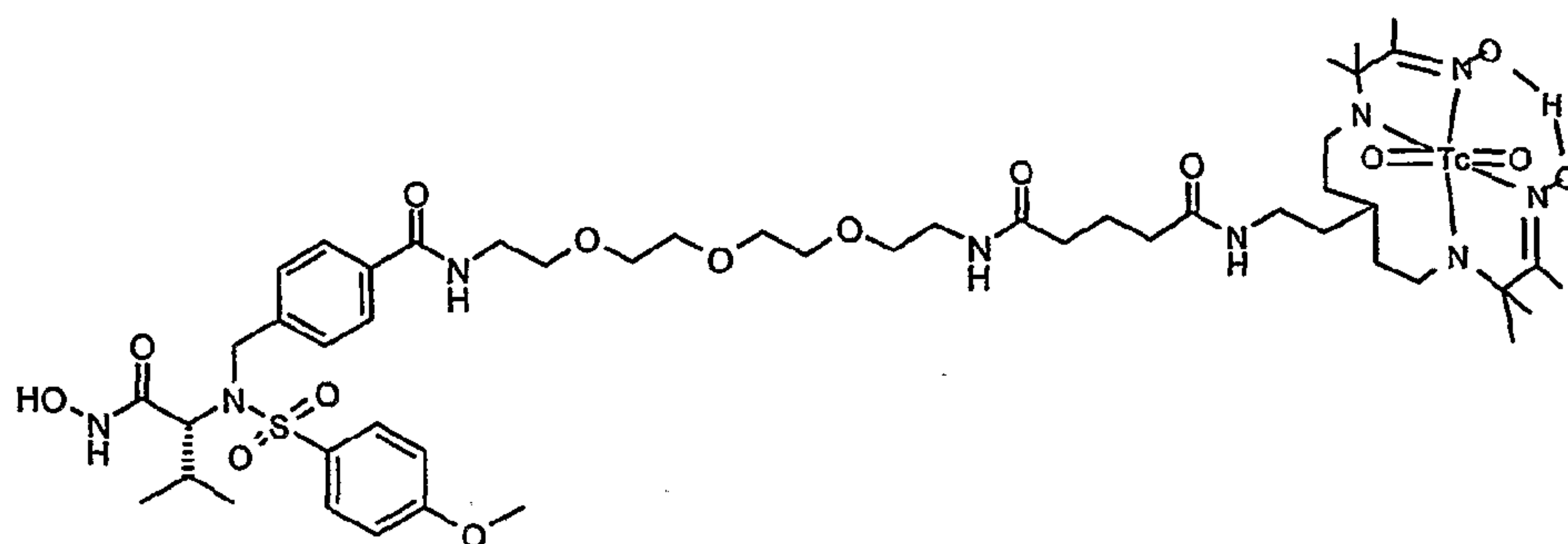
Compound 16
