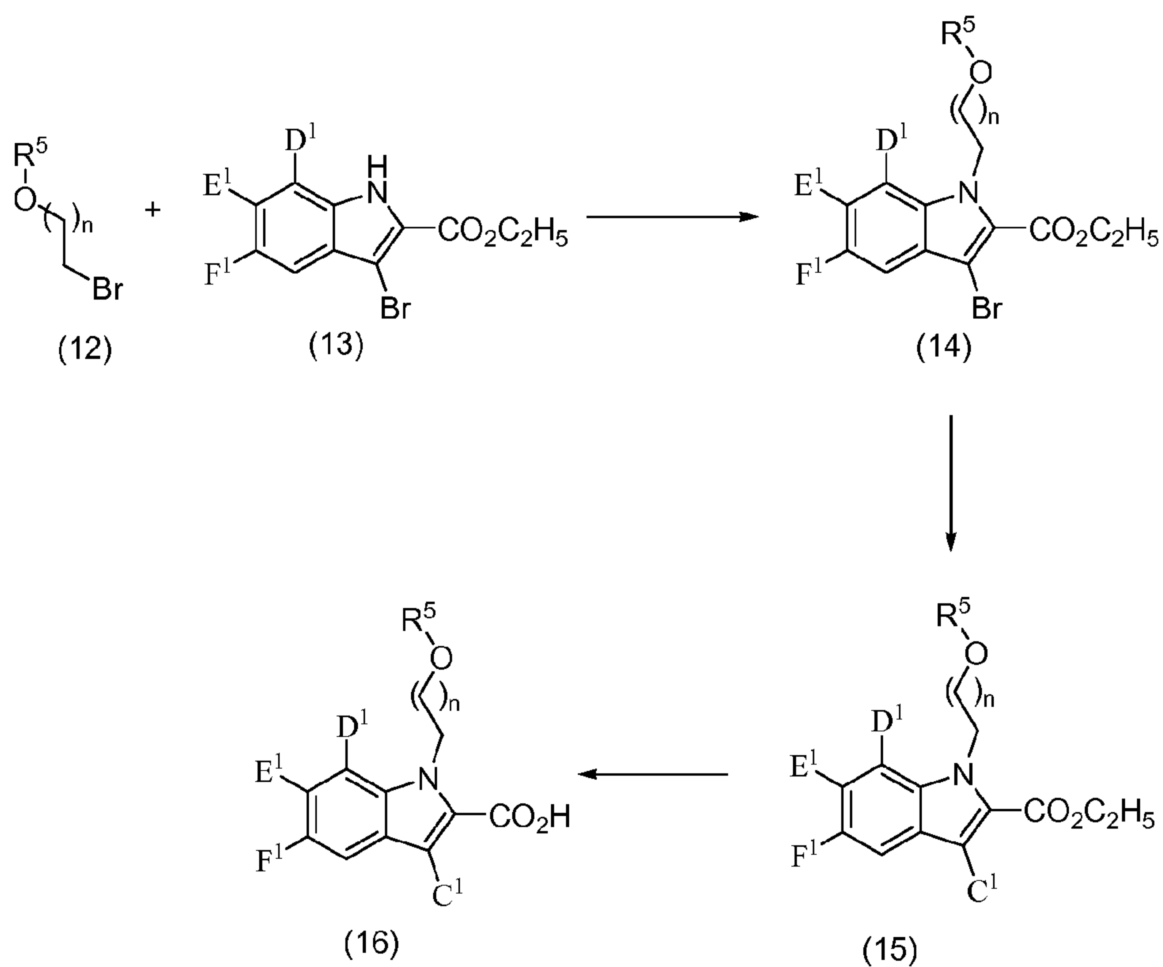
SCHEME 5
