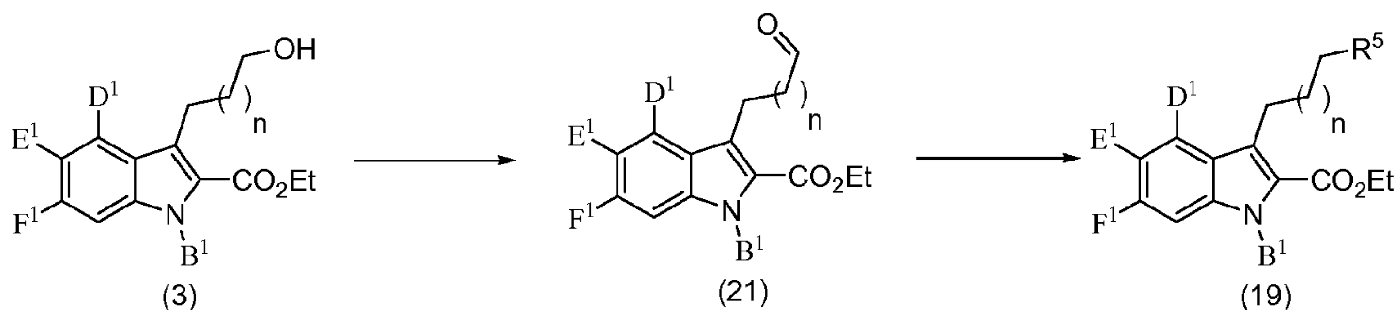
SCHEME 7
