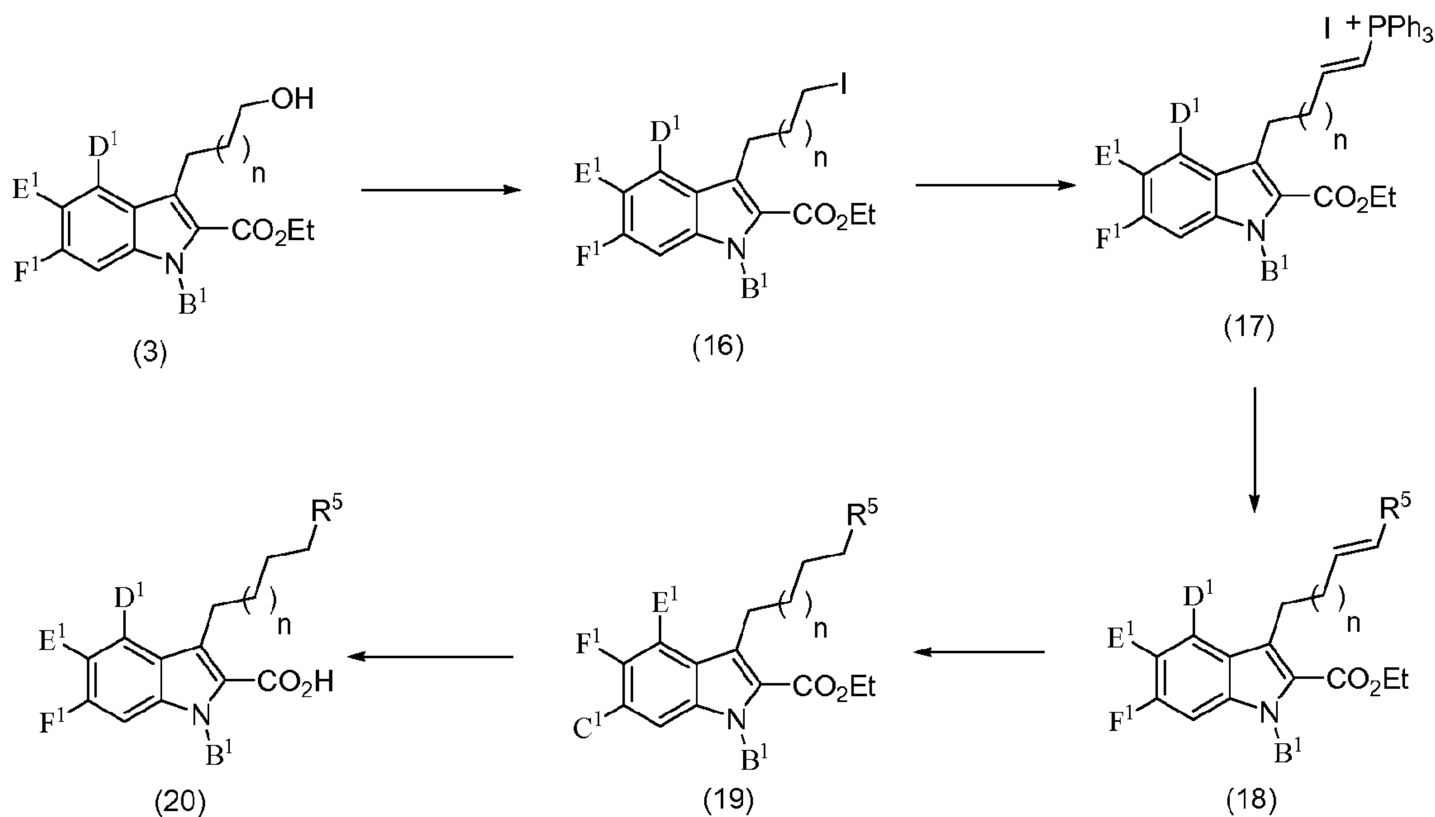
SCHEME 6
