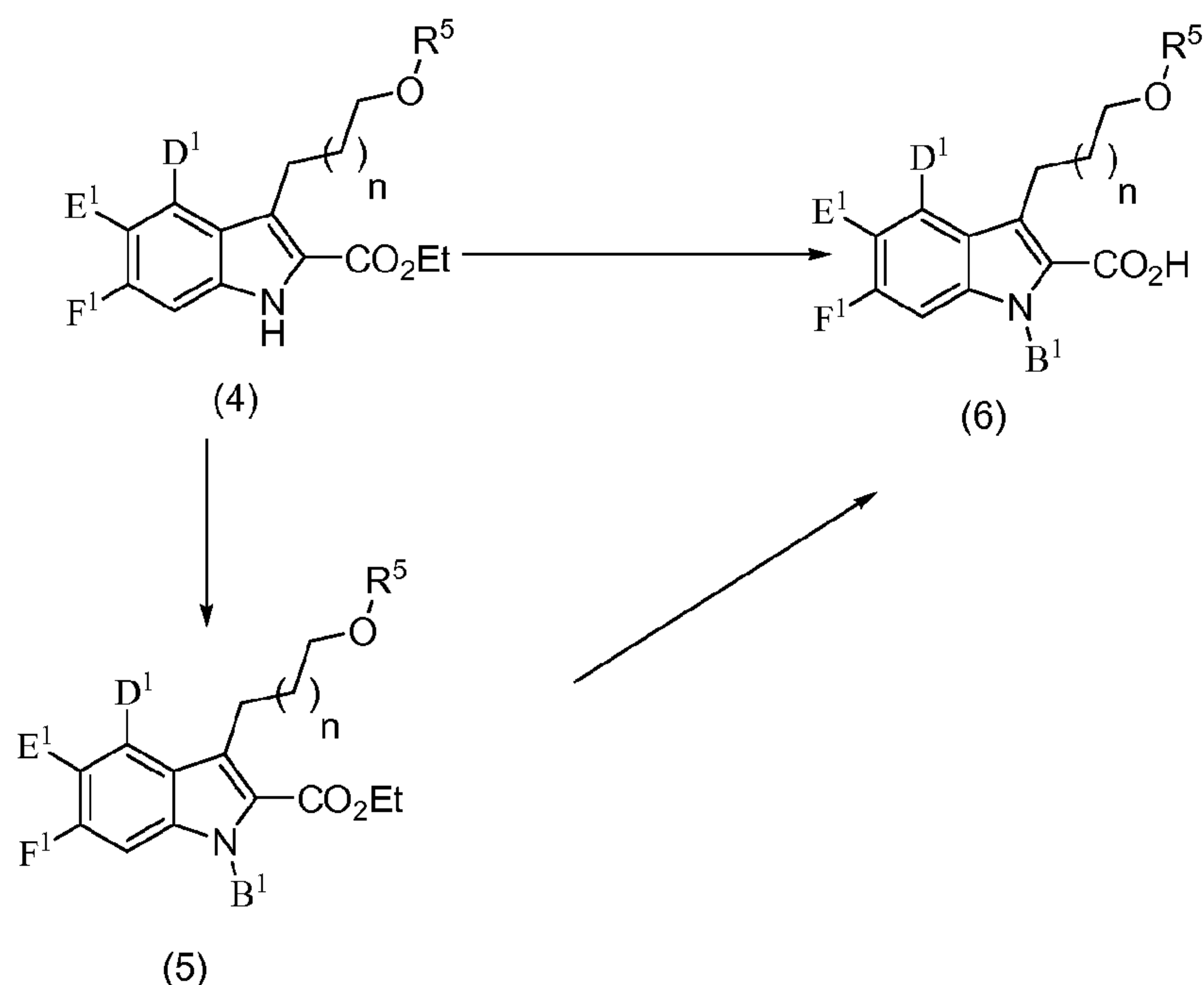
SCHEME 2
