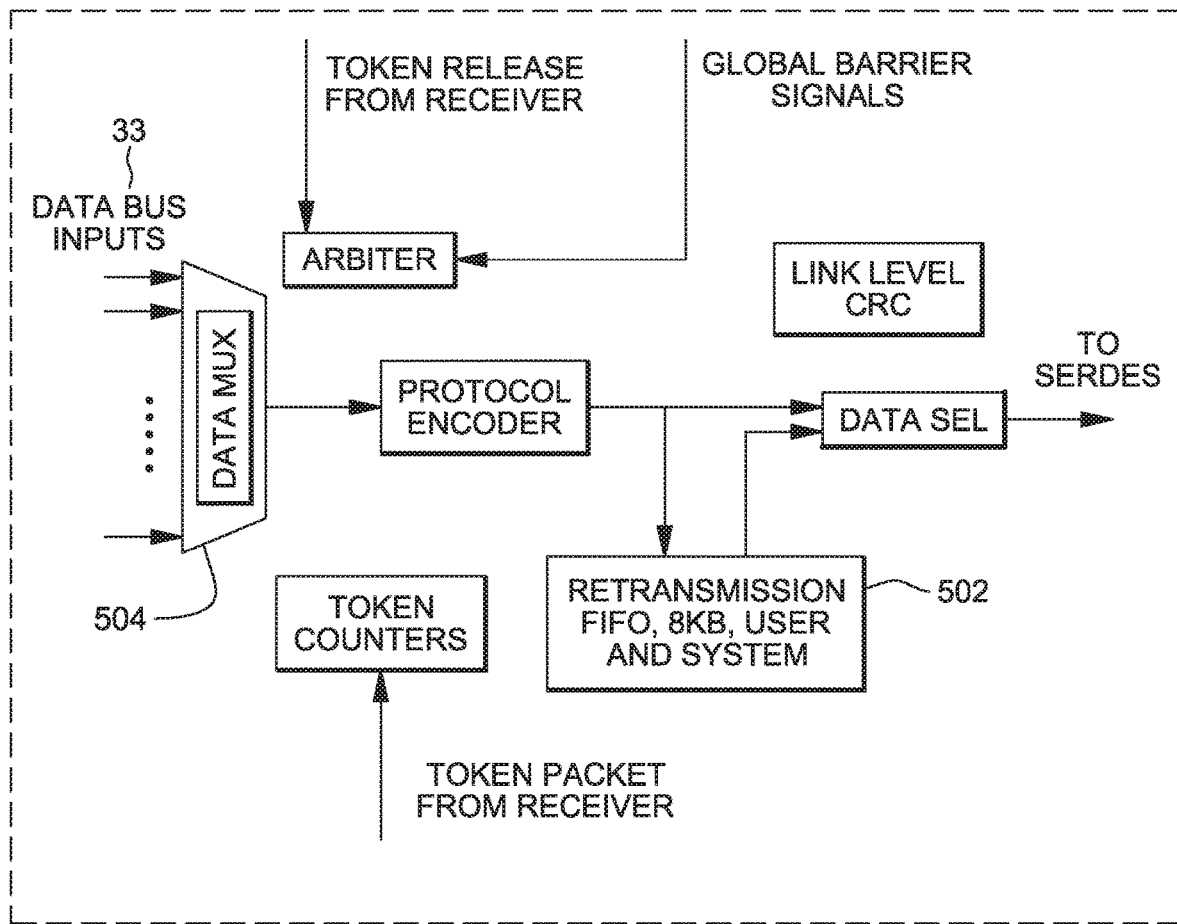
NETWORK SENDER LOGIC BLOCK DIAGRAM
