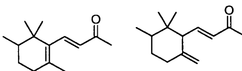
\beta -irone or \gamma -irone
