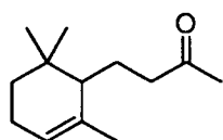
dihydro \alpha -ionone
