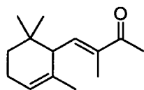
isomethyl \alpha -ionone (3-methyl- \alpha -ionone)
