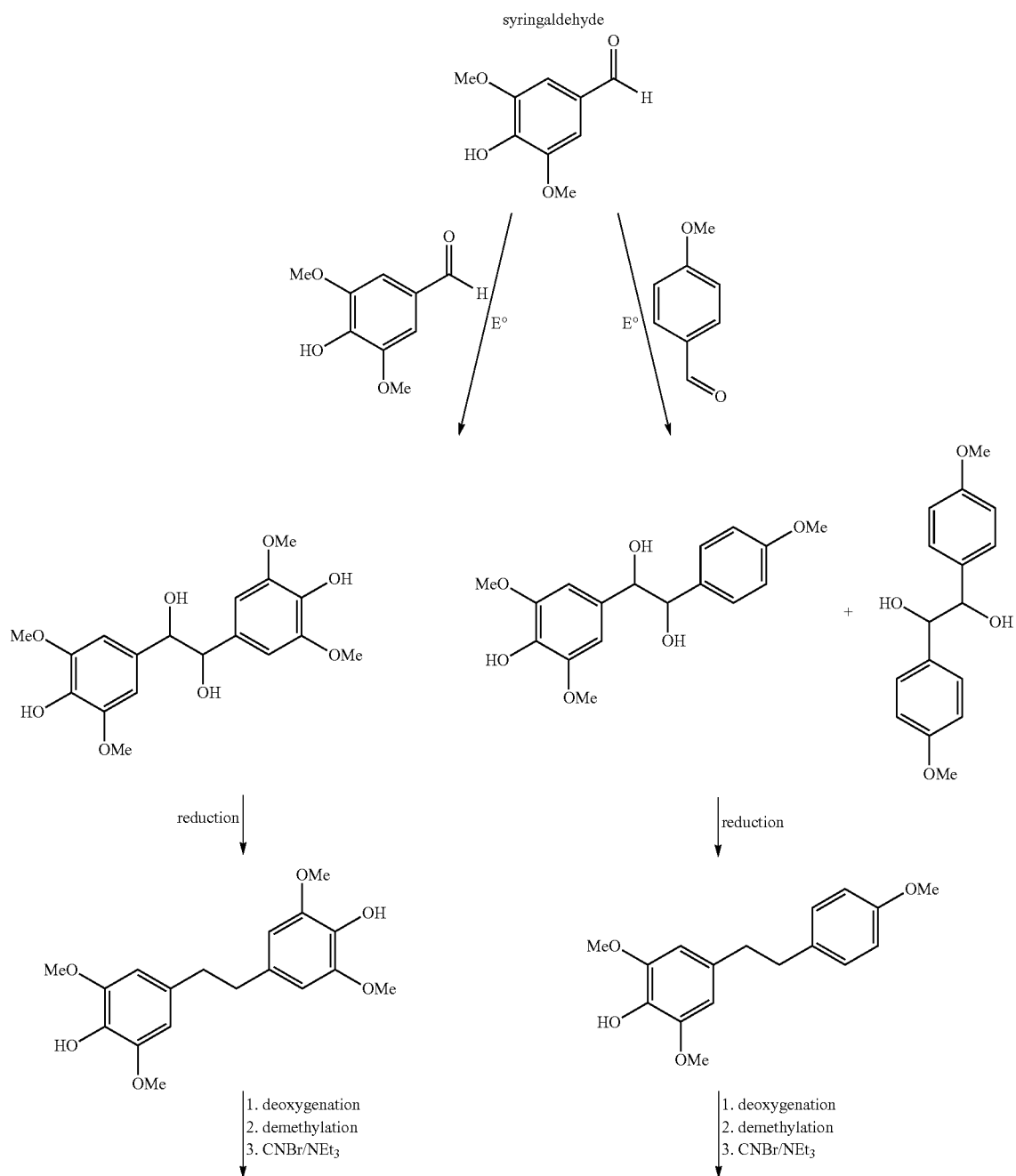
Scheme 4. Conversion of syringaldehyde to cyanate esters without initial dehydrodeoxygenation (electrochemical coupling)
