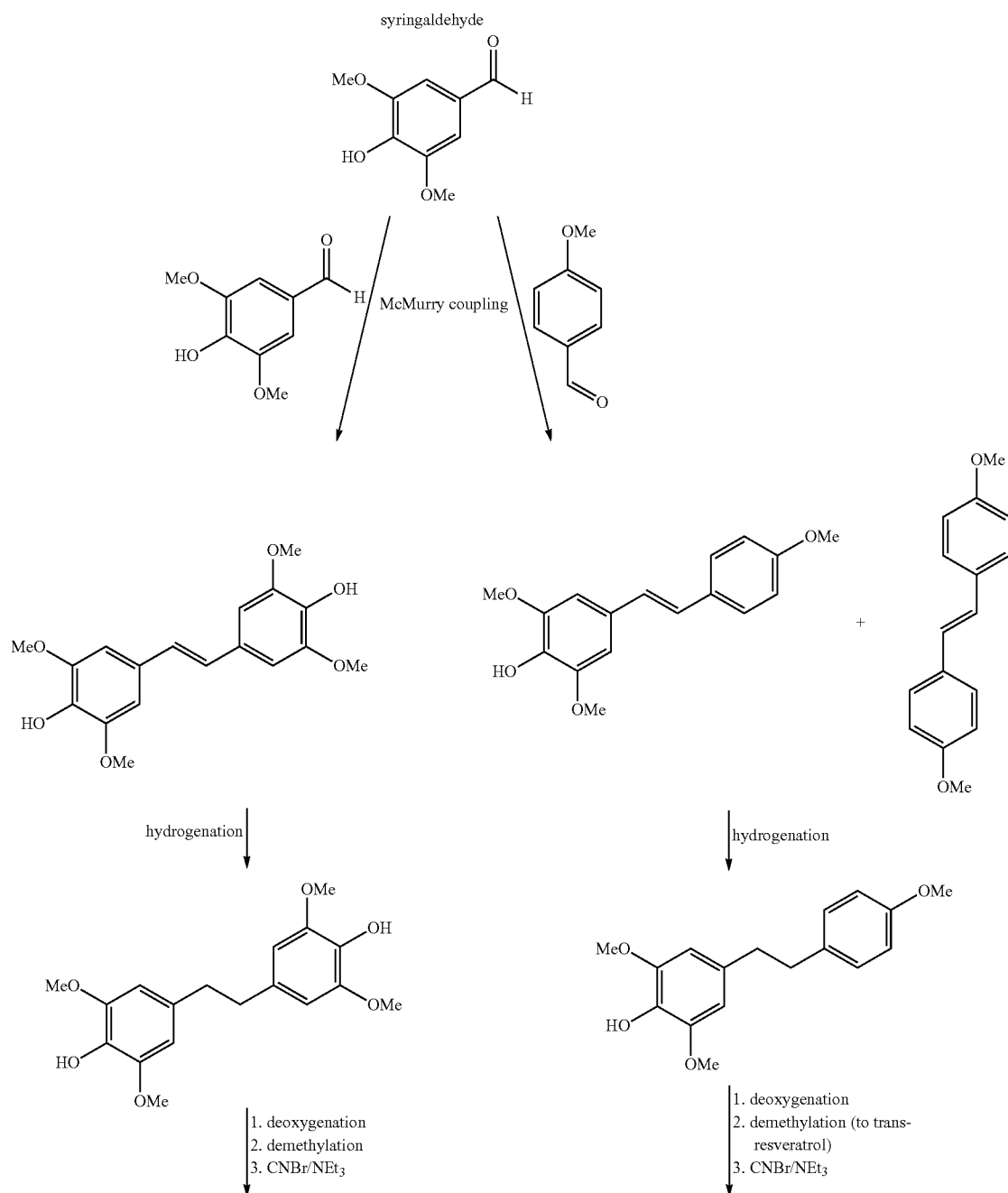
Scheme 3. Conversion of syringaldehyde to cyanate esters without initial dehydrodeoxygenation (McMurry coupling)
