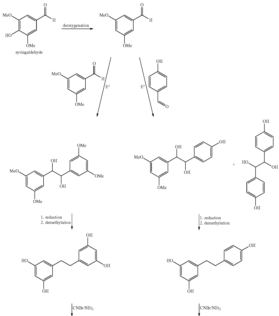
Scheme 2. Conversion of syringaldehyde to cyanate esters with initial dehydrodeoxygenation followed by reduction electrochemical coupling
