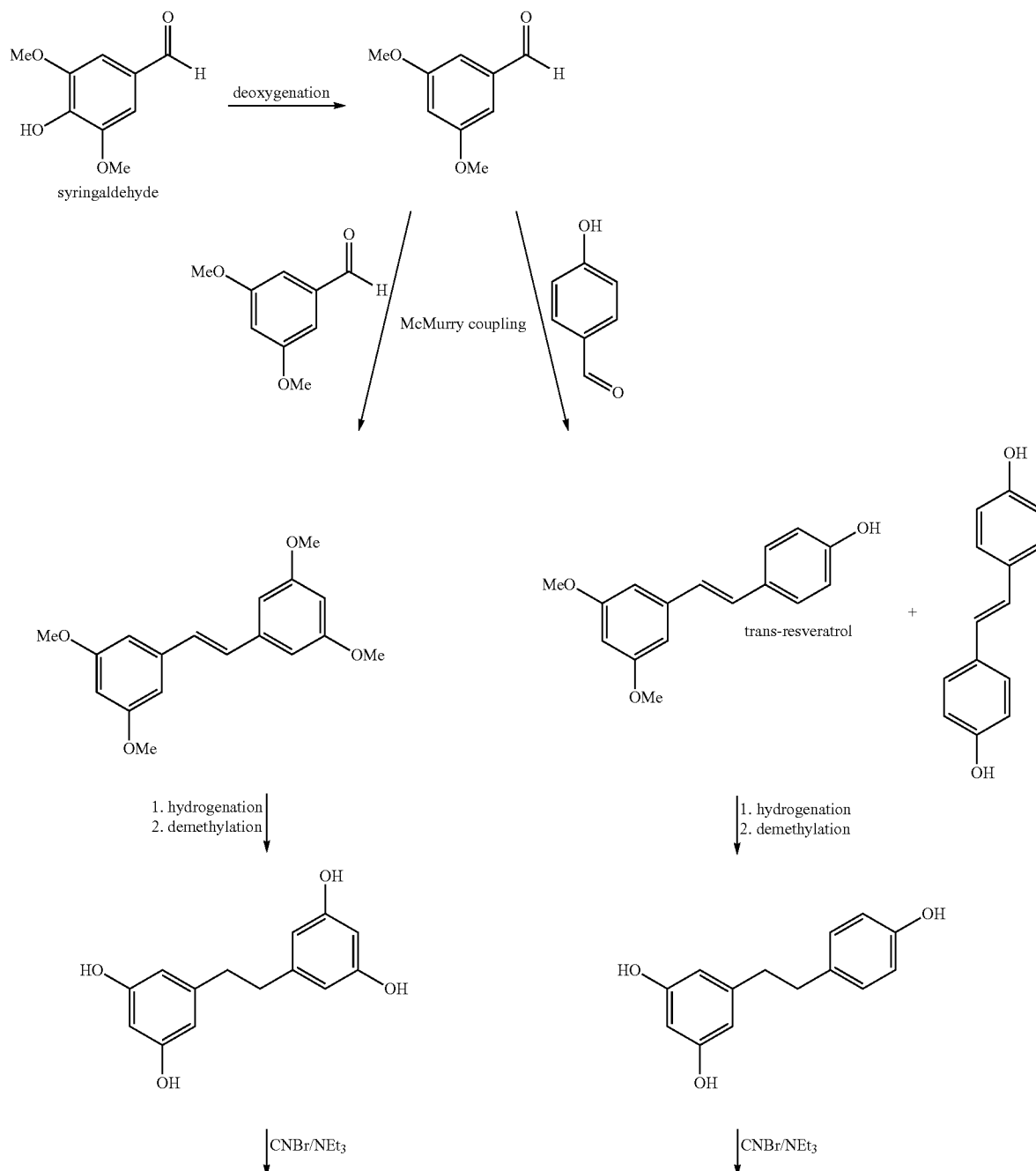
Scheme 1. Conversion of syringaldehyde to cyanate esters by initial dehydrodeoxygenation followed by a McMurry coupling.
