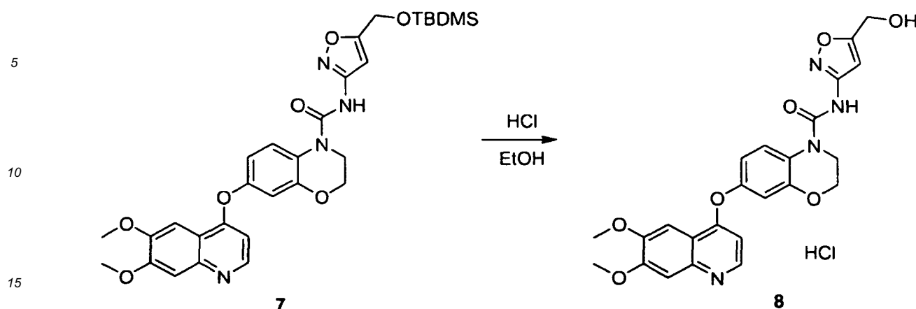
7-(6,7-dimethoxyquinolin-4-yloxy)-N-(5-(hydroxymethyl)isoxazol-3-yl)-2,3-dihydrobenzo[b][1,4]oxazine-4-carboxamide hydrochloride (8).
