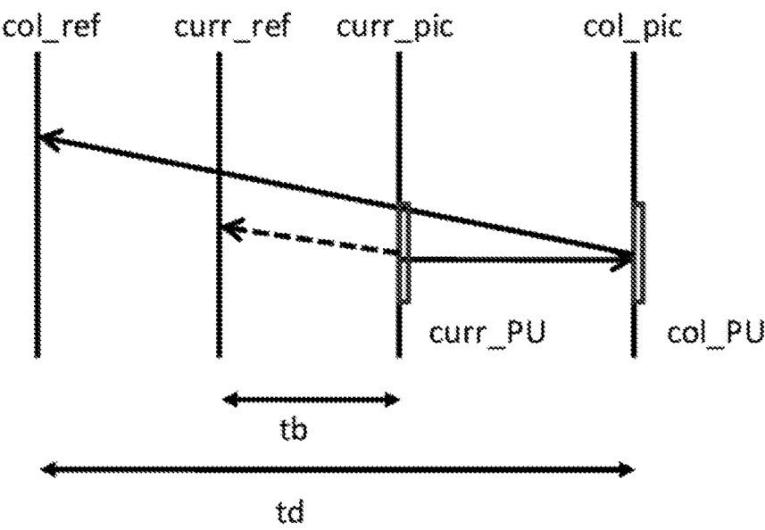
Illustration of motion vector scaling for temporal merge candidate
