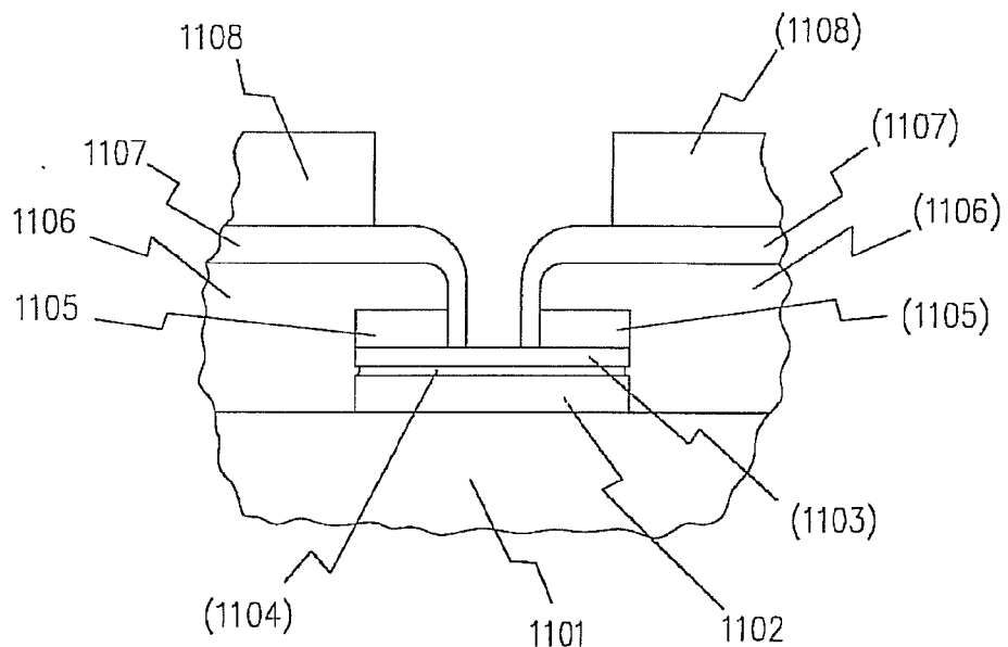
FIGURE 11a ELECTRODES
