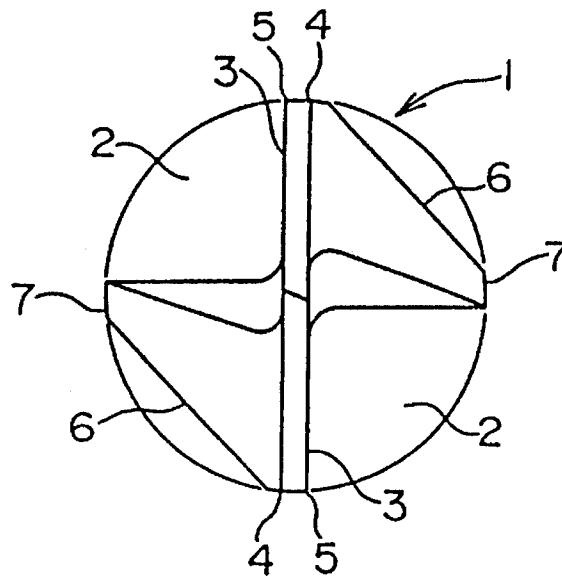
FIG. 7 PRIOR ART
