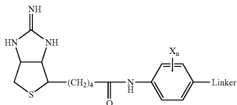
Examples of Affinity-Coupled Mass Defect Labels
