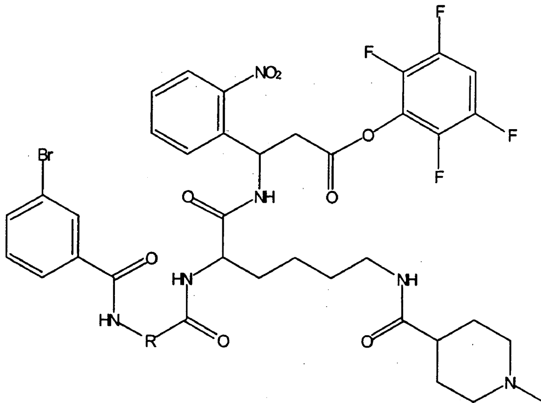
The general structure of the photocleavable mass defect tag where Br is the mass defect element that is linked through the amino acid (R) to the remainder of the tag.
