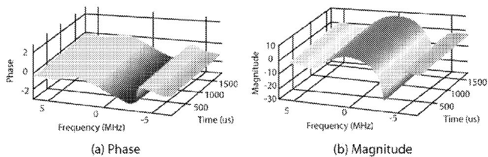
Figure 2 Indoor wireless channel (ETSI BRAN)
