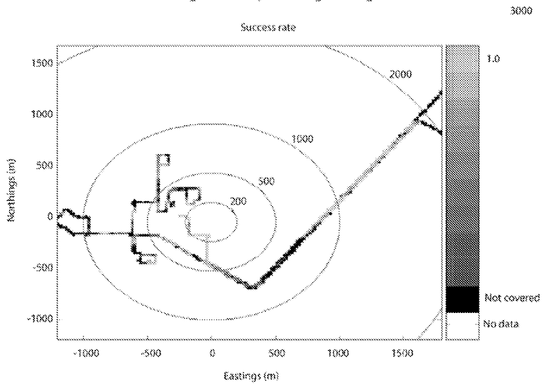
Figure 17 Best grade 6 Mbps 802.11g coverage
