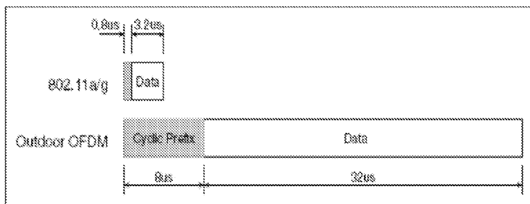
Figure 9 OFDM symbol dimensions
