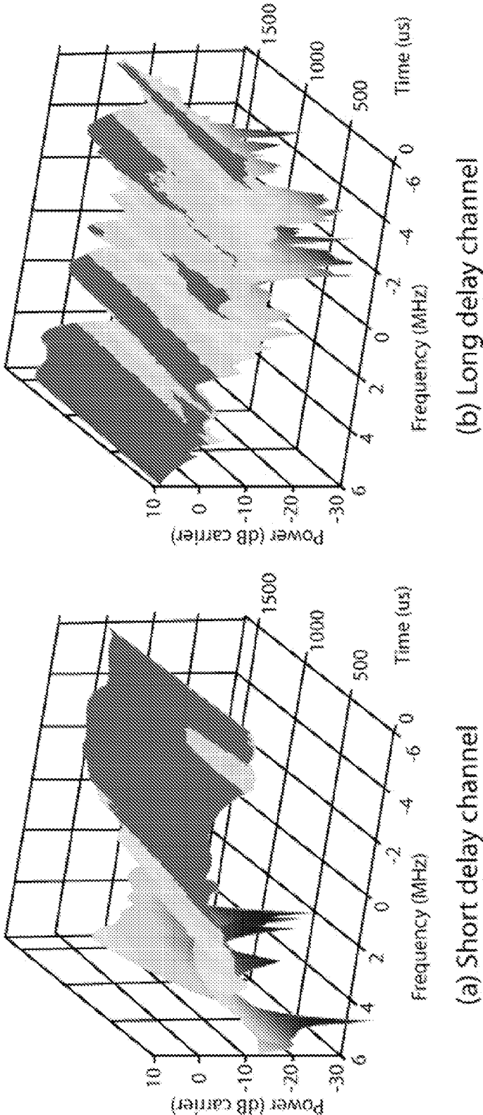
Figure 7 Mobile channel captures at 60mph
