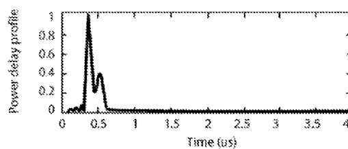
(c) Power delay profile
