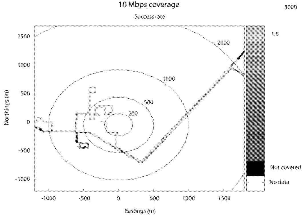
Figure 16 10 Mbps coverage
