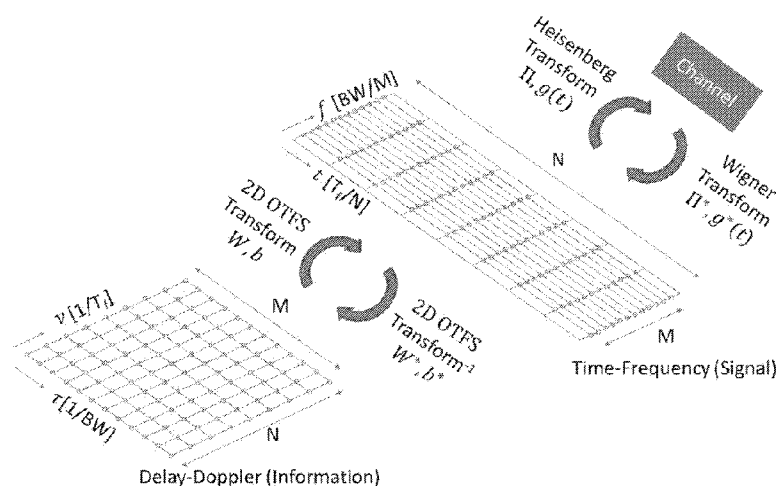
Transformation of the Time-Frequency Plane to the Doppler-Delay Plane
