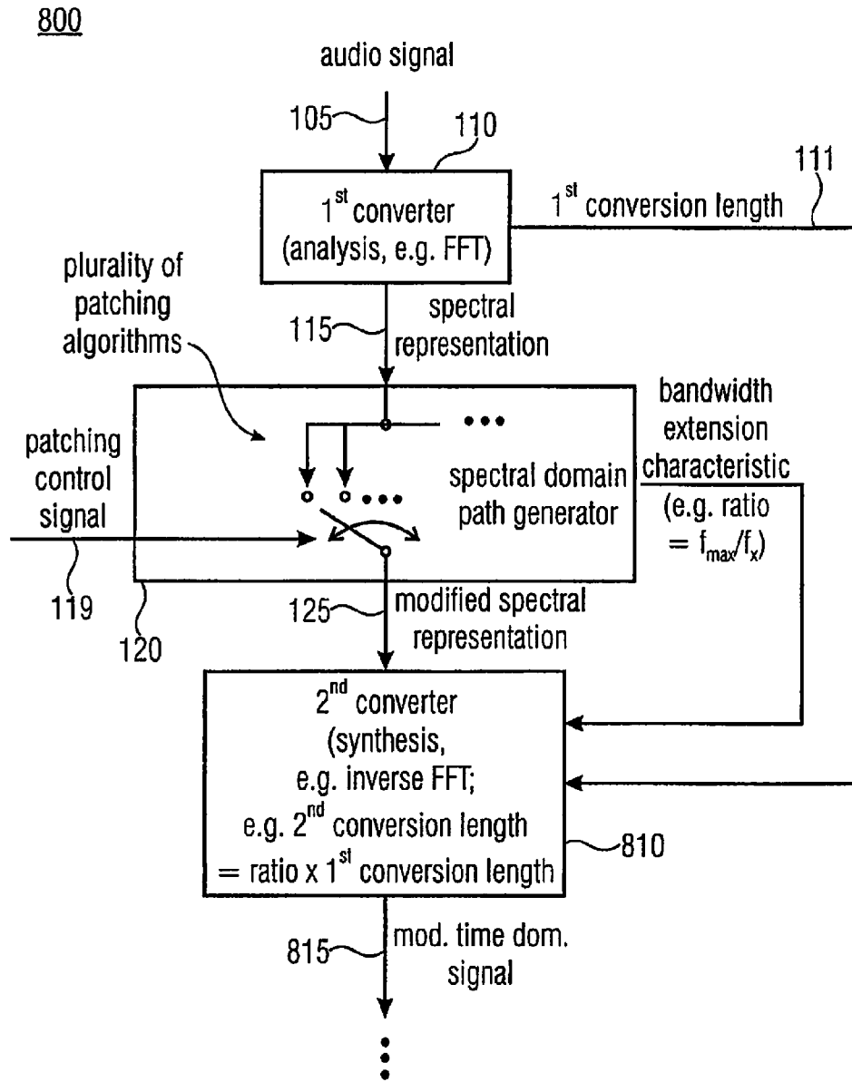
FIGURE 8 (AUDIO SIGNAL SYNTHESIZER)
