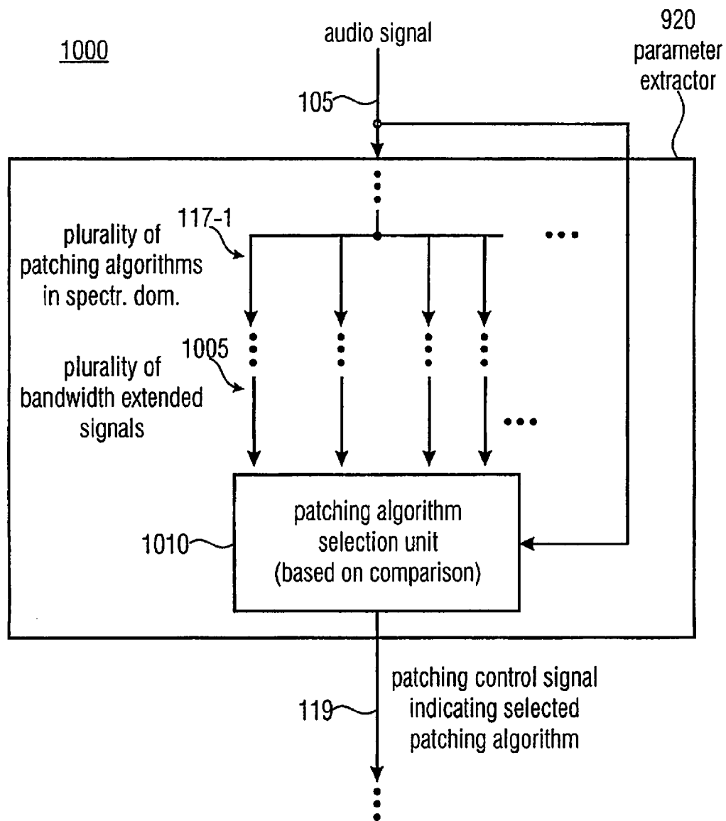
FIGURE 10 (ENCODER)
