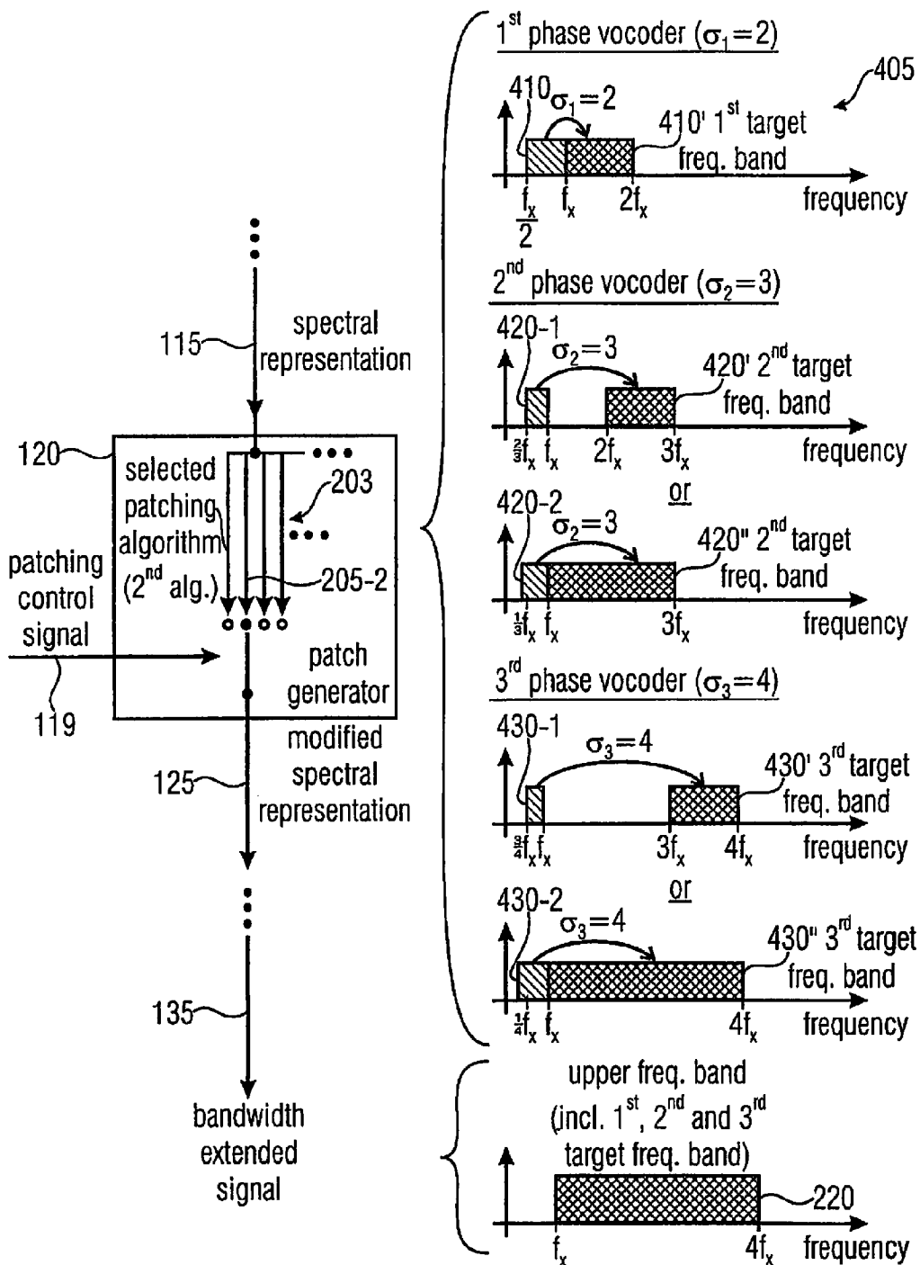
FIGURE 4 (SECOND PATCHING ALGORITHM)
