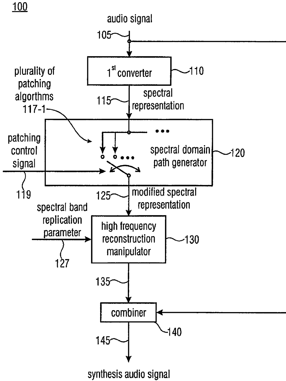
FIGURE 1A (AUDIO SIGNAL SYNTHESIZER)
