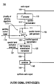
(AUDIO SIGNAL SYNTHESIZER)
