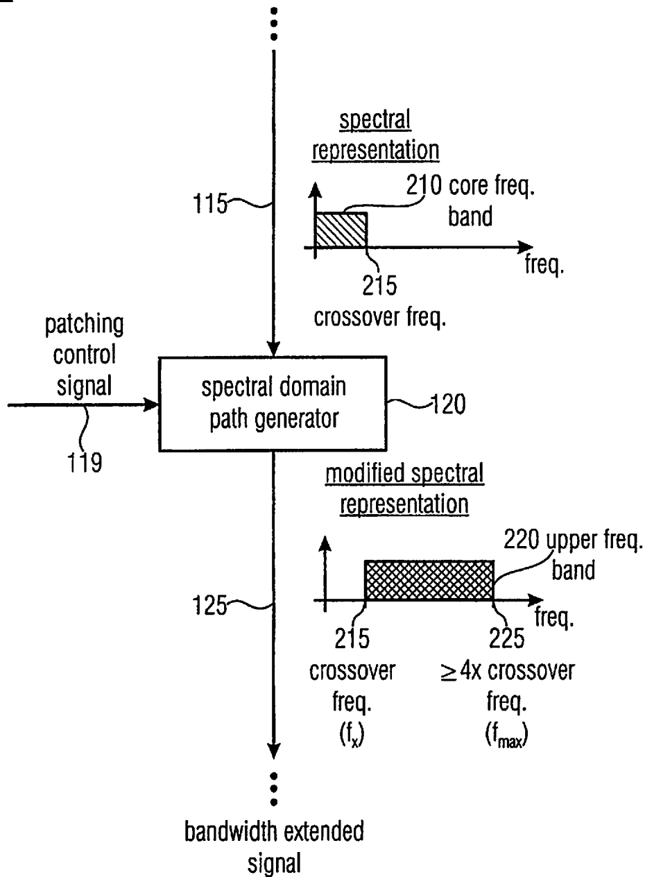
FIGURE 2B (BANDWIDTH EXTENSION SCHEME)
