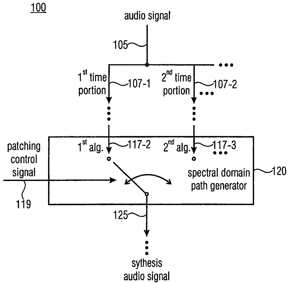
FIGURE 1B (SPECTRAL DOMAIN PATCH GENERATOR)
