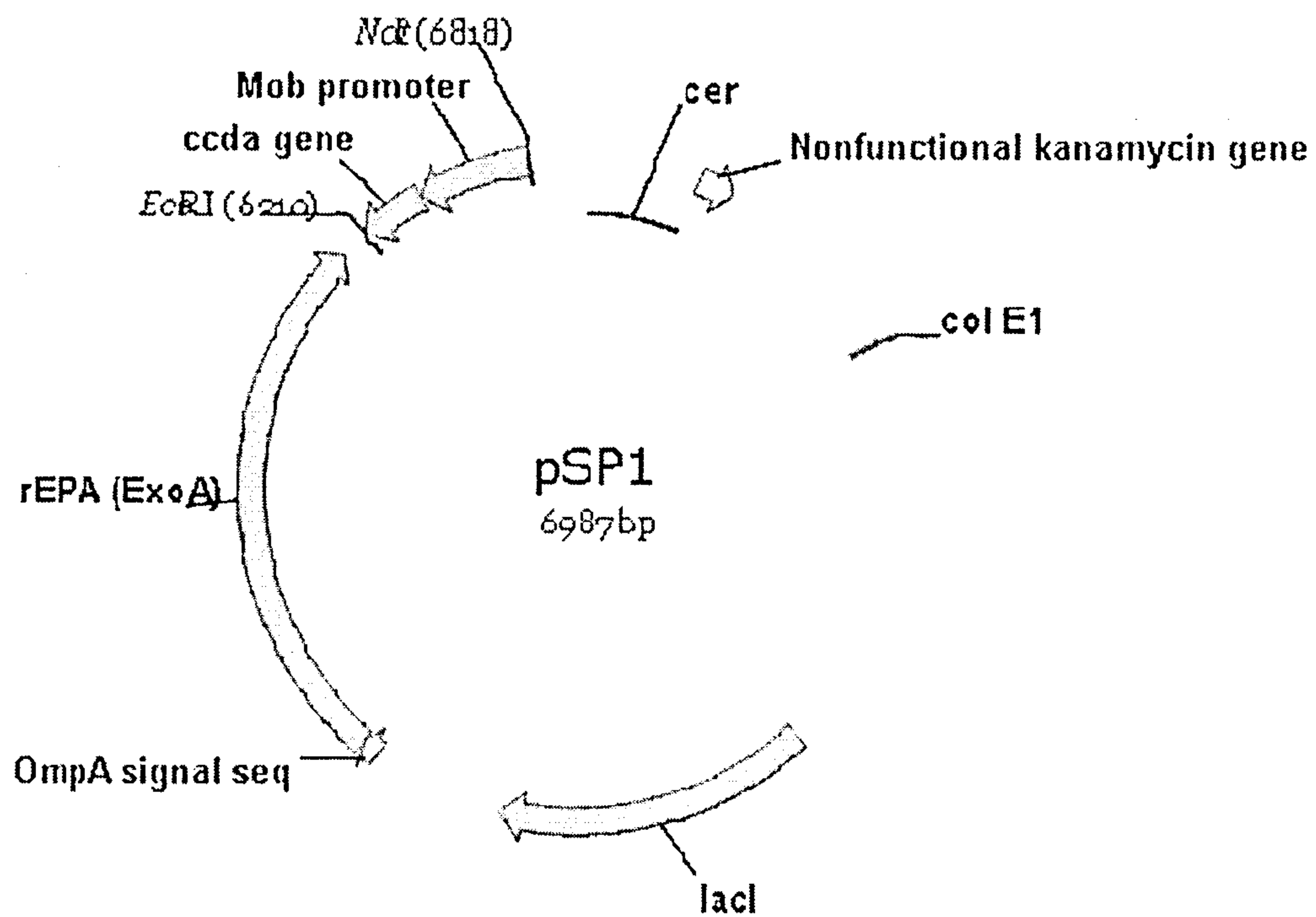
Figure 1: Schematic representation of the plasmid pSP1
