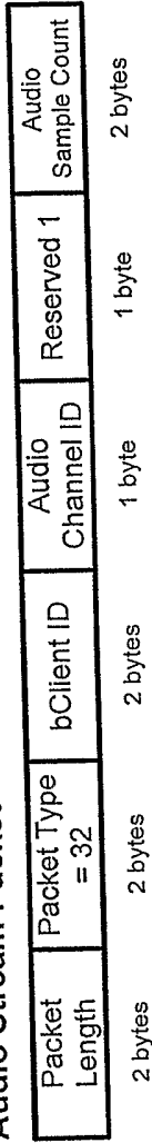
Audio Stream Packet
