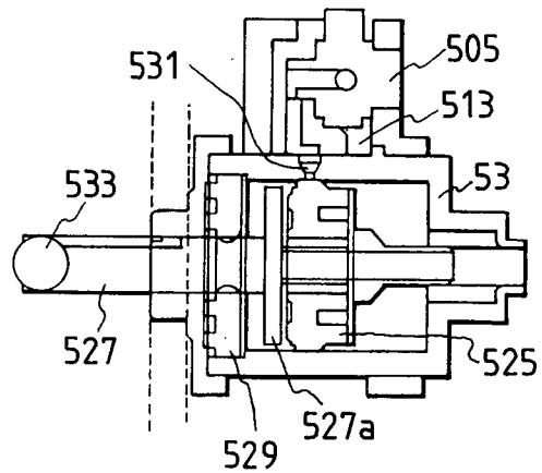
④ POSITION FOR PREPARING IDLE SUCTION
