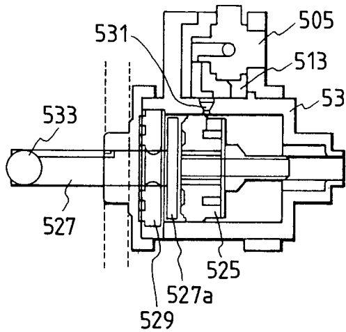
② UPPER DEAD CENTER
